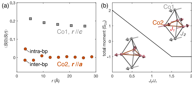
FIG. 3. (a) Spin correlations \langle S(0) \cdot S(r) \rangle as a function of distance r calculated through RMC. Gray squares (red circles) are the correlations for the Co1 (Co2) spins along the c ( a ) axis. For the first-neighbor Co2 spins at r \sim 3.2 Å, correlations within the bipyramids (intra-bp) and out of the bipyramids (inter-bp) are calculated separately. Error bars representing the standard deviations are smaller than the size of the symbol. (b) Total moment of the spin bipyramid as a function of J_2/J_1 . Insets are representative ground states for infinitely small J_2/J_1 (left) and J_2/J_1 \geq 1.5 (right).
