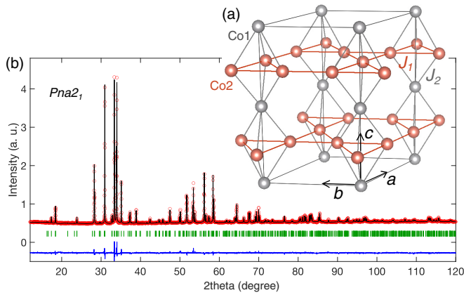
FIG. 1. (a) The Co ions in CYBCO form a lattice of alternating triangular (Co1) and kagome (Co2) layers in the ab plane. The crystal structure is shown in the hexagonal unit cell. J_1 ( J_2 ) denotes the couplings within the kagome layers (between the kagome and triangular layers). (b) Refinement results of the XRD data measured at room temperature for pulverized CYBCO crystals. Data points are shown as red circles. The calculated pattern is shown as the black solid line. The vertical bars show the positions of the Bragg peaks for CYBCO with space group Pna2_1 . The blue line at the bottom shows the difference of measured and calculated intensities.
