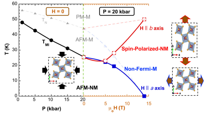
FIG. 5. A phase diagram for T_{MI} (thick lines) and T_N (dashed thin lines) as functions of pressure and magnetic field for H||a axis (blue lines) and H||b axis (red lines) at P = 20 kbar. The schematic illustrations of the magnetostrictive effects on the orthorhombicity due to P and H . Note that PM stands for paramagnetic, M for metal, and NM for nonmetal.
