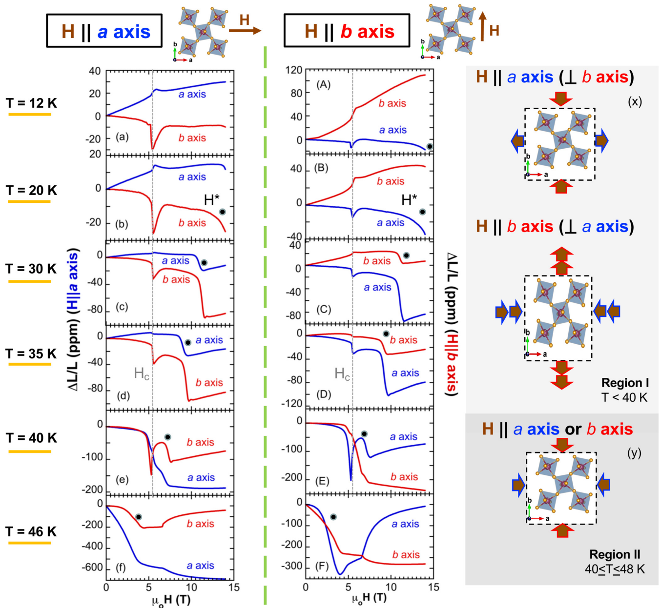
FIG. 2. The magnetic field dependence of magnetostriction \Delta L/L (a)–(f) for \Delta L/L ( H||a axis) and (A)–(F) for \Delta L/L ( H||b axis) at six representative temperatures; (x), (y) Schematic illustrations of the magnetostrictive effects on the lattice. Note that H^* is marked by the black solid circles, and H_c by the light-gray dashed line.
