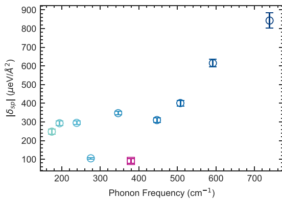
FIG. 4. Absolute value of the spin-phonon interaction strength evaluated with the mean-field model for the phonon modes in YIG. The measured \delta_{sp} for the \omega_{378} mode is negative (purple square), while the rest of the measured \delta_{sp} are positive.
