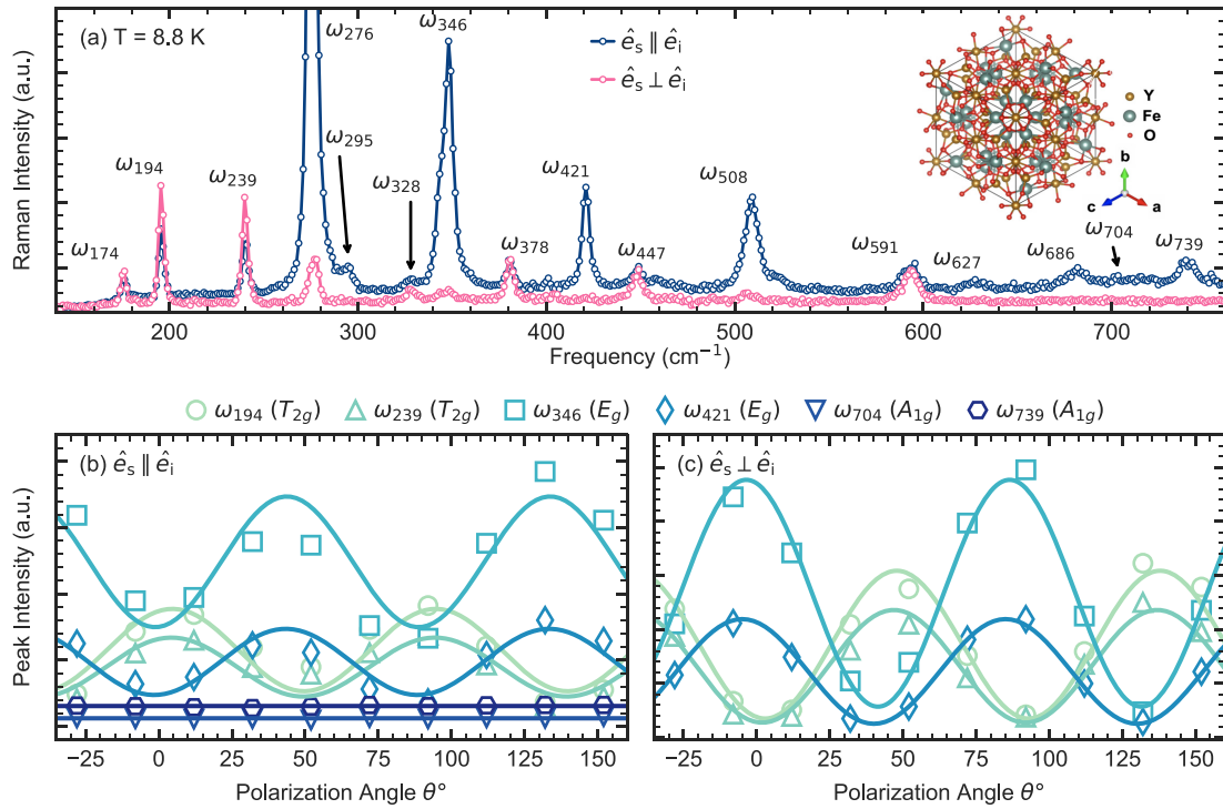
FIG. 1. (a) Raman spectra taken with \hat{e}_s \parallel \hat{e}_i (colinear) and \hat{e}_s \perp \hat{e}_i (crossed) polarization configurations at 8.8 K. Solid lines connect data points for clarity. Inset shows the YIG crystal structure viewed along the [111] direction. (b), (c) Angle-dependent intensities of the representative A_{1g} , E_g , and T_{2g} modes. The spectra were obtained by keeping incident polarization fixed. Panels (b) and (c) refer to colinear and crossed polarization configurations, respectively. The fit curves follow theoretical predictions from crystal lattice symmetry.
