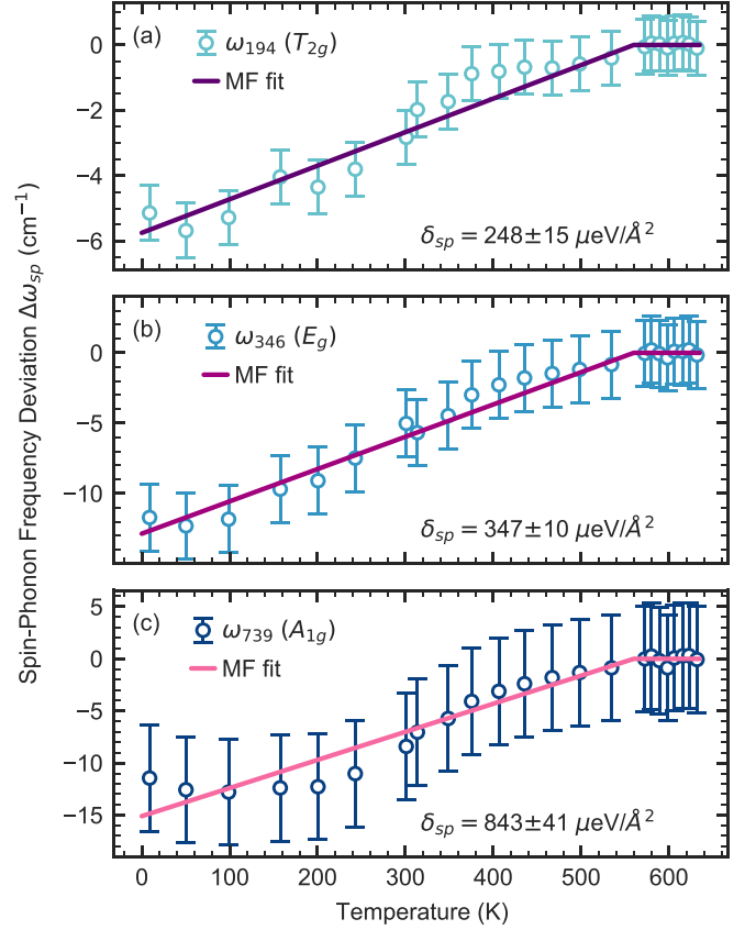
FIG. 3. The measured phonon frequencies are subtracted from the temperature-dependent frequency found with the anharmonic fit [see Figs. 2(b) and 2(c)] to determine \Delta\omega_{sp} . Solid lines show fits to the mean-field model which yield the spin-phonon interaction strength \delta_{sp} , given in Eq. (7).
