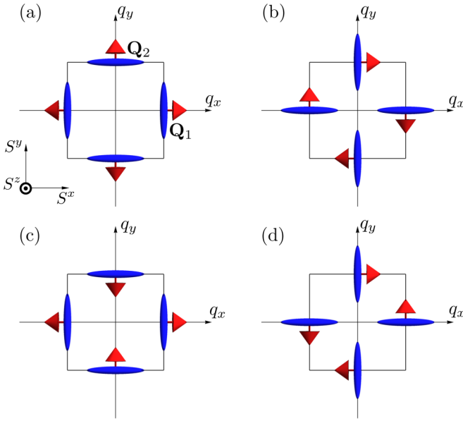
FIG. 3. Similar pictorial representations to Fig. 2 for the 2D models realizing the VCs of (a) proper-screw(I) [Eqs. (21) and (22)], (b) cycloid(I) [Eqs. (23) and (24)], (c) proper-screw(II) [Eqs. (25) and (26)], and (d) cycloid(II) [Eqs. (27) and (28)] types. The notations are common to those in Fig. 2.
