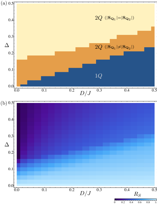
FIG. 14. Variational results for the infinite-range model in two dimensions. We take \Lambda = 16 . (a) Phase diagram, including the 1Q state, the anisotropic 2Q state with |\mathbf{S}_{\mathbf{Q}_1}| \neq |\mathbf{S}_{\mathbf{Q}_2}| , and the isotropic 2Q state with |\mathbf{S}_{\mathbf{Q}_1}| = |\mathbf{S}_{\mathbf{Q}_2}| . (b) Contour plot of the ratio of the Fourier components of spins, R_S \equiv |\mathbf{S}_{\mathbf{Q}_{\max}}^{\mu_{\perp,1}}|/|\mathbf{S}_{\mathbf{Q}_{\max}}^{\mu_{\perp,2}}| , representing the ellipticity of the constituent spin helix; see the text for the definition.
