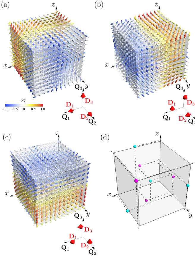
FIG. 19. Isotropic 3Q spin states in the infinite-range model in three dimensions with D/J = 0.3 , \Delta = 0.3 , and \Lambda = 12 : (a) proper-screw, (b) cycloid(I), and (c) cycloid(II) HLs. The forms of J_{\mathbf{Q}\eta}^{\alpha\alpha} and \mathbf{D}_{\mathbf{Q}\eta} in each case are summarized in Table I. Insets show \mathbf{D}_{\mathbf{Q}\eta} as well as \mathbf{Q}_\eta for each case. The color of arrows indicates the z component of spin according to the color bar in (a). (d) Positions of the hedgehogs (magenta spheres) and the antihedgehogs (cyan spheres), which are common to all the HLs shown in (a)–(c). The dashed lines are the guides for eyes.
