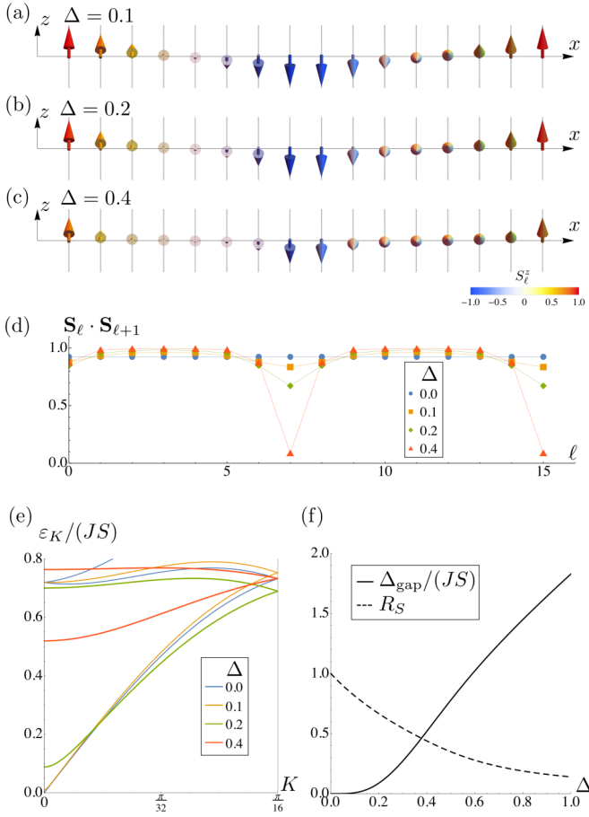
FIG. 11. Effect of the anisotropy \Delta in the symmetric interactions [Eq. (15)] for the 1D finite-range model with \Lambda = 16 , D/J = 0.2 , and \gamma = 0.3 . [(a)–(c)] Stable spin configurations for (a) \Delta = 0.1 , (b) \Delta = 0.2 , and (c) \Delta = 0.4 . The color of arrows indicates the z component of spin according to the color bar in (c). (d) Inner product of nearest-neighbor spins, \mathbf{S}_\ell \cdot \mathbf{S}_{\ell+1} , representing the spatial modulation of the spin twist. (e) Spin excitation spectra for different \Delta . (f) \Delta dependences of the spin excitation gap \Delta_{\text{gap}} and the ratio of the Fourier components of spins, R_S = |\mathcal{S}_Q^z|/|\mathcal{S}_Q^y| .
