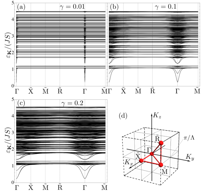
FIG. 20. Spin excitation spectra in the isotropic 3Q spin states in three dimensions for (a) \gamma = 0.01 , (b) \gamma = 0.1 , and (c) \gamma = 0.2 . We take D/J = 0.3 , \Delta = 0.3 , and \Lambda = 12 , as in Fig. 19. (d) Symmetric lines in the folded Brillouin zone, used for the plots in (a)–(c).
