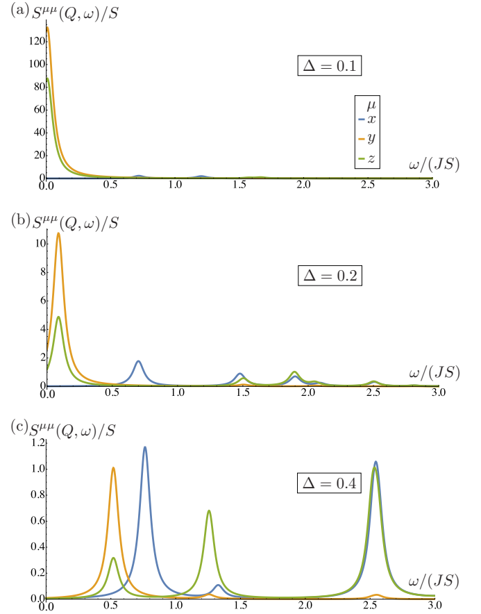
FIG. 12. The dynamical spin structure factor S^{\mu\mu}(q, \omega)/S at q = Q for (a) \Delta = 0.1 , (b) \Delta = 0.2 , and (c) \Delta = 0.4 . The model and parameters are the same as Fig. 11.
