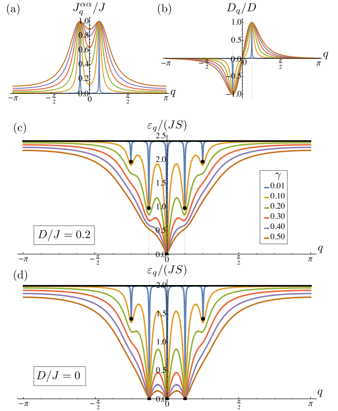
FIG. 9. Interaction range \gamma dependences of (a) the symmetric interaction J_q = J_q^{\alpha\alpha} , (b) the antisymmetric interaction D_q , and [(c) and (d)] the spin-wave dispersion \varepsilon_q for the isotropic case ( \Delta = 0 ) with \Lambda = 16 in one dimension. The antisymmetric interaction is set to (c) D/J = 0.2 and (d) D/J = 0 . The black dots and lines in (c) and (d) represent the results in the infinite-range limit of \gamma \rightarrow 0 ; see also Fig. 8.
