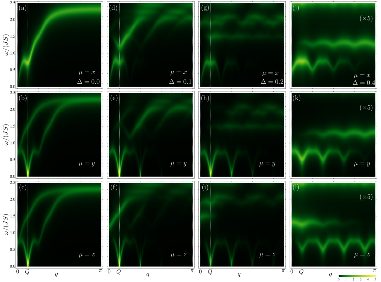
FIG. 10. Anisotropy dependence of the dynamical spin structure factor S^{\mu\mu}(q, \omega)/S for the proper-screw HS state in one dimension. The anisotropy \Delta is set to [(a)–(c)] \Delta = 0 (the isotropic case), [(d)–(f)] \Delta = 0.1 , [(g)–(i)] \Delta = 0.2 , and [(j)–(l)] \Delta = 0.4 . Panels (a), (d), (g), and (j); (b), (e), (h), and (k); and (c), (f), (i), and (l) show the \mu = x, y , and z components, respectively. The color bar is common to all plots whereas the data for \Delta = 0.4 in (j)–(l) are plotted by multiplying a factor of 5 for better visibility. The parameters are taken as \Lambda = 16 , D/J = 0.2 , \gamma = 0.3 , and \epsilon = 0.1 .
