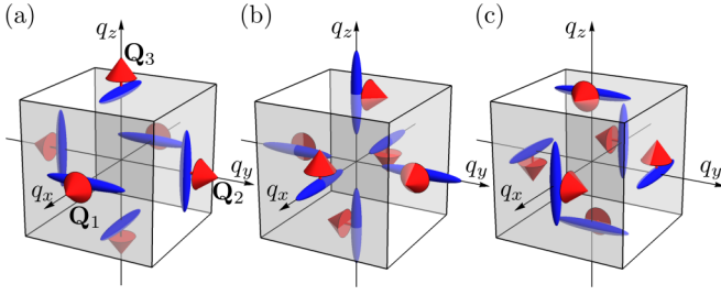
FIG. 4. Similar pictorial representations to Fig. 2 for the 3D models realizing the HLs of (a) proper-screw [Eqs. (29) and (30)], (b) cycloid(I) [Eqs. (31) and (32)], and (c) cycloid(II) [Eqs. (33) and (34)] types. The notations are common to those in Fig. 2.
