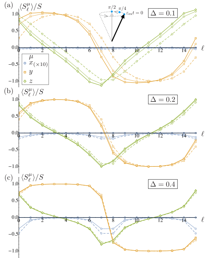
FIG. 13. Time evolution of the lowest-energy excitation mode at K = 0 for (a) \Delta = 0.1 , (b) \Delta = 0.2 , and (c) \Delta = 0.4 . The data connected by the solid, dotted, and dashed lines indicate the spin configurations obtained by Eq. (83) with \varepsilon_{\text{ex}}t = 0, \pi/4 , and \pi/2 , respectively, for \lambda = 0.1 . The model and parameters are the same as Fig. 11. Inset of (a) shows a schematic view of a spin precession motion (black arrow) around the ground state (gray arrow).
