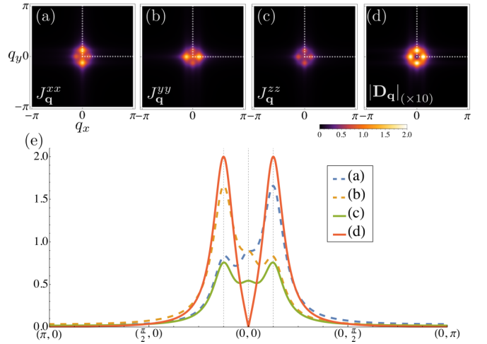
FIG. 6. \mathbf{q} = (q_x, q_y) dependences of (a) J_q^{xx} , (b) J_q^{yy} , (c) J_q^{zz} , and (d) |\mathbf{D}_q| in the 2D finite-range model. The color bar is common to (a)–(d), while |\mathbf{D}_q| in (d) is plotted by multiplying a factor of 10 for better visibility. (e) Profile of (a)–(d) along the path (\pi, 0) \rightarrow (0, 0) \rightarrow (0, \pi) [white dotted lines in (a)–(d)]. We take \Lambda = 16 , \gamma = 0.2 , J = 1 , D = 0.2 , and \Delta = 0.3 . The values for Q_j^* and Q_D^* are the same as those in Fig. 5.
