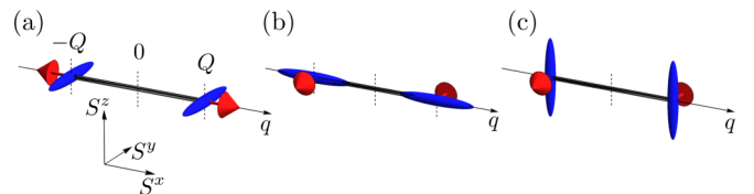
FIG. 2. Pictorial representations of the coupling constants for the symmetric and antisymmetric interactions in the 1D models for (a) proper-screw [Eqs. (14) and (15)], (b) cycloid(I) [Eqs. (16) and (17)], and (c) cycloid(II) [Eqs. (17) and (18)] HS states. The blue ellipsoids represent J_{\pm Q}^{\alpha\alpha} : the lengths along the principal axes [100], [010], and [001] denote the amplitudes of J_{\pm Q}^{xx} , J_{\pm Q}^{yy} , and J_{\pm Q}^{zz} , respectively. The red arrows represent \mathbf{D}_{\pm Q} . The axes for the spin space are shown in (a).
