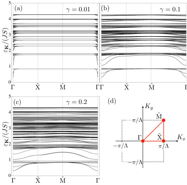
FIG. 16. Spin excitation spectra in the isotropic 2Q spin states in two dimensions while changing the parameter for the interaction range: (a) \gamma = 0.01 , (b) \gamma = 0.1 , and (c) \gamma = 0.2 . We take D/J = 0.2 , \Delta = 0.3 , and \Lambda = 16 , as in Fig. 15. (d) Symmetric lines in the folded Brillouin zone, used for the plots in (a)–(c).
