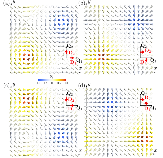
FIG. 15. Isotropic 2Q spin states stabilized in the infinite-range model in two dimensions with D/J = 0.2 , \Delta = 0.3 , and \Lambda = 16 : (a) proper-screw(I), (b) cycloid(I), (c) proper-screw(II), and (d) cycloid(II) VCs. The forms of J_{\mathbf{Q}_\eta}^{\alpha\alpha} and \mathbf{D}_{\mathbf{Q}_\eta} in each case are summarized in Table I. The configurations of \mathbf{D}_{\mathbf{Q}_\eta} as well as \mathbf{Q}_\eta are shown in each figure. The color of arrows indicates the z component of spin according to the color bar in (a).
