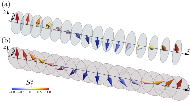
FIG. 1. Helimagnetic orders: (a) proper-screw and (b) cycloidal helical spin states. The latter is obtained by \pi/2 spin rotation of the former about the z axis.
