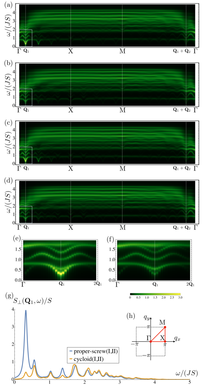
FIG. 17. Transverse component of the dynamical spin structure factor, S_{\perp}(\mathbf{q}, \omega) in Eq. (61), for (a) proper-screw(I), (b) cycloid(I), (c) proper-screw(II), and (d) cycloid(II) VCs, plotted along the symmetric lines in the first Brillouin zone shown in (h). (e) and (f) show the enlarged views of the dotted areas in (a) and (c) and then (b) and (d), respectively. (g) \omega dependence at \mathbf{q} = \mathbf{Q}_1 . The interaction range and the relaxation rate are taken as \gamma = 0.2 and \epsilon = 0.05 , respectively. The other parameters are \Lambda = 16 , D/J = 0.2 , and \Delta = 0.3 as in Fig. 15.
