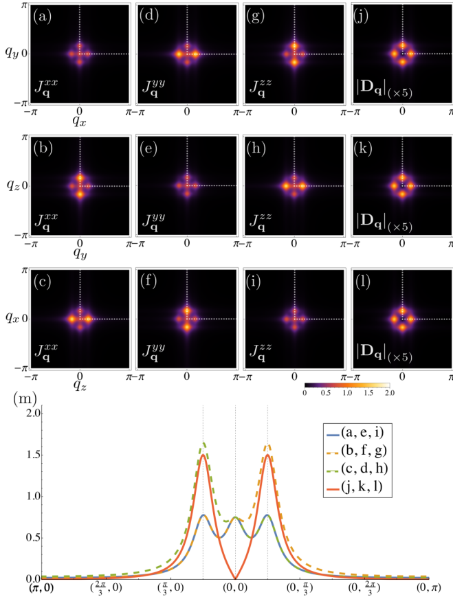
FIG. 7. \mathbf{q} = (q_x, q_y, q_z) dependences of [(a)–(c)] J_{\mathbf{q}}^{xx} , [(d)–(f)] J_{\mathbf{q}}^{yy} , [(g)–(i)] J_{\mathbf{q}}^{zz} , and [(j)–(l)] |\mathbf{D}_{\mathbf{q}}| in the 3D finite-range model. Panels (a), (d), (g), and (j); (b), (e), (h), and (k); and (c), (f), (i), and (l) show the q_z = 0 , q_x = 0 , and q_y = 0 planes, respectively. The color bar is common to (a)–(l), while |\mathbf{D}_{\mathbf{q}}| in (j), (k), and (l) are plotted by multiplying a factor of 5 for better visibility. (m) Profile along the white dotted lines in (a)–(l). We take \Lambda = 12 , \gamma = 0.2 , J = 1 , D = 0.3 , and \Delta = 0.3 . Q_j^* and Q_D^* are set to Q_j^* = 0.525 and Q_D^* = 0.522 so that J_{\mathbf{q}}^{\alpha\alpha} and |\mathbf{D}_{\mathbf{q}}| take their maxima at q = \pm Q = \pm\pi/6 .
