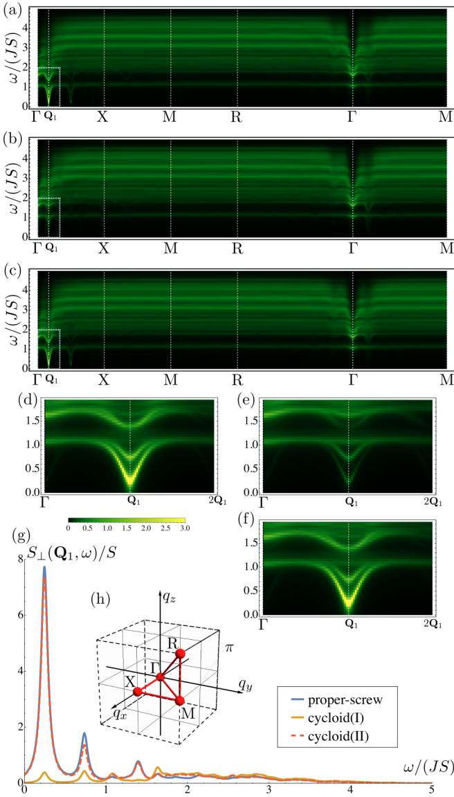
FIG. 21. Transverse component of the dynamical spin structure factor, S_{\perp}(\mathbf{q}, \omega) in Eq. (61), for (a) proper-screw, (b) cycloid(I), and (c) cycloid(II) HLs, plotted along the symmetric lines in the first Brillouin zone shown in (h). (d), (e), and (f) show the enlarged views of the dotted areas in (a), (b), and (c), respectively. (g) \omega dependence at \mathbf{q} = \mathbf{Q}_1 . The interaction range and the relaxation rate are taken as \gamma = 0.2 and \epsilon = 0.05 , respectively. The other parameters are \Lambda = 12 , D/J = 0.3 , and \Delta = 0.3 as in Fig. 19.
