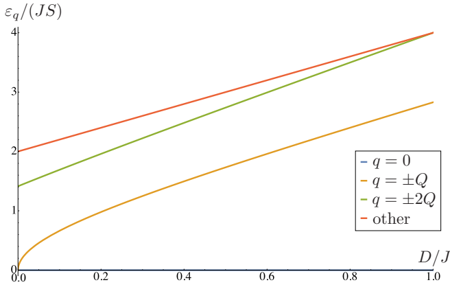
FIG. 8. D dependence of the spin excitation energy \varepsilon_q of the infinite-range model ( \gamma = 0 ) with the isotropic symmetric interactions ( \Delta = 0 ) in one dimension for q = 0 (blue), q = \pm Q (orange), q = \pm 2Q (green), and the other generic q (red) [Eq. (74)].
