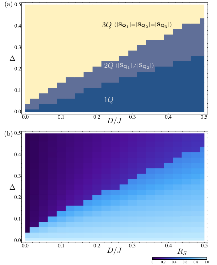
FIG. 18. Variational results for the infinite-range model in three dimensions. We take \Lambda = 12 . (a) Phase diagram, which includes the 1Q state, the anisotropic 2Q state with |\mathbf{S}_{\mathbf{Q}_1}| > |\mathbf{S}_{\mathbf{Q}_2}| \neq 0 and \mathbf{S}_{\mathbf{Q}_3} = 0 (the cyclic permutations of \mathbf{Q}_\eta are energetically degenerate) and the isotropic 3Q state with |\mathbf{S}_{\mathbf{Q}_1}| = |\mathbf{S}_{\mathbf{Q}_2}| = |\mathbf{S}_{\mathbf{Q}_3}| . (b) Contour plot of the ratio of the Fourier components of spins, R_S , defined in Sec. IV B 1 and Fig. 14.
