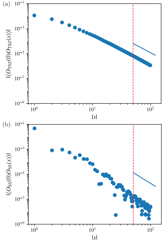
FIG. 8. Pairing quasi-long-range orders of a state in \pi SG phase. The parameters of the state: U = 3 , \alpha = 0.8 , and filling 5/11 . The asymptotic behavior of the TSCz order (a) is predicted as \sim 1/r^{1/K} ; while for the “s-wave” order (b) is \cos(2k_F x)/r^{1/K+K} . K can be independently extracted by SDWz/CDW order (Fig. 7). Using the extracted value 0.406, we plot 1/r^{1/K} and 1/r^{K+1/K} (the solid lines) in the first and second figure respectively, approximately matching the leading decaying slope of the numerical data. Note that the asymptotic behavior should be found at distance beyond the correlation length of the spin boson [estimated in the (1,0) and (0,1) sectors and denoted by the red dashed lines].
