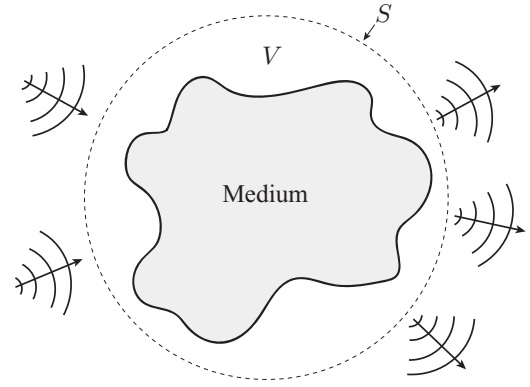
FIG. 2. Application of the Poynting theorem showing electromagnetic waves impinging on and being scattered by a lossless and gainless medium possessing dipolar and quadrupolar responses. Energy conservation requires that the energy entering V equals the energy leaving it.
