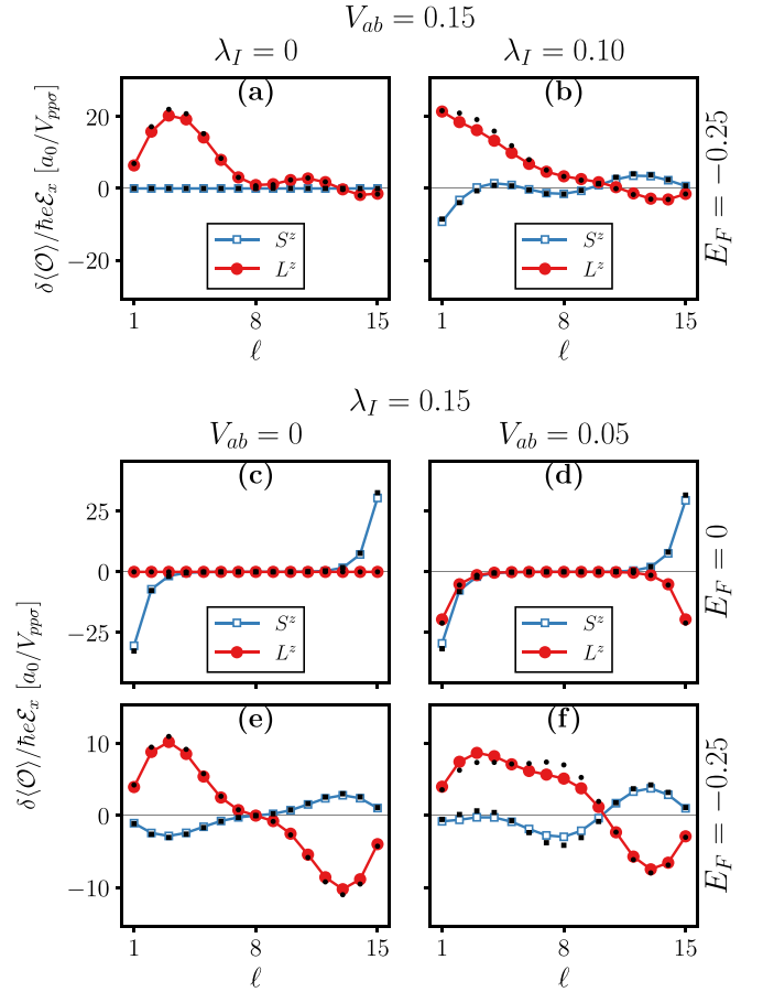
FIG. 2. Spin and OAM accumulation profiles induced by an applied electric field across ZZ nanoribbons with 15 atomic lines wide. \delta\langle S_\ell^z\rangle and \delta\langle L_\ell^z\rangle are calculated per atom in each atomic line \ell of the ribbon. Results for V_{AB} = 0.15 and E_F = -0.25 with (a) \lambda_I = 0 and (b) 0.10. Results obtained for V_{AB} = 0 and \lambda_I = 0.15 with (c) E_F = 0 and (e) E_F = -0.25 . (d) and (f) Results for V_{AB} = 0.05 , \lambda_I = 0.15 , and the same values of E_F as in (c) and (e), respectively. Black squares and circles represent the results obtained by means of an alternative approach (see text) for the spin and OAM accumulations, respectively. Here, we used \Gamma = 10^{-3} .
