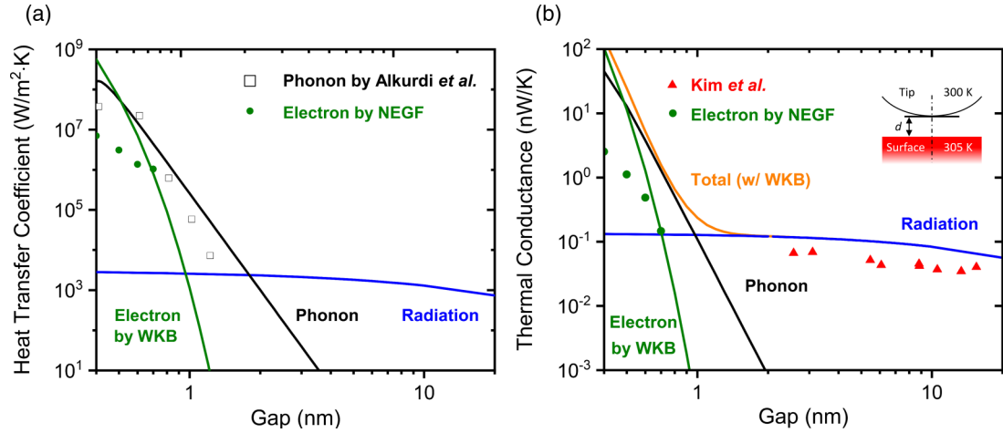
FIG. 2. (a) Heat transfer coefficients due to radiation, phonon, and electron between two Au surfaces separated by a vacuum gap \bar{d} ( T_L = 305 K, T_R = 300 K, V_{\text{bias}} = 0 V). The electron heat transfer coefficient is calculated via the WKB approximation and the NEGF. The phonon heat transfer coefficient predicted via the 1D AGF method is compared against the 3D lattice dynamics results of Alkurdi et al. [27]. (b) Thermal conductance between a 450-nm-radius tip (300 K) and a surface (305 K), both made of Au, separated by a vacuum gap d . The total conductance is calculated using the electron heat transfer coefficient from the WKB approximation. The predicted conductance is compared against the experimental results of Kim et al. [33].
