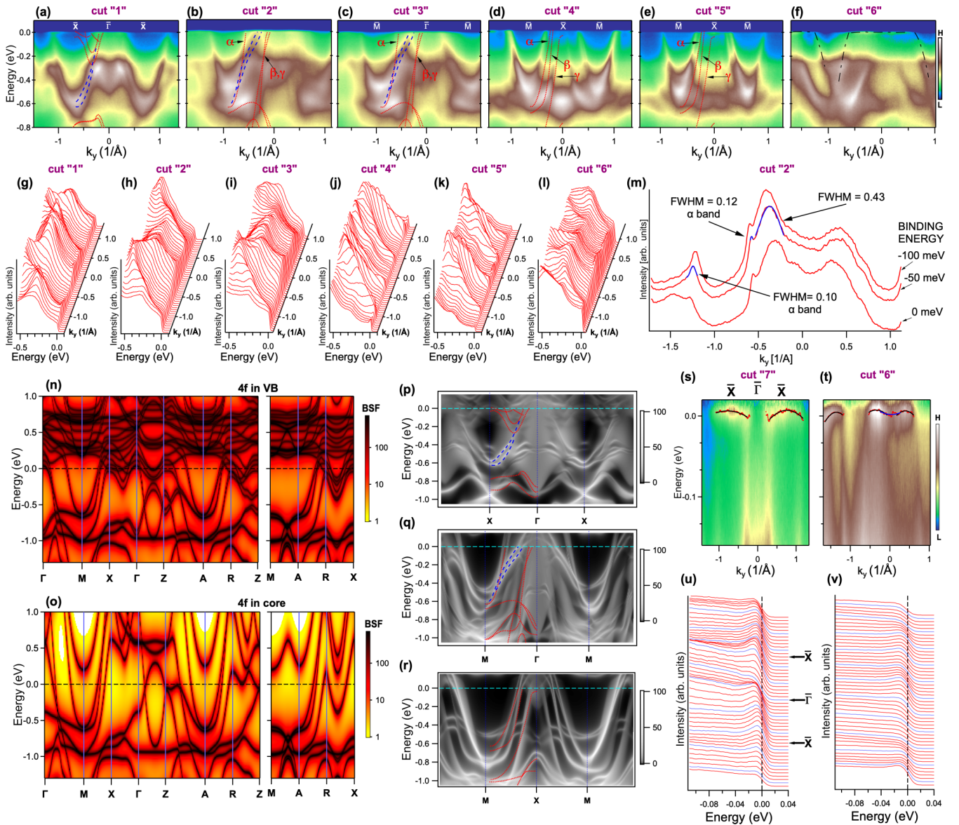
FIG. 2. Band structure of CeCoIn 5 along selected paths in k-space denoted as cut 1–cut 7 in Fig. 1. ARPES scans recorded with photon energy of 122 eV at T=6 K are shown along the paths: 1 ( \bar{X} - \bar{\Gamma} - \bar{X} ) (a), 2 ( \bar{M} - \bar{\Gamma} - \bar{M} ) (b), 3 (c), 4 ( \bar{M} - \bar{X} - \bar{M} ) (d), 5 ( \bar{M} - \bar{X} - \bar{M} ) (e), and 6 (f). The same band structures are represented in a form of EDCs in the corresponding panels (g)–(l). Red dotted lines represent bulk CeCoIn 5 dispersions obtained from BSF fitting, whereas blue dashed lines denote surface states, which appeared in one-step model simulations. The black dash-dot line in (f) is a guide to the eye, which shows the dispersion. Selected MDCs extracted from (b) are shown in (m) with full width at half maximum (FWHM) of the fitted Gaussian peaks. Panels (n) and (o) present BSFs along important crystallographic directions calculated with SPR-KKR package in presence ( 4f in VB) and absence ( 4f in core) of c - f hybridization effects, respectively. One-step model of photoemission simulations of ARPES spectra are presented for photon energy of 122 eV and Ce-In surface termination along X - \Gamma - X (p), M - \Gamma - M (q), and M - X - M (r) directions. The meaning and positions of red dotted and blue dashed lines is the same as in (a)–(e). Weakly dispersive band is visible near the Fermi level in spectra collected for cuts 7 (s) and 6 (t) shown in Fig. 1 after dividing by Fermi-Dirac distribution (FDD). Fitted dispersions are represented by black lines. The corresponding EDCs shown in (u) and (v) have not been normalized with FDD.
