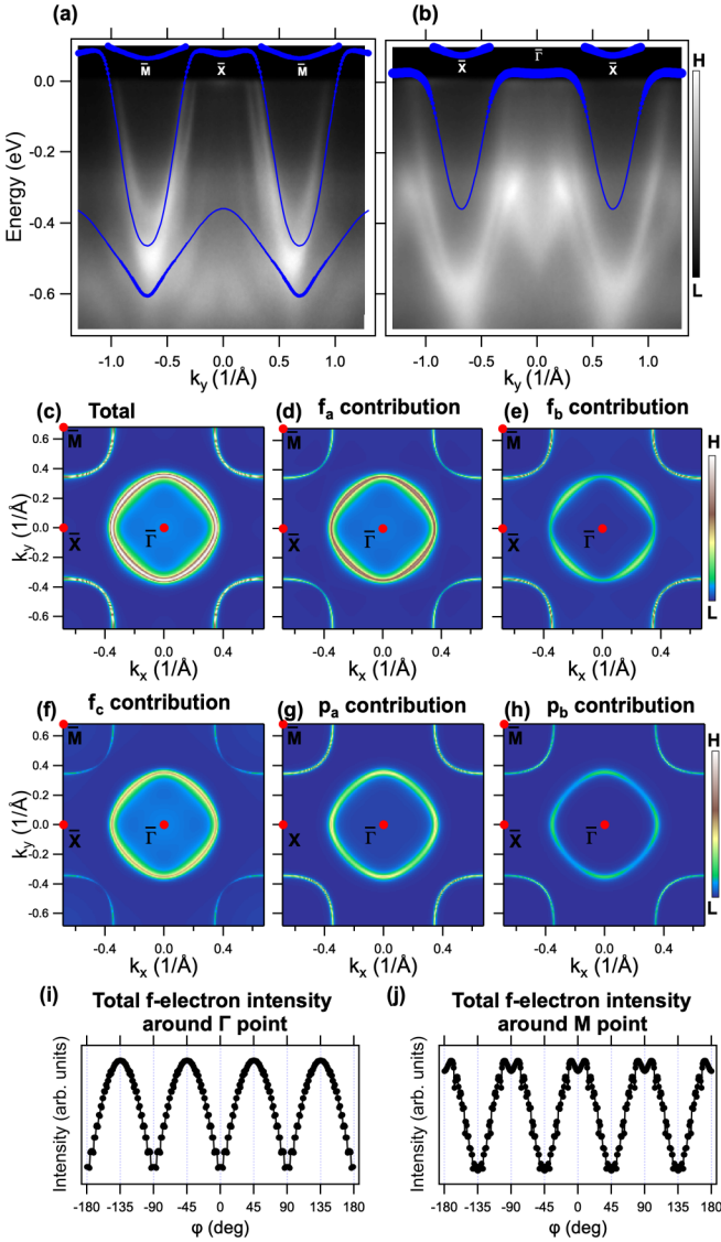
FIG. 8. Theoretical band structure for Ce-In planes (solid lines) obtained by tight-binding (TB) calculations. TB parameters have been adjusted by fitting theoretical bands to ARPES data with assumption (pp\pi) = 0 . This is the alternative version of TBA fit model presented in main part of the paper. The comparison of fitted model with the spectra collected along \bar{M} - \bar{X} - \bar{M} (a) and \bar{X} - \bar{\Gamma} - \bar{X} direction is shown. The marker size is proportional to the contribution of f orbital to the band. Panel (c) shows the distribution of the spectral weight on the Fermi surface. The projections on different base states are shown in (d)–(h). The Lorentzian broadening of 15 meV was applied to plot such maps. Panels (i) and (j) show total f -electron intensity extracted from TBA calculations along FS contours around \bar{\Gamma} and \bar{M} points. Azimuthal angle \phi = 0 corresponds to \bar{\Gamma} - \bar{X} direction in (i) and \bar{M} - \bar{X} direction in (j).
