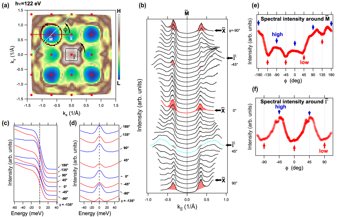
FIG. 3. (a) Symmetrized experimental Fermi surface obtained by a superposition of ARPES data rotated four times by 90^\circ . Red circle presents the pocket around \bar{M} subjected to f -electron intensity analysis. \phi is defined as the angle between horizontal \bar{M} - \bar{X} direction and the line crossing the particular point of the contour and \bar{M} point, measured in counterclockwise direction. (b) Momentum distribution curves extracted from symmetrized data along lines crossing \bar{M} point in different directions given by \phi . The exemplary red and cyan curves represent paths which are drawn with the same colors in (a). The peaks related to the contour around \bar{M} are highlighted with red area for \bar{M} - \bar{X} and \bar{\Gamma} - \bar{X} directions. (c) Energy distribution curves (EDCs) and (d) symmetrized EDCs from the electron pocket around \bar{M} for selected \phi angles. (e) Intensity at the Fermi energy along the electron pocket indicated with the red circle in (a) as a function of \phi . Red arrows in (e) denote the minima of intensity, which appear to be located along \bar{\Gamma} - \bar{M} direction, while blue arrows show \bar{M} - \bar{X} direction characterized with higher spectral intensity. (f) Intensity at the Fermi energy along the hole pocket around \bar{\Gamma} indicated by the black contour in (a) as a function of \phi_1 . Red arrows denote minima in intensity, which are complementary to those in (e).
