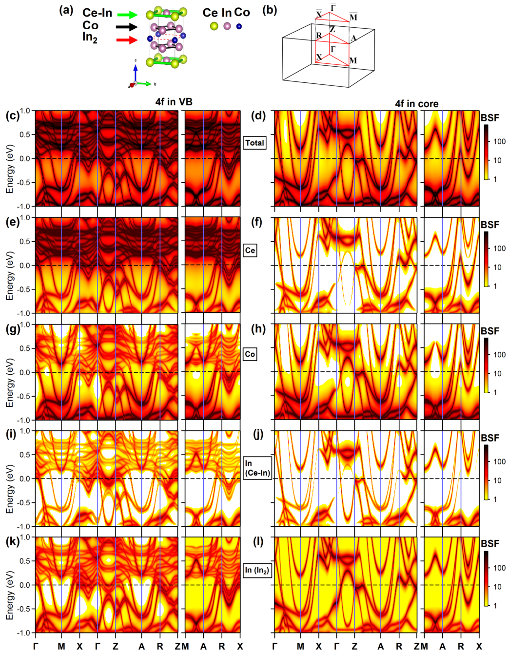
FIG. 6. Bloch spectral functions calculated along high symmetry directions in the BZ. (a) The crystal structure of CeCoIn 5 . (b) The first Brillouin zone with marked high symmetry points. Two types of calculations are provided: with included hybridization between 4f states and rest of orbitals [(c), (e), (g), (i), (k)], as well as the results without the hybridization (4f in core) [(d), (f), (h), (j), (l)]. The projections on Ce [(e), (f)], Co [(g), (h)], In from Ce-In planes [(i), (j)] and In from In planes [(k), (l)] are also provided.
