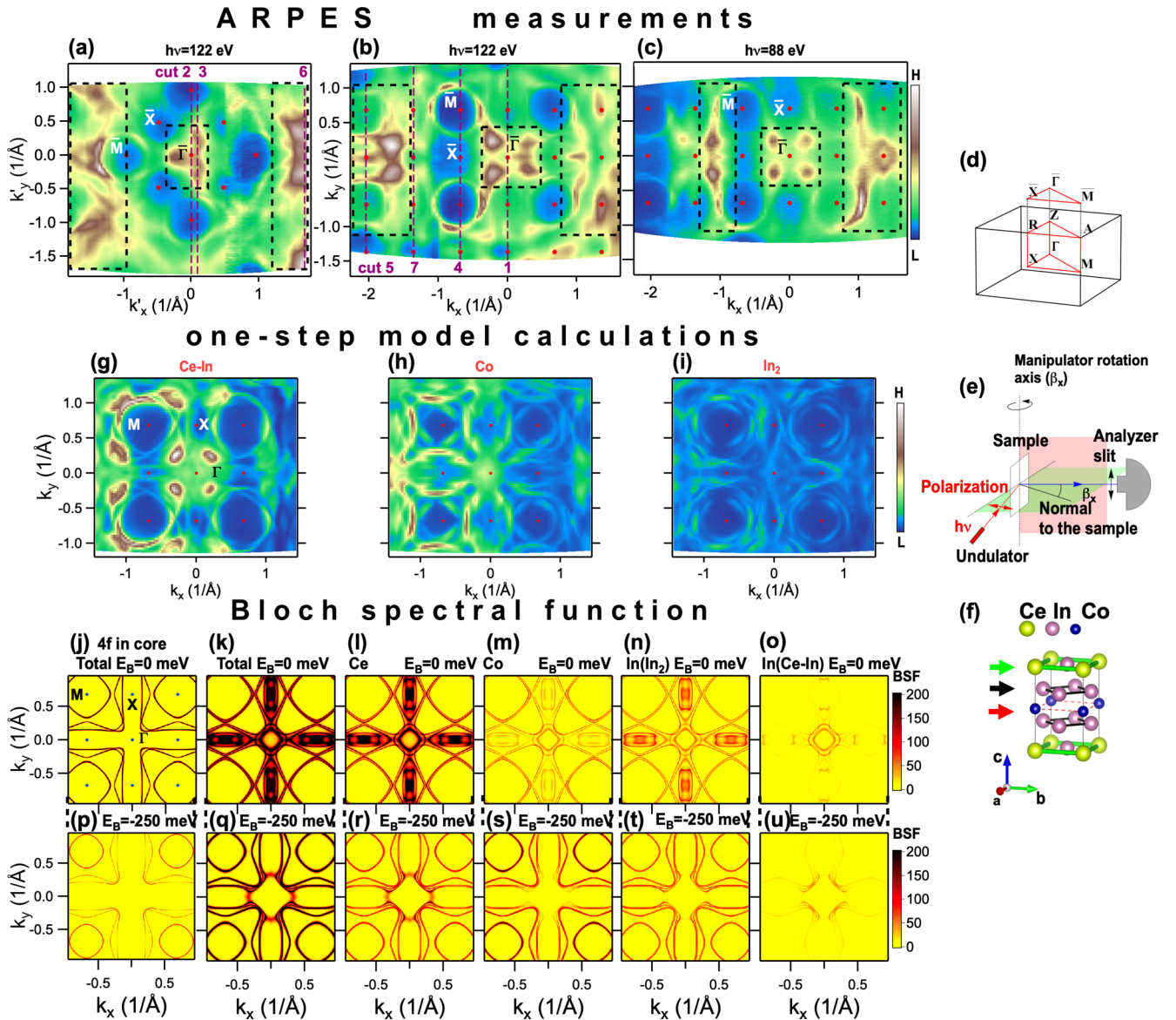
FIG. 1. Fermi surface of \text{CeCoIn}_5 . Intensity maps along Fermi surface obtained by ARPES at T = 6 K for photon energies of 122 eV (a), (b) and 88 eV (c). Black dashed rectangles enclose FS regions with higher spectral intensity. (d) Three-dimensional Brillouin zone and surface Brillouin zone with marked high symmetry points. (e) Geometry of the experiment. Rotation of the manipulator ( \beta_x ) corresponds to the variation of k'_x or k_x which depends on sample orientation. Linear horizontal polarization of the radiation is shown with red arrows. (f) Crystal structure of \text{CeCoIn}_5 . One-step model based simulation of the ARPES spectra obtained for photon energy of 122 eV for Ce-In (g), Co (h), \text{In}_2 (i) surface terminations. Constant energy contours at 0 eV (j)–(o) and -0.25 eV (p)–(u) of Bloch spectral functions obtained in SPR-KKR calculations. These represent a topology of the Fermi surface. The total Bloch spectral function (k), (q) is projected onto atomic wave functions of Ce (l), (r), Co (m), (s), In from \text{In}_2 layers (n), (t) and In from Ce-In planes (o), (u). The total Bloch spectral function calculated in the absence of hybridization effects (4f in core) is shown in (j) and (p)
