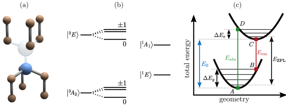
FIG. 1. (a) Atomic structure of the NV center in diamond. (b) Energy-level diagram of the NV center. Splitting of the magnetic sublevels is not to scale. (c) One-dimensional representation of adiabatic potential energy surfaces in the ground and the excited states. Points A and D represent equilibrium geometry of the ground state, while points B and C represent equilibrium geometry of the excited state. \Delta E_g and \Delta E_e are lattice relaxation energies. E_0 is energy difference between the potential energy minima, and E_{ZPL} is the energy of the zero-phonon line.
