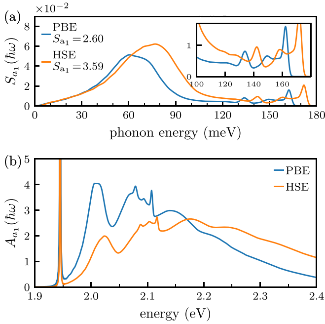
FIG. 6. (a) Spectral densities S_{a_1}(\hbar\omega) (in units \text{meV}^{-1} ) due to coupling to a_1 phonons for absorption, calculated with PBE and HSE functionals. Huang-Rhys factors are also given. The inset enlarges the high-frequency part. (b) Spectral functions A_{a_1}(\hbar\omega) [in units \text{eV}^{-1} , Eq. (15)] for absorption calculated using PBE and HSE. The ZPL energy is set to the experimental value.
