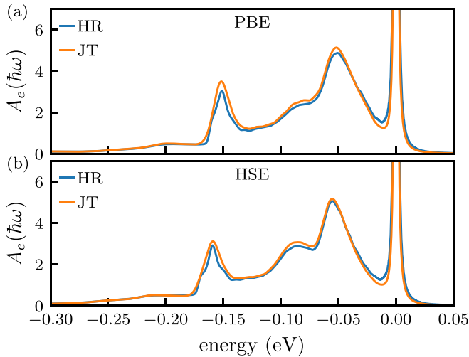
FIG. 8. The spectral function A_e(\hbar\omega) (in units \text{eV}^{-1} ) for emission [Eq. (14)] obtained with (a) PBE and (b) HSE functionals. We compare spectral functions obtained via the solution of the multi-mode Jahn-Teller problem (“JT”) and via the Huang-Rhys treatment (“HR”).
