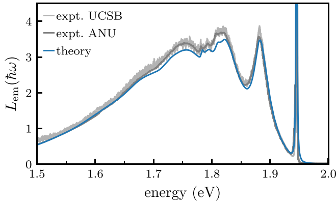
FIG. 12. Calculated normalized luminescence lineshape, compared with the experimental lineshape (both in units \text{eV}^{-1} ). In the calculations we used scaled PBE spectral densities S'_{a_1} = \zeta S_{a_1}(\hbar\omega) and S'_e = \zeta S_e(\hbar\omega) , with \zeta = 1.2 . Experimental spectra are as in Fig. 10.
