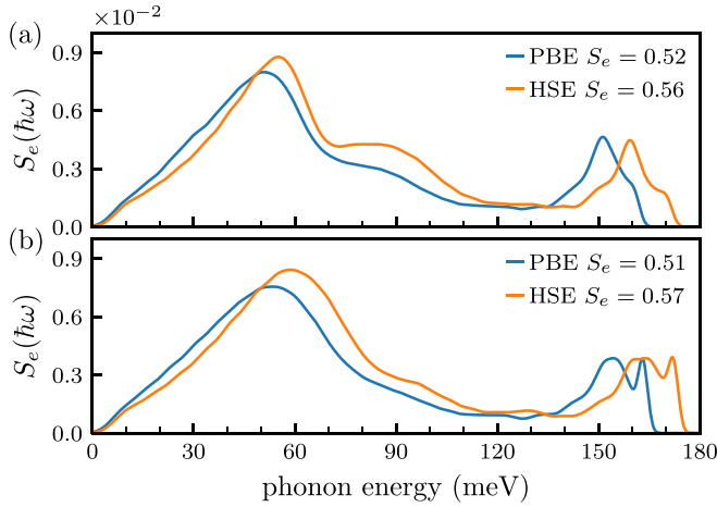
FIG. 7. Spectral density S_e(\hbar\omega) (in units \text{meV}^{-1} ) due to coupling to e phonons for (a) luminescence and (b) absorption, calculated with PBE and HSE functionals. Results are for the 20 \times 20 \times 20 supercell. Huang-Rhys factors are also given.
