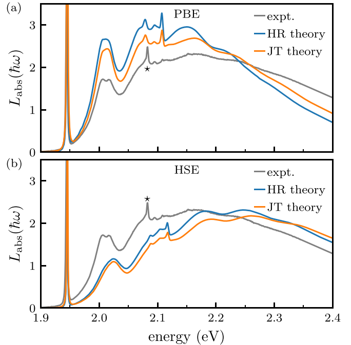
FIG. 11. Theoretical normalized absorption lineshapes (in units \text{eV}^{-1} ) calculated using the Huang-Rhys (labeled “HR theory”) and Jahn-Teller treatment (labeled “JT theory”), compared with the experimental spectrum: (a) PBE functional and (b) HSE functional. The experiment is from Ref. [54]. The ZPL energy of the theoretical curves is set to the experimental value. The small peak marked with a star “*” in the experimental curve is the ZPL of another center and should be disregarded in the comparison.
