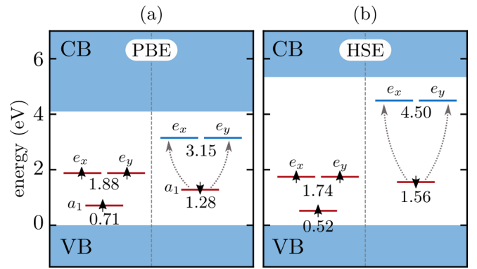
FIG. 3. Defect-level diagrams of the NV -1 center calculated using PBE (a) and HSE (b) functionals. Diagrams show Kohn-Sham single particle defect levels for the ground state {}^3A_2 . The spin-majority channel is denoted with upward arrows and the spin-minority channel is denoted with downward arrows. Shaded areas correspond to the valence band (VB) and the conduction band (CB). Dotted arrows show optical excitation.
