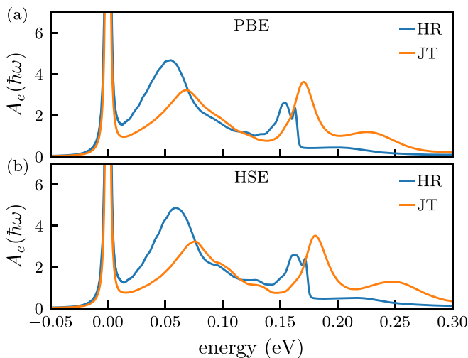
FIG. 9. The spectral function A_e(\hbar\omega) (in units \text{eV}^{-1} ) for absorption [Eq. (16)] obtained with (a) PBE and (b) HSE functionals. We compare spectral functions obtained via the solution of the multi-mode Jahn-Teller problem (“JT theory”) and via the Huang-Rhys treatment (“HR theory”).
