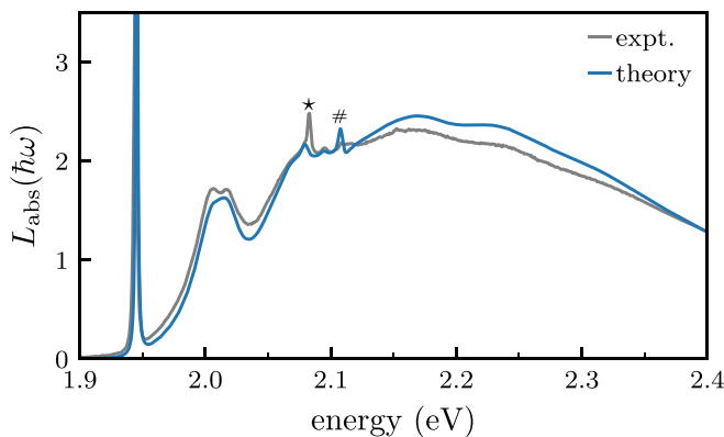
FIG. 13. Calculated normalized absorption lineshape, compared with the experimental lineshape (both in units \text{eV}^{-1} ). In the calculations we used scaled PBE spectral densities S'_{a_1} = \zeta S_{a_1}(\hbar\omega) and S'_e = \zeta S_e(\hbar\omega) , with \zeta = 1.2 . Experimental spectrum as in Fig. 11. The experimental peak marked “*” is the ZPL of another defect and should be disregarded in the comparison. The feature marked “#” in the calculated curve is discussed in the text.
