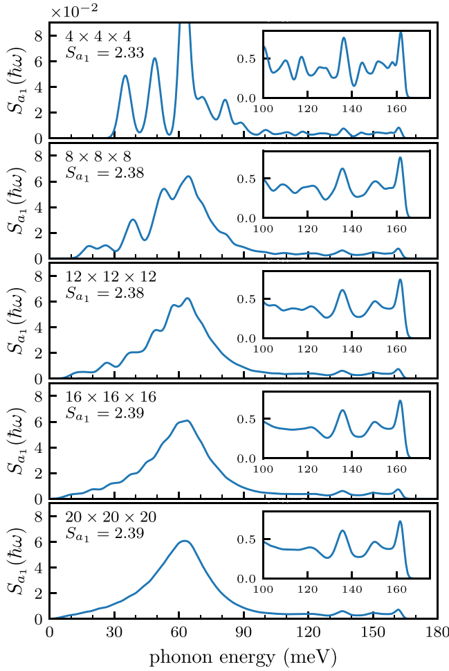
FIG. 4. Convergence of spectral densities S_{a_1}(\hbar\omega) (in units \text{meV}^{-1} ) due to coupling to a_1 phonons with respect to the supercell size. Supercells range in size from 4 \times 4 \times 4 (512 atomic sites) to 20 \times 20 \times 20 (64 000 sites). Huang-Rhys factors for each supercell are also given. The insets enlarge the high-frequency part. Gaussian smearing with varying \sigma was used, as explained in the text.
