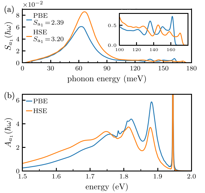
FIG. 5. (a) Spectral densities S_{a_1}(\hbar\omega) (in units \text{meV}^{-1} ) due to coupling to a_1 phonons for luminescence, calculated with PBE and HSE functionals. Huang-Rhys factors are also given. The inset enlarges the high-frequency part. (b) Spectral functions A_{a_1}(\hbar\omega) [in units \text{eV}^{-1} , Eq. (13)] for luminescence calculated using PBE and HSE. The ZPL energy is set to the experimental value.
