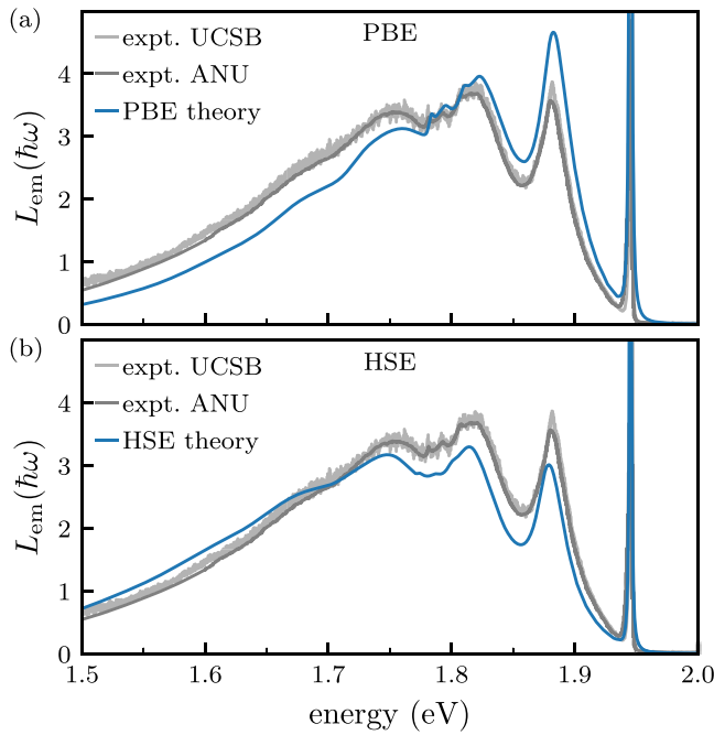
FIG. 10. Theoretical normalized luminescence lineshapes (in units \text{eV}^{-1} ), compared with experimental spectra: (a) PBE functional and (b) HSE functional. Experimental spectra from Refs. [55] (labeled “ANU”) and [8] (labeled “UCSB”). The ZPL energy of the theoretical curves is set to the experimental value.
