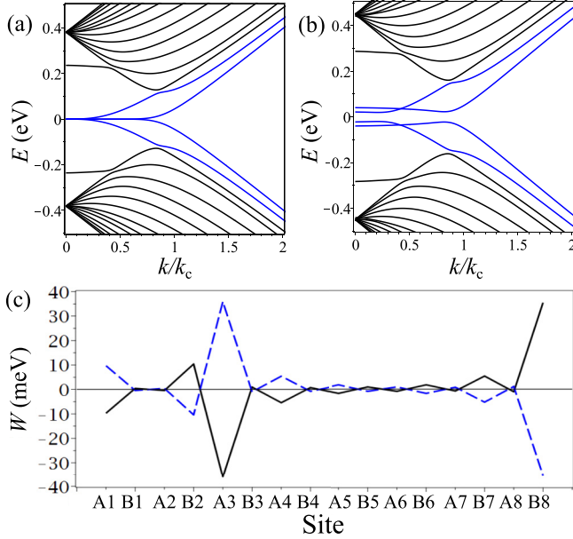
FIG. 9. Low-energy band structure of RMG with N = 16 layers and a Bernal stacking fault between its third and fourth layers, (m, n) = (3, 13) , with (a) noninteracting electrons described by Hamiltonian (1) and (b) interacting electrons described by the mean-field theory Eqs. (2) and (3) with interaction strength \alpha_g = 0.3 and zero temperature. Black lines are bulk bands, blue lines are surface bands for k \lesssim k_c where \hbar v k_c = \gamma_1 . (c) The values of the exchange potential W_{k=0\sigma XX} at the valley center k = 0 and for each site X' = X for RMG with N = 8 layers and a Bernal stacking fault off center [78] between the second and third layers, (m, n) = (2, 6) . The black solid line shows the exchange for two flavors, the blue dashed line is exchange for the other two flavors.
