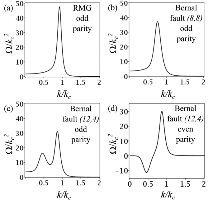
FIG. 4. Berry curvature \Omega(k) as a function of the magnitude of the wave vector k plotted from the valley center (the Berry curvature is isotropic in the minimal model) for N = 16 , \alpha_g = 0.3 , and T = 0 K. (a) is for pristine RMG in the odd parity ground state, (b) is for RMG with a Bernal stacking fault at its center in the odd parity ground state, (c) is for an off-centre Bernal stacking fault in the odd parity ground state, (d) is for an off-centre Bernal stacking fault in an even parity state (which is not the ground state).
