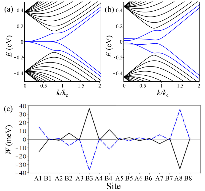
FIG. 13. Low-energy band structure of RMG with N = 16 layers and a twin boundary fault off center at its third layer, (m, n) = (3, 14) , with (a) noninteracting electrons described by Hamiltonian (1) and (b) interacting electrons described by the mean-field theory Eqs. [(2) and (3)] with interaction strength \alpha_g = 0.3 and zero temperature. Black lines are bulk bands, blue lines are surface bands for k \lesssim k_c where \hbar v k_c = \gamma_1 . (c) The values of the exchange potential W_{k=0\sigma XX} at the valley center k = 0 and for each site X' = X for RMG with N = 8 layers and a twin boundary stacking fault off center [78] at its third layer, (m, n) = (3, 6) . The black solid line shows the exchange for two flavors, the blue dashed line is exchange for the other two flavors.
