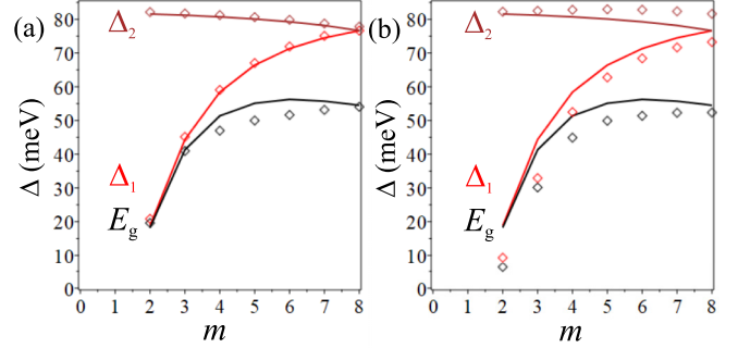
FIG. 10. (a) The band gap E_g and order parameters \Delta_1, \Delta_2 of RMG with N = 16 layers and a Bernal stacking fault of structure (m, 16 - m) consisting of a rhombohedral section of length m coupled to a rhombohedral section of length 16 - m . Points are data for the system with the stacking fault, solid lines are data from Fig. 3 for a single RMG section with m layers for \Delta_1 and E_g , and 16 - m layers for \Delta_2 . (b) The band gap E_g and order parameters \Delta_1, \Delta_2 of RMG with N = 15 layers and a twin boundary fault of structure (m, 16 - m) consisting of a rhombohedral section of length m coupled to a rhombohedral section of length 16 - m . Points are data for the system with the stacking fault, solid lines are data from Fig. 3 for a single RMG section with m layers for \Delta_1 and E_g , and 16 - m layers for \Delta_2 . For both plots, the interaction strength is \alpha_g = 0.3 and temperature T = 0 K.
