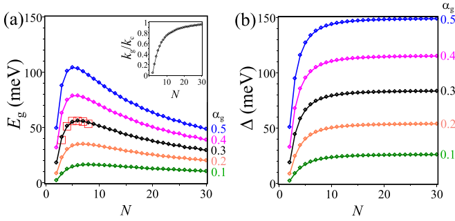
FIG. 3. The band gap of rhombohedral multilayer graphene at zero temperature as a function of layer number N for different values of interaction strength \alpha_g showing (a) the band gap E_g and (b) the order parameter \Delta . Solid lines are a guide for the eye. Red squares in (a) show the results of Ref. [64] for N = 3 to N = 8 obtained using density functional theory. The inset of (a) shows the position of the band gap k_g in units of k_c as a function of N for \alpha_g = 0.3 .
