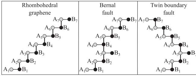
FIG. 1. Schematic side view of the lattice of rhombohedral graphene with N = 7 layers showing the pristine lattice, a lattice with a single Bernal stacking fault, and a lattice with a single twin boundary stacking fault. Labels indicate the A_n and B_n atomic sites on the n th layer, horizontal solid lines indicate intralayer hopping with parameter \gamma_0 , vertical solid lines indicate interlayer hopping \gamma_1 .
