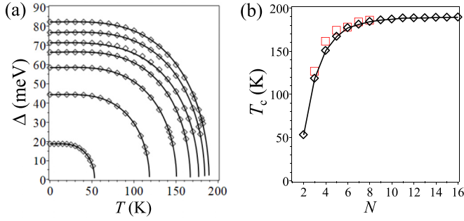
FIG. 5. (a) the order parameter \Delta(T) of rhombohedral multilayer graphene as a function of temperature T for interaction strength \alpha_g = 0.3 and layer number N = 2, 3, 4, 5, 6, 8 , and 16 from bottom to top. Solid lines are fits according to Eq. (21). (b) Critical temperature T_c as a function of layer number N for interaction strength \alpha_g = 0.3 obtained using the fit (21). The solid line is a guide to the eye. Red squares show the results of Ref. [64] for N = 3 to N = 8 obtained using density functional theory.
