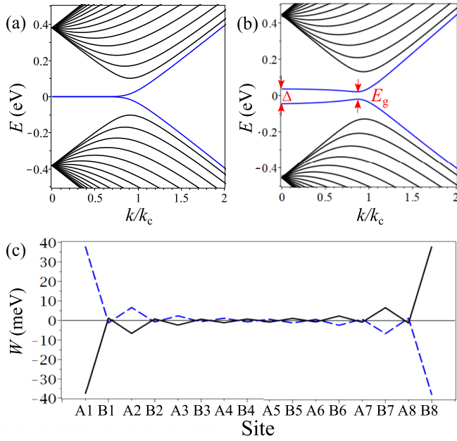
FIG. 2. Low-energy band structure of RMG with N = 16 layers with (a) noninteracting electrons described by Hamiltonian (1) and (b) interacting electrons described by the mean-field theory [(2 and 3)] with interaction strength \alpha_g = 0.3 and at zero temperature. Black lines are bulk bands, blue lines are surface bands for k \lesssim k_c where \hbar v k_c = \gamma_1 . E_g is the band gap (at k \approx k_c ), \Delta is the order parameter (the separation of the surface bands at k = 0 ). (c) The values of the exchange potential W_{k=0\sigma XX} at the valley center k = 0 and for each site X' = X for RMG with N = 8 layers [78]. The black solid line shows the exchange for two flavors, the blue dashed line is exchange for the other two flavors.
