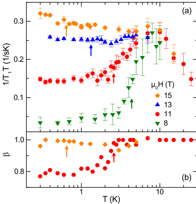
FIG. 3. (a) Temperature-dependent 1/T_1T of FeSe for fields parallel to the c axis. The arrows denote T_c as determined from the RF reflection and NMR intensity experiments, respectively. (b) Stretching exponent \beta of the T_1 relaxation as a function of temperature.
