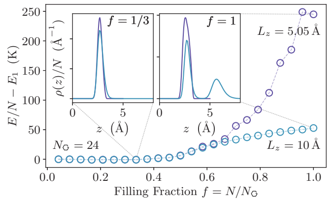
FIG. 17. Equation of state (energy per particle as a function of filling fraction) for N_G = 24 adsorption sites for two box sizes with L_z = 5.05 and 10.0 \text{ \AA} . The curves have been shifted by the energy for a single particle N = 1 corresponding to a filling fraction-independent value of \sim 6 \text{ K} due to the presence of \mathcal{V}_{\text{wall}} . The insets show the density of particles along the z direction at filling fractions f = 1/3 and 1 . For unit filling, the cell with L_z = 10 \text{ \AA} can accommodate a second layer.
