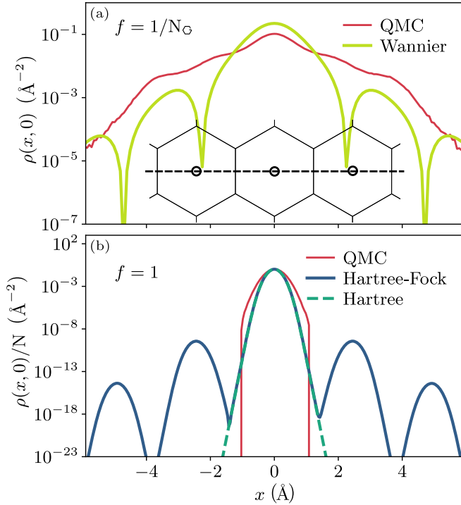
FIG. 7. Spatial dependence of the density \rho(x, y) = |\psi(x, y)|^2/N of an adsorbed {}^4\text{He} atom on graphene for a y = 0 cut in the xy -plane corresponding to the lattice path shown in the top inset. (a) A comparison of the localized Wannier function defined in Eq. (13) to that computed via quantum Monte Carlo (QMC) for a single particle N = 1 , f = 1/N_G by slightly biasing a single site at the level of the trial wave function as discussed in Sec. IV E. The wave function strongly penetrates into neighboring lattice sites, leading to the breakdown of Wannier theory for the computation of interaction parameters. (b) The density at unit filling N = N_G as computed via QMC, and within the Hartree-Fock and Hartree approximations showing the tendency towards exponential localization on a single site. In both panels, the 2D normalization is computed over the full graphene sheet.
