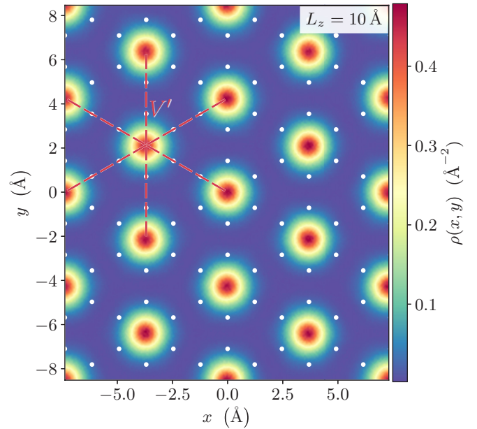
FIG. 10. The two-dimensional density of particles \rho(x, y) obtained from ground state quantum Monte Carlo simulations for a simulation cell with L_x \times L_y \times L_z = 14.75707 \times 17.04 \times 10.0 \text{ \AA} corresponding to the C1/3 phase with f = 1/3 for N = 16 {}^4\text{He} atoms on N_G = 48 adsorption sites. Finite size effects in the spatial wave function are negligible beyond N_G = 12 .
