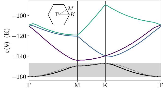
FIG. 6. The band structure obtained using \tilde{\mathcal{V}}_{\text{He-G}}(z) as introduced Eq. (A4c) along a high-symmetry path in the first Brillouin zone as shown in the inset. The first band (with n=1 ) is well separated from the higher excited bands and thus the low energy properties of the system are determined by the lowest band. The dashed line shows the tight-binding dispersion from Eq. (15), in excellent agreement with the continuum model supporting the use of an effective 2D lattice model. The shaded region corresponds to the bandwidth equal to 9t by symmetry.
