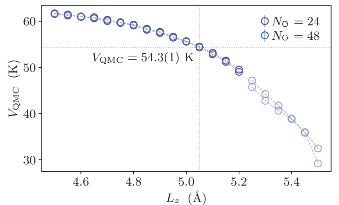
FIG. 12. The effective nearest-neighbor interaction parameter of the Bose-Hubbard model computed from Eq. (29) via quantum Monte Carlo for simulation cells with N_{\text{G}} = 24 and 48 as a function of the cell size in the z direction, L_z . The indicated value of V_{\text{QMC}} = 54.3(1) \text{ K} was computed at L_z = 5.05 \text{ \AA} as described in the text. The semi-transparent symbols for L_z \geq 5.25 \text{ \AA} indicate cell sizes which allowed the nascent formation of a second layer, where the mapping of the microscopic Hamiltonian to the 2D Bose-Hubbard model breaks down.
