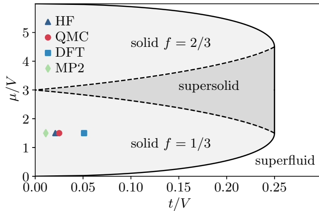
FIG. 3. The mean-field phase diagram for hard-core bosons on the triangular lattice with nearest-neighbor interactions V and hopping t with density controlled by the chemical potential \mu . Identified phases include commensurate solids (at fillings f = 1/3 and 2/3 ), superfluid, and supersolid (a superfluid that breaks triangular lattice symmetries). Solid lines indicate discontinuous (first-order) transitions, while continuous (second-order) transitions occur across dashed lines. The data points in the lower left-hand corner represent the major results of this paper, indicating that the ground state of a single layer of ^4\text{He} on graphene resides deep in the commensurate solid phase at 1/3 filling. For these data points, the chemical potential has been chosen such that \mu/V has the same value as the tip of the first lobe.
