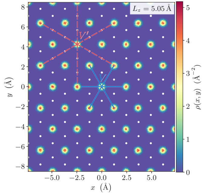
FIG. 11. The two-dimensional density of particles \rho(x, y) obtained from ground state quantum Monte Carlo simulations for a simulation cell with L_x \times L_y \times L_z = 14.75707 \times 17.04 \times 5.05 \text{ \AA} corresponding to the fully filled phase with f = 1 for N = 48 {}^4\text{He} atoms on N_{\text{G}} = 48 adsorption sites. Finite size effects in the spatial wave function are negligible beyond N_{\text{G}} = 12 . nearest-neighbor ( V ) and next-nearest-neighbor ( V' ) couplings in the effective Bose-Hubbard description are indicated with solid and dashed lines, respectively.
