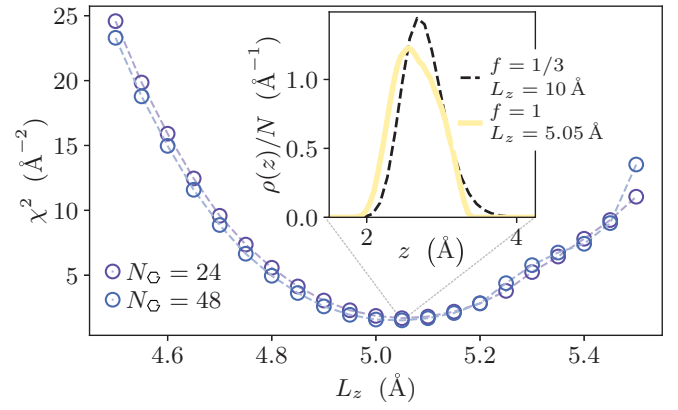
FIG. 16. The squared deviation between solid and dashed curves in Fig. 15(a) as a function the box size in the z direction as quantified in Eq. (B1). The minimum at L_z = 5.05 \text{ \AA} is independent of the size of the graphene sheet, where data for N_G = 24 and 48 are shown. The inset shows a comparison of the density profiles in the z direction for this value at N_G = 48 . The dashed line is a guide to the eye.
