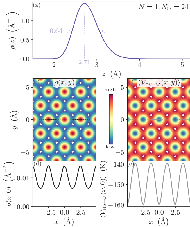
FIG. 9. Quantum Monte Carlo results for a single {}^4\text{He} atom ( N = 1 ) above a graphene membrane with N_G = 24 adsorption sites. (a) The average density in the z direction showing a well defined particle position a distance 2.71 \text{ \AA} above the sheet with a width of 0.64 \text{ \AA} . (b) The average density in the xy plane showing the ability of a single particle to hop between the sites of the triangular lattice. White dots show the location of carbon atoms (not to scale). (c) The average potential energy experienced by the {}^4\text{He} atom due to the graphene sheet in the xy plane. (d) A horizontal cut of the particle density \rho(x, y) along the line y = 0 . (e) A horizontal cut of the adsorption potential \mathcal{V}_{\text{He-G}}(x, y) along the line y = 0 .
