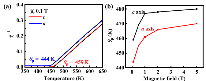
FIG. 2. (a) Temperature dependence of inverse susceptibility along both the c and the a axes. (b) Magnetic-field dependence of \theta_p along the c and a axes.
