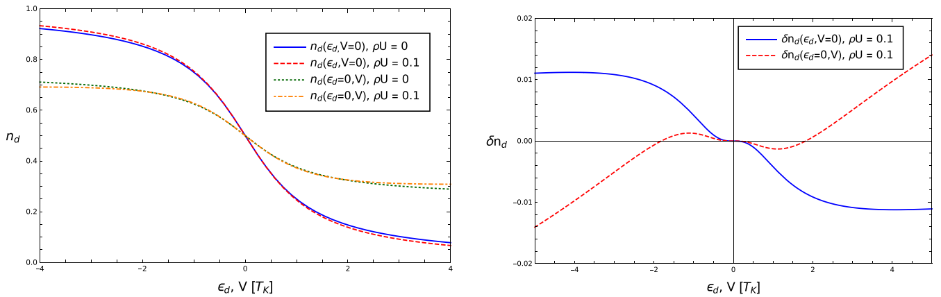
FIG. 1. Left: the steady-state occupancy n_d \equiv \langle n_d \rangle_{\text{s.s.}} at zero temperature in the two-lead IRL, either as a function of dot potential \epsilon_d or voltage V . The leads are held at chemical potentials \mu_1 = 0 and \mu_2 = -V . The equilibrium ( V = 0 ) curves are given by Eq. (3.27) and in fact are independent of the number of leads, in agreement with the Bethe ansatz answer from the literature (Appendix E). The nonequilibrium ( V \neq 0 ) curves are given by Eq. (3.28). In both cases, we compare the noninteracting occupancy ( \rho U = 0 ) with the weakly interacting occupancy (first order in \rho U = 0.1 ), where \rho = 1/(2\pi) is the density of states per unit length. Right: the weakly interacting case with the noninteracting occupancy subtracted, i.e., \delta n_d \equiv n_d - n_d|_{U=0} . In equilibrium, \delta n_d reaches finite limits as \epsilon_d/T_K \rightarrow \pm\infty . Out of equilibrium, |\delta n_d| grows logarithmically as V/T_K \rightarrow \pm\infty , indicating that some resummation of the series in \rho U is needed to make sense of the extremely large voltage regime.
