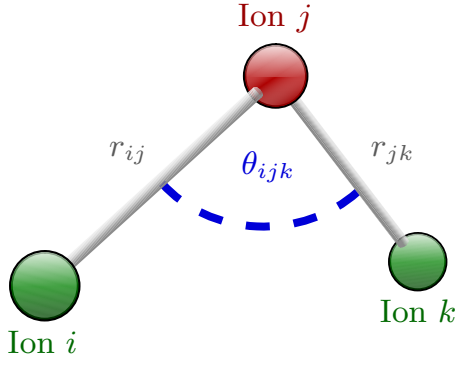
FIG. 1. Schematic of a triplet of ions in the lattice with bond lengths and angles from Eq. (4) marked.
