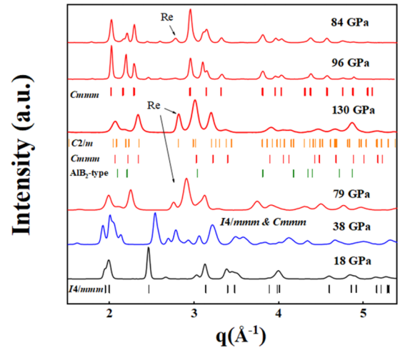
FIG. 3. X-ray diffraction (XRD) patterns measured in the diamond anvil cell experiment of this paper. The data are integrated using DIOPAS [32], and the background is subtracted. The patterns presented by different colors correspond to different phases. The pressure was increased to 130 GPa at room temperature, and then the sample was laser heated. After this, the pressure dropped to 96 GPa, and XRD patterns were measured on the pressure release. Ticks indicate simulated XRD peaks for different phases, and “Re” denotes the diffraction peak of the rhenium gasket.
