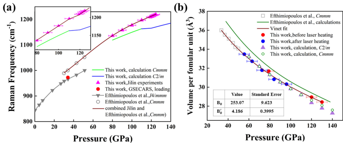
FIG. 5. (a) Frequencies of the measured and calculated Raman modes of BaO 2 as a function of pressure. The solid gray triangles and open gray circles are the data reported in Ref. [15]. Solid green and blue lines are the calculated Raman data of Cmmm and C2/m structures, respectively. Inset shows zoomed-in experimental and theoretical dependencies at high pressures. The error bars in the Jilin experiment are indicated when they are smaller or larger than the size of the symbols, and the error bars on the frequencies are smaller than the size of the symbols. (b) Volume per formula unit for the orthorhombic Cmmm structure of BaO 2 at high pressure range in comparison with those previously obtained at lower pressure condition. The squares and green solid line are the experimental and calculated data reported in Ref. [15]. The hexagons and solid purple triangles are the calculated volumes of Cmmm and C2/m structures, respectively. Red and blue solid circles correspond to data in this paper measured before and after laser heating, respectively. The error bars at each data point are indicated when they are smaller or larger than the size of the symbols. The solid line is the Vinet fit, as given in the text, with B_0 = 253(07) GPa and B'_0 = 4.18(6) and fixed V_0 = 36 \text{ \AA}^3 ( P = 33.6 GPa).
