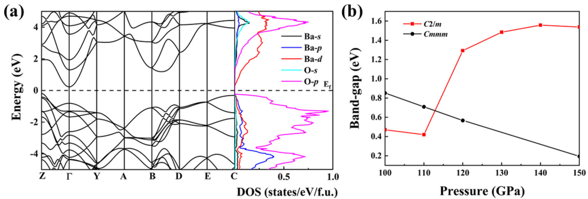
FIG. 6. (a) Electronic band structure (left panel) and projected density of states (right panel) of C2/m structure at 110 GPa. (b) The band gap values of Cmmm and C2/m structures at various pressures.
