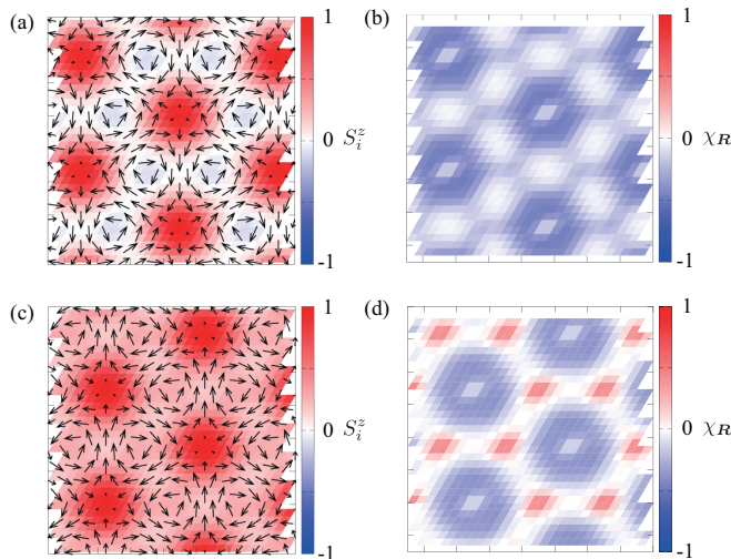
FIG. 50. Real-space spin and chirality configurations of the n_{\text{sk}} = 1 skyrmion crystals at K = 0.1 and I^A = 0.6 . The magnetic field is taken at H^z = 0.5 for panels (a) and (b) and H^z = 1 for panels (c) and (d). In panels (a) and (c), the contour shows the z component of the spin moment, and the arrows represent the xy components. In panels (b) and (d), the contour shows the scalar chirality.
