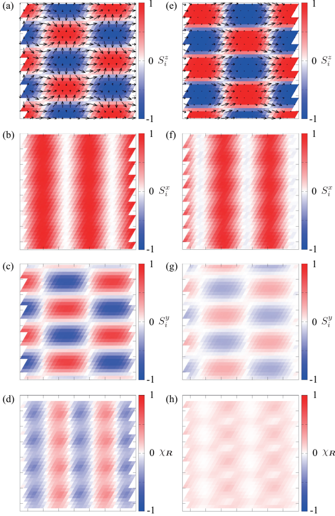
FIG. 20. Real-space spin and chirality configurations of (a)–(d) the anisotropic triple- Q state at H^x = 0.9 and A = 0.2 and (e)–(h) the n_{\text{sk}} = 2 skyrmion crystal at H^x = 0.8 and A = 0.4 . The contour shows the (a), (e) z , (b), (f) x , and (c), (g) y components of the spin moment, and the arrows in panels (a) and (e) represent the xy components. In panels (d) and (h), the contour shows the scalar chirality.
