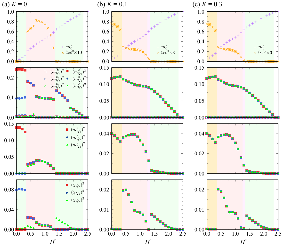
FIG. 41. H^z dependence of (first row) m_0^z and (\chi_0)^2 , (second row) (m_{Q_i}^{Q_j})^2 and (m_{Q_i}^{Q_l})^2 , (third row) (m_{Q_i}^z)^2 , and (fourth row) (\chi_{Q_i})^2 for K = 0 for (a) K = 0 , (b) K = 0.1 , and (c) K = 0.3 at I^A = 0.2 .
