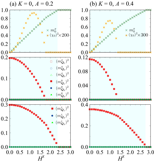
FIG. 16. H^x dependence of (first row) m_0^x and (\chi_0)^2 , (second row) (m_{Q_v}^x)^2 and (m_{Q_v}^y)^2 , and (third row) (m_{Q_v}^z)^2 for K = 0 at (a) A = 0.2 and (b) A = 0.4 .
