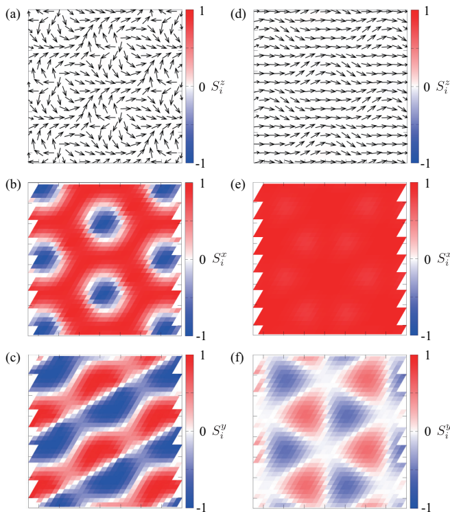
FIG. 25. Real-space spin configurations of (a)–(c) the triple- Q coplanar bubble crystal at K = 0 , A = -0.3 , and H^x = 1 and (d)–(e) the triple- Q coplanar fan state at K = 0.3 , A = -0.1 , and H^x = 1.8 . The contour shows the (a), (d) z , (b), (e) x , and (c), (f) y components of the spin moment, and the arrows in panels (a) and (d) represent the xy components.
