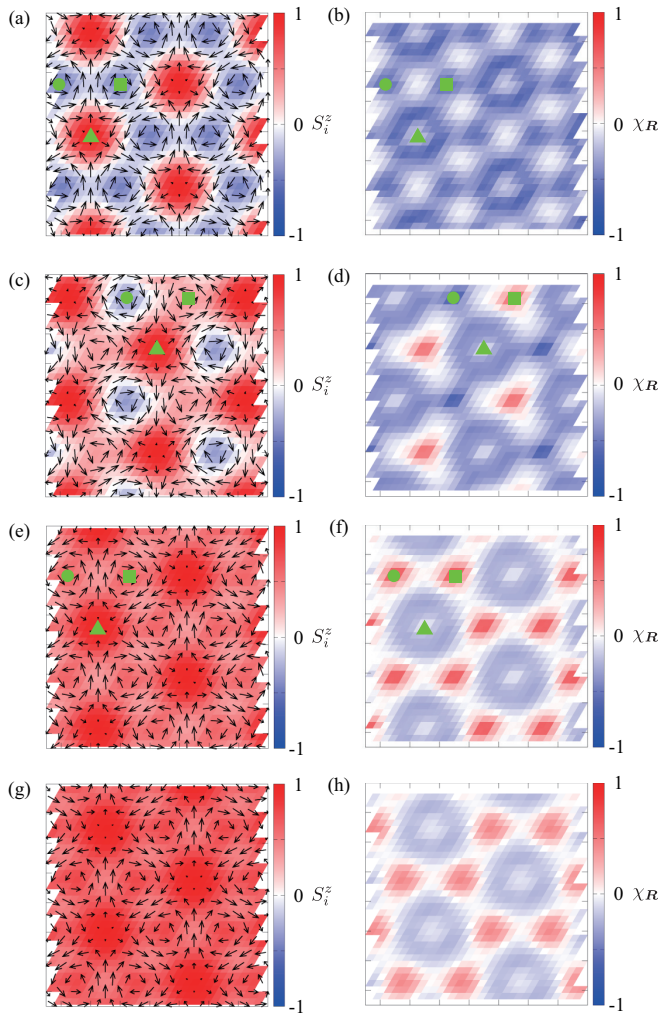
FIG. 48. Real-space spin and chirality configurations at K = 0.3 and I^A = 0.4 . The magnetic field is taken at H^z = 0.1 for (a), (b) the n_{\text{sk}} = 2 skyrmion crystal, H^z = 0.6 for (c), (d) the n_{\text{sk}} = 1 skyrmion crystal, H^z = 1.3 for (e), (f) the triple- Q state with nonzero (\chi_0)^2 , and H^z = 1.6 for (g), (h) the triple- Q state without (\chi_0)^2 . In panels (a), (c), (e), and (g), the contour shows the z component of the spin moment, and the arrows represent the xy components. In panels (b), (d), (f), and (h), the contour shows the scalar chirality. In panels (a)–(f), the green squares and circles represent the cores of the type I and II vortices with vorticity +1 , respectively, whereas the green triangles represent the cores of the vortices with vorticity -2 . See the main text in the details.
