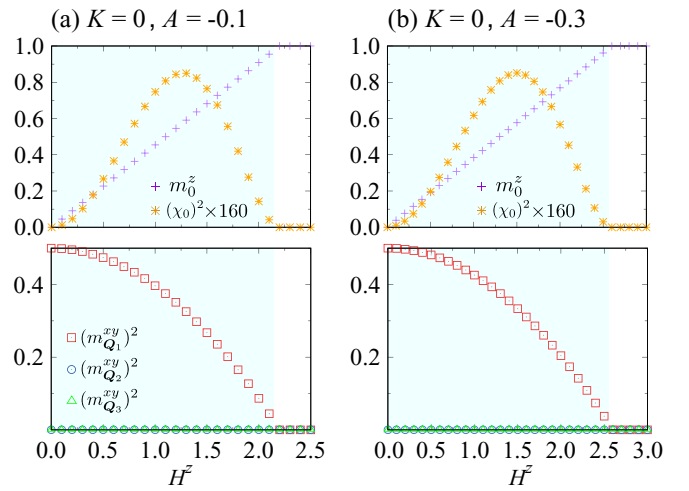
FIG. 11. H^z dependence of (upper) m_0^z and (\chi_0)^2 and (lower) (m_{Q_v}^{xy})^2 for K = 0 at (a) A = -0.1 and (b) A = -0.3 .
