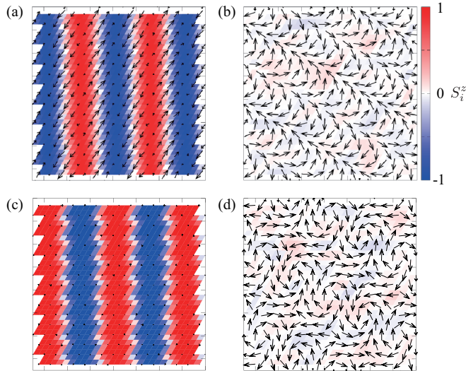
FIG. 3. Real-space spin configurations of (a) the single- Q (1 Q ) helical state at A = 0.2 and K = 0 , (b) the 1 Q cycloidal state at A = -0.4 and K = 0 , (c) the 1 Q collinear state at A = 0.6 and K = 0 , and (d) the double- Q (2 Q ) coplanar state at A = -0.4 and K = 0.3 . The contour shows the z component of the spin moment [144], and the arrows represent the xy components.
