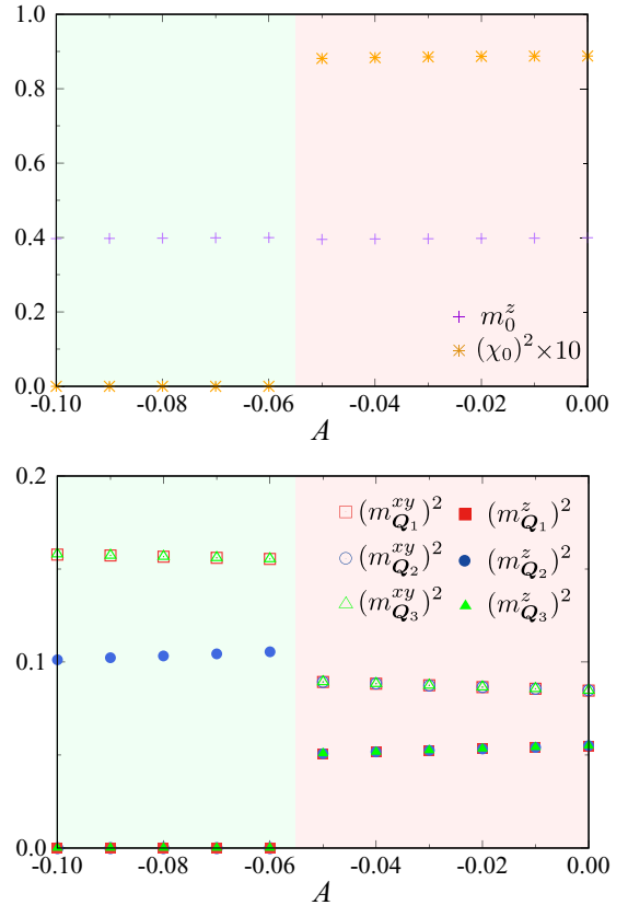
FIG. 15. A dependence of (upper) m_0^z and (\chi_0)^2 and (lower) (m_{\mathbf{Q}_v}^{xy})^2 and (m_{\mathbf{Q}_v}^z)^2 at K = 0.3 and H^z = 0.7 .
