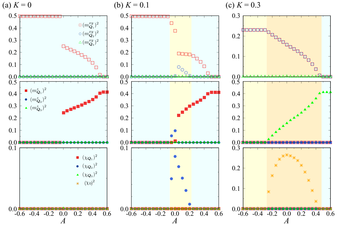
FIG. 5. A dependence of (first row) (m_{Q_i}^{xy})^2 , (second row) (m_{Q_i}^z)^2 , and (third row) (\chi_{Q_i})^2 and (\chi_0)^2 for (a) K = 0 , (b) K = 0.1 , and (c) K = 0.3 . See also Fig. 2.
