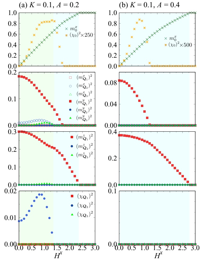
FIG. 17. H^x dependence of (first row) m_0^x and (\chi_0)^2 , (second row) (m_{Q_v}^x)^2 and (m_{Q_v}^y)^2 , (third row) (m_{Q_v}^z)^2 , and (fourth row) (\chi_{Q_v})^2 for K = 0.1 at (a) A = 0.2 and (b) A = 0.4 .
