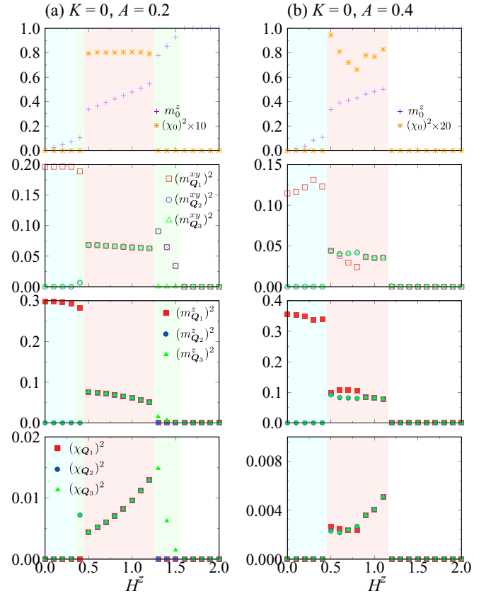
FIG. 8. H^z dependence of (first row) m_0^z and (\chi_0)^2 , (second row) (m_{Q_v}^{xy})^2 , (third row) (m_{Q_v}^z)^2 , and (fourth row) (\chi_{Q_v})^2 for K = 0 at (a) A = 0.2 and (b) A = 0.4 .
