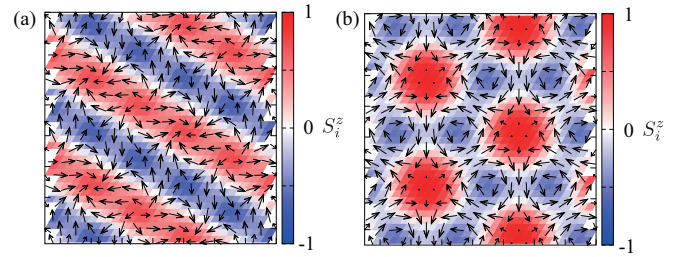
FIG. 14. Real-space spin configuration of the n_{\text{sk}} = 2 skyrmion crystals at (a) H^z = 0.1 and (b) H^z = 0.2 . The contour shows the z component of the spin moment, and the arrows represent the xy components.
