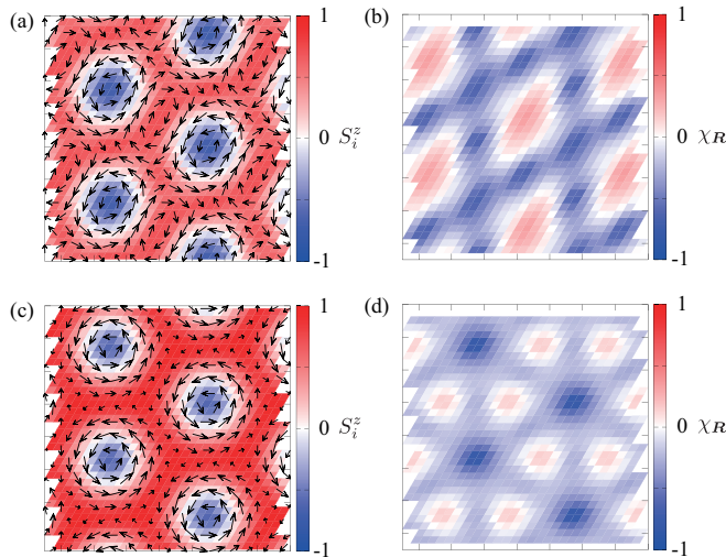
FIG. 42. Real-space spin and chirality configurations of the n_{\text{sk}} = 1 skyrmion crystals at K = 0 and I^A = 0.2 . The magnetic field is taken at H^z = 0.5 for panels (a) and (b) and at H^z = 1 for panels (c) and (d). In panels (a) and (c), the contour shows the z component of the spin moment, and the arrows represent the xy components. In panels (b) and (d), the contour shows the scalar chirality.
