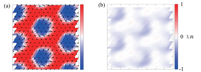
FIG. 31. Real-space spin and chirality configurations of the triple- Q state with nonzero (\chi_0)^2 at \theta = 58.5^\circ for K = 0.3 and A = 0.4 . The contour shows panel (a) the z component of the spin moment, and the arrows represent the xy components. In panel (b), the contour shows the scalar chirality.
