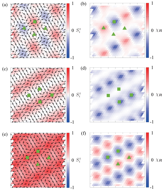
FIG. 47. Real-space spin and chirality configurations at K = 0 and I^A = 0.4 . The magnetic field is taken at H^z = 0.1 for (a), (b) the n_{\text{sk}} = 1 meron crystal, H^z = 0.3 for (c), (d) the n_{\text{sk}} = 2 meron crystal, and H^z = 1.2 for (e), (f) the anisotropic triple- Q state. In panels (a), (c), and (e), the contour shows the z component of the spin moment, and the arrows represent the xy components. In panels (b), (d), and (f), the contour shows the scalar chirality. The green triangles and squares represent the cores with the positive and negative skyrmion numbers, respectively.
