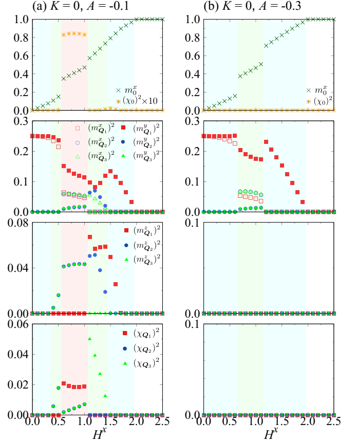
FIG. 21. H^x dependence of (first row) m_0^x and (\chi_0)^2 , (second row) (m_{Q_v}^x)^2 and (m_{Q_v}^y)^2 , (third row) (m_{Q_v}^z)^2 , and (fourth row) (\chi_{Q_v})^2 for K = 0 at (a) A = -0.1 and (b) A = -0.3 .
