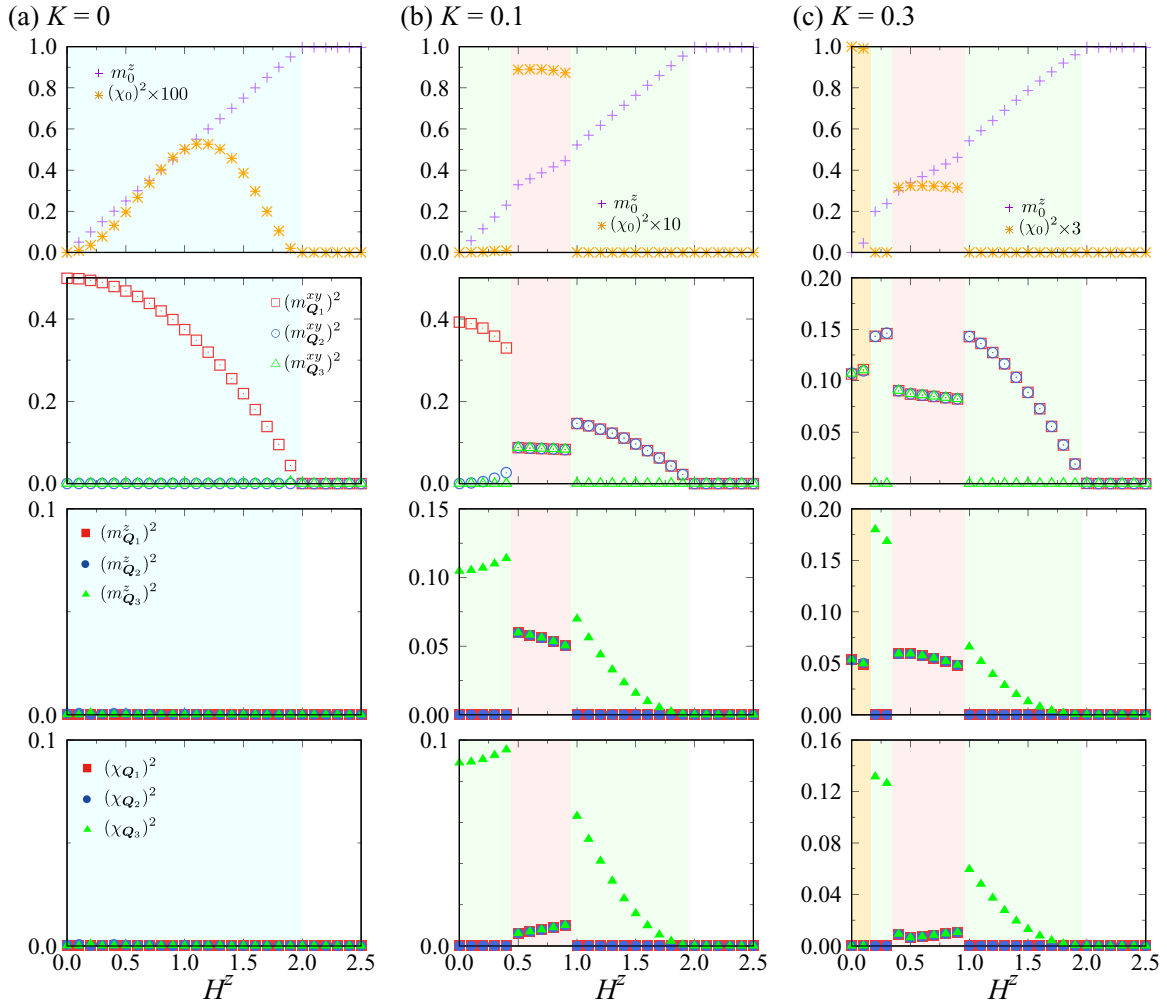
FIG. 6. H^z dependence of (first row) m_0^z and (\chi_0)^2 , (second row) (m_{Q_v}^{xy})^2 , (third row) (m_{Q_v}^z)^2 , and (fourth row) (\chi_{Q_v})^2 for (a) K = 0 , (b) K = 0.1 , and (c) K = 0.3 at A = 0 .
