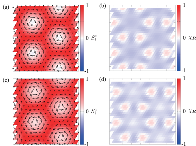
FIG. 43. Real-space spin and chirality configurations of the (a), (b) n_{\text{sk}} = 1 skyrmion crystal at K = 0 and (c), (d) the triple- Q crystal at K = 0.1 for I^A = 0.2 and H^z = 1.3 . In panels (a) and (c), the contour shows the z component of the spin moment, and the arrows represent the xy components. In panels (b) and (d), the contour shows the scalar chirality.
