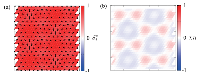
FIG. 45. Real-space spin and chirality configurations of the isotropic triple- Q state at K = 0 , I^A = 0.2 , and H^z = 2 . In panel (a), the contour shows the z component of the spin moment, and the arrows represent the xy components. In panel (b), the contour shows the scalar chirality.
