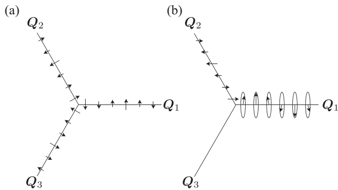
FIG. 40. Schematic pictures of (a) three sinusoidal waves consisting the n_{\text{sk}} = 2 skyrmion crystal and (b) the single- Q helical and single- Q sinusoidal waves consisting of the double- Q chiral stripe state in Fig. 36 for I^A > 0 at zero field. See also Figs. 37(a), 37(b), 37(e), and 37(f).
