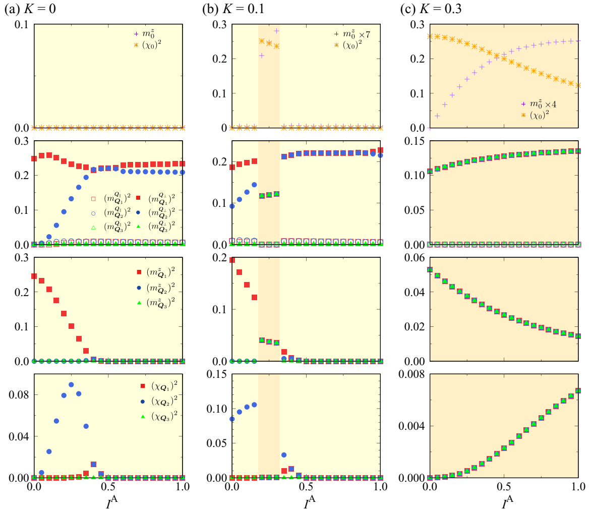
FIG. 39. I^A dependence of (first row) m_0^z and (\chi_0)^2 , (second row) (m_{Q_1}^Q)^2 and (m_{Q_2}^Q)^2 , (third row) (m_{Q_1}^z)^2 , and (fourth row) (\chi_{Q_i})^2 for (a) K = 0 , (b) K = 0.1 , and (c) K = 0.3 in the absence of the magnetic field.
