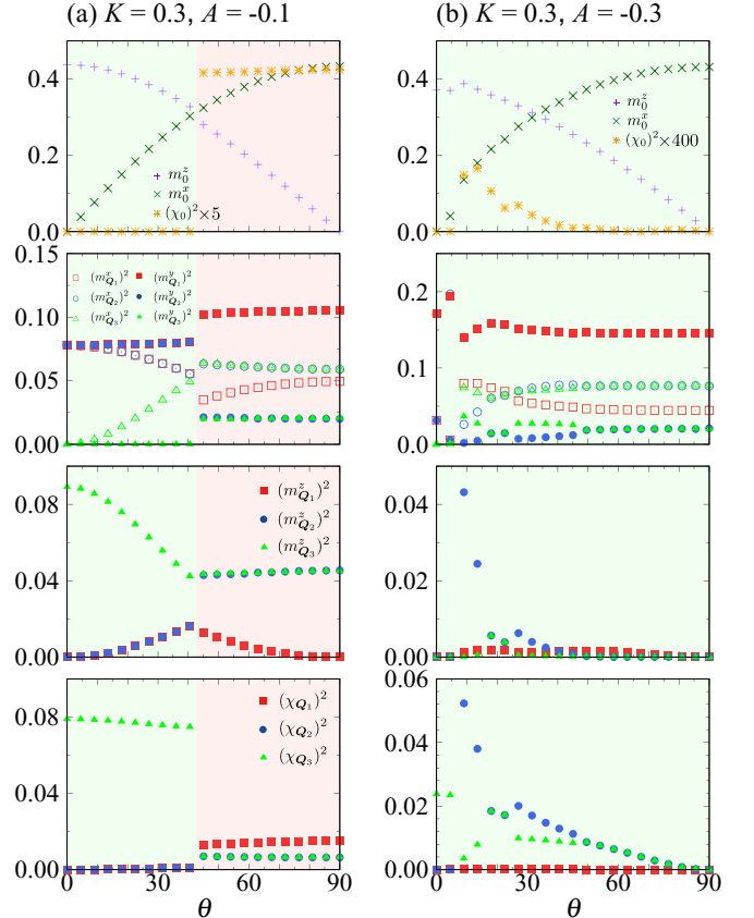
FIG. 35. The same plots as in Fig. 33 for K = 0.3 .
