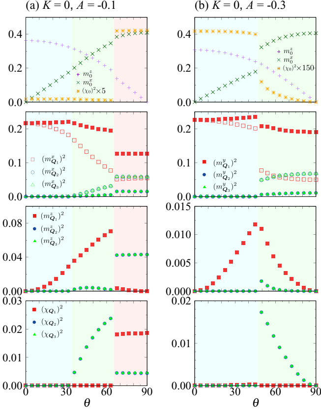
FIG. 33. \theta dependence of (first row) m_0^z , m_0^x , and (\chi_0)^2 , (second row) (m_{Q_1}^x)^2 and (m_{Q_2}^y)^2 , (third row) (m_{Q_1}^z)^2 , and (fourth row) (\chi_{Q_1})^2 for K = 0 at (a) A = -0.1 and (b) A = -0.3 . The magnitude of the magnetic field is fixed at H = 0.8 .
