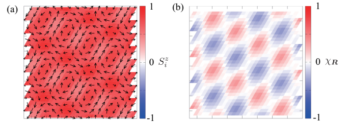
FIG. 44. Real-space spin and chirality configurations of the anisotropic triple- Q state at K = 0 , I^A = 0.2 , and H^z = 1.5 . In panel (a), the contour shows the z component of the spin moment, and the arrows represent the xy components. In panel (b), the contour shows the scalar chirality.
