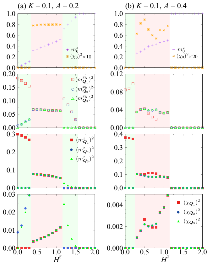
FIG. 9. The same plots as in Fig. 8 for K = 0.1 .
