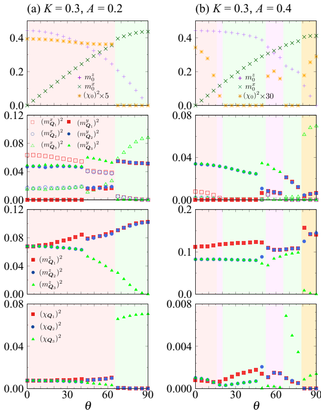
FIG. 28. The same plots as in Fig. 26 for K = 0.3 .
