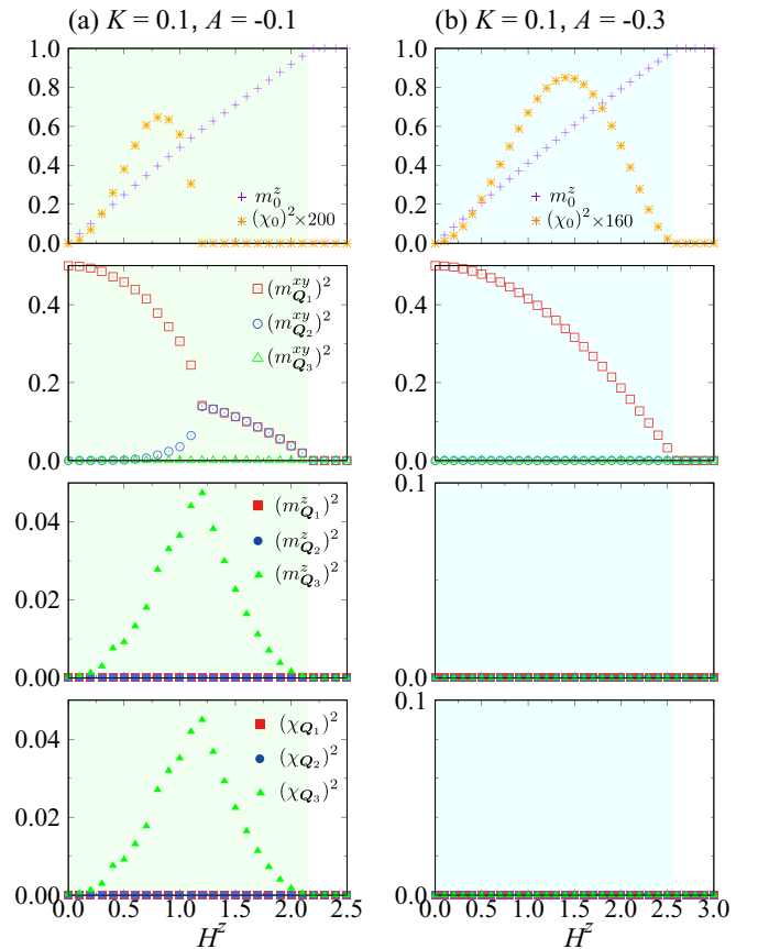
FIG. 12. H^z dependence of (first row) m_0^z and (\chi_0)^2 , (second row) (m_{Q_v}^{xy})^2 , (third row) (m_{Q_v}^z)^2 , and (fourth row) (\chi_{Q_v})^2 for K = 0.1 at (a) A = -0.1 and (b) A = -0.3 .
