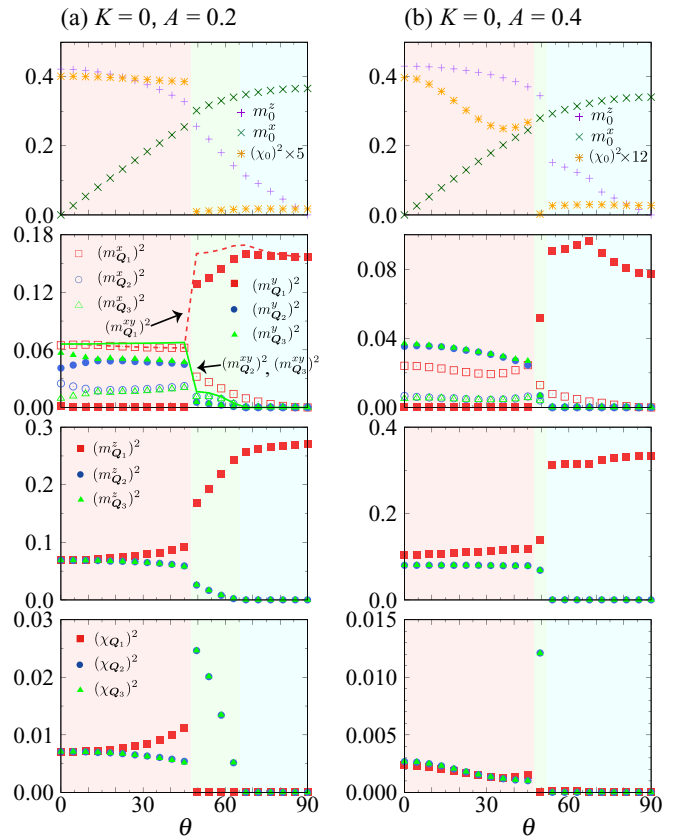
FIG. 26. \theta dependence of (first row) m_0^z , m_0^x , and (\chi_0)^2 , (second row) (m_{Q_v}^x)^2 and (m_{Q_v}^y)^2 , (third row) (m_{Q_v}^z)^2 , and (fourth row) (\chi_{Q_v})^2 for K = 0 at (a) A = 0.2 and (b) A = 0.4 . In the second row in panel (a), the dashed line represents (m_{Q_1}^{xy})^2 , while the solid lines represent (m_{Q_2}^{xy})^2 and (m_{Q_3}^{xy})^2 . The magnitude of the magnetic field is fixed at H = 0.8 .
