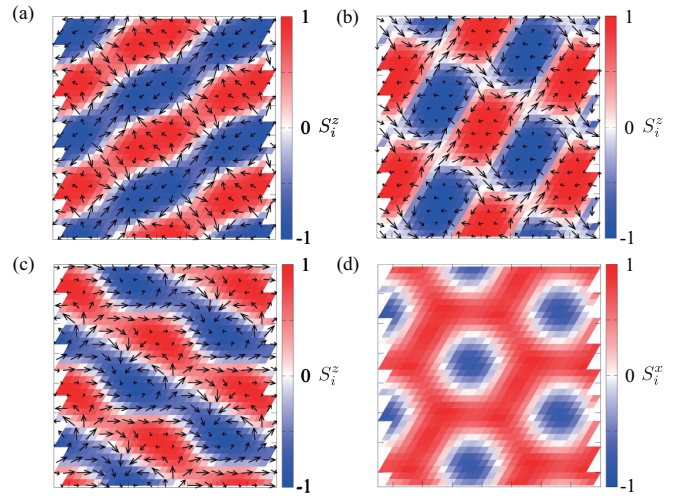
FIG. 19. Real-space spin configuration of the n_{\text{sk}} = 2 skyrmion crystals at (a) H^x = 0.1 and (b) H^x = 0.3 , and (c), (d) the n_{\text{sk}} = 2 skyrmion crystal at H^x = 0.5 for K = 0.3 and A = 0.2 . In panels (a)–(c), the contour shows the z component of the spin moment, and the arrows represent the xy components. In panel (d), the contour shows the x component of the spin moment.
