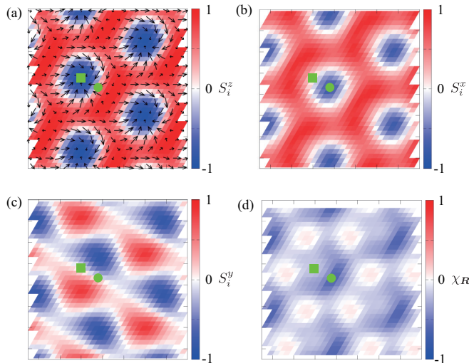
FIG. 30. Real-space spin and chirality configurations of the n_{\text{sk}} = 1 skyrmion crystal at \theta = 63^\circ for K = 0.3 and A = 0.2 . The contour shows the (a) z , (b) x , and (c) y components of the spin moment, and the arrows in panel (a) represent the xy components. In panel (d), the contour shows the scalar chirality. The green squares and circles represent the positions of the minima of S^z and S^x , respectively.
