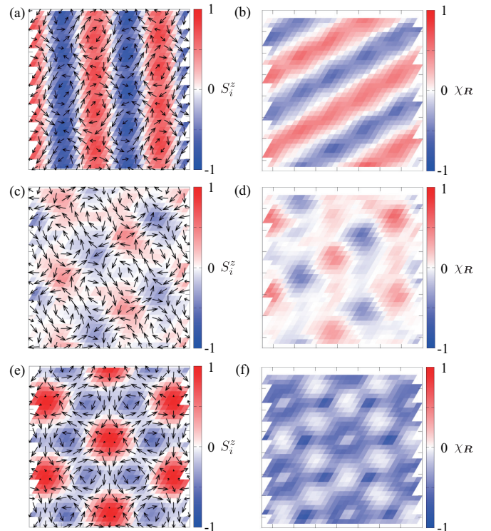
FIG. 37. Real-space spin configurations of (a) the double- Q ( 2Q ) chiral stripe state at K = 0.1 and I^A = 0.1 , (c) the 2Q helical state at K = 0.1 and I^A = 0.4 , and (e) the n_{\text{sk}} = 2 skyrmion crystal at K = 0.3 and I^A = 0.5 . The contour shows the z component of the spin moment, and the arrows represent the xy components. Panels (b), (d), and (f) display the real-space chirality configurations corresponding to panels (a), (c), and (e), respectively.
