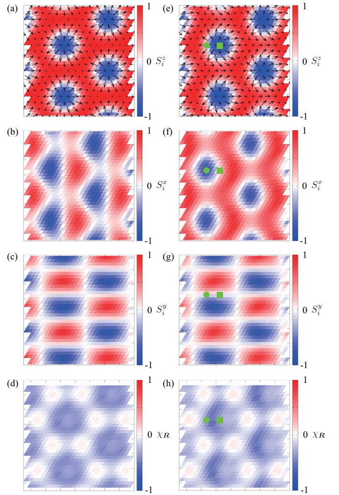
FIG. 29. Real-space spin and chirality configurations of the n_{\text{sk}} = 1 skyrmion crystals at (a)–(d) \theta = 5^\circ and (e)–(h) \theta = 45^\circ for K = 0 and A = 0.2 . The contour shows the (a), (e) z , (b), (f) x , and (c), (g) y components of the spin moment, and the arrows in panels (a) and (e) represent the xy components. In panels (d) and (h), the contour shows the scalar chirality. In panels (e)–(h), the green squares and circles represent the positions of the minima of S^z and S^x , respectively.
