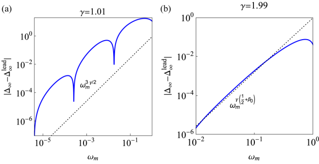
FIG. 26. The expansion of the exact \Delta_\infty(\omega_m) in powers of \omega_m . The leading term at small \omega_m is \Delta_\infty^{\text{lead}}|\omega_m|^{\gamma/2} = \cos(\beta\gamma \log|\omega_m|/\bar{g} + \phi) . The subleading terms form series of local and nonlocal terms. Local series hold in powers of |\omega_m|^{n\gamma} ( n = 1, 2, \dots ), and all terms in these series oscillate, like the leading term. The nonlocal terms do not oscillate and form series in |\omega_m|^{(n'+\beta_m)\gamma} , where n' = (0, 1, 2, \dots) and \beta_m ( m = 0, 1, 2, \dots ) are some \gamma -dependent numbers. We show |\Delta^\infty - \Delta_\infty^{\text{lead}}| for \gamma = 1.01 and \gamma = 1.99 . An analytical analysis shows that in the first case, \beta_0 > 1 , such that the leading correction comes from the local series and oscillates. For \gamma = 1.99 , \beta_0 \simeq 0.9 < 1 . In this case the leading correction comes from nonlocal series and does not oscillate. The numerical evaluation of |\Delta^\infty - \Delta_\infty^{\text{lead}}| shown here confirms these results.
