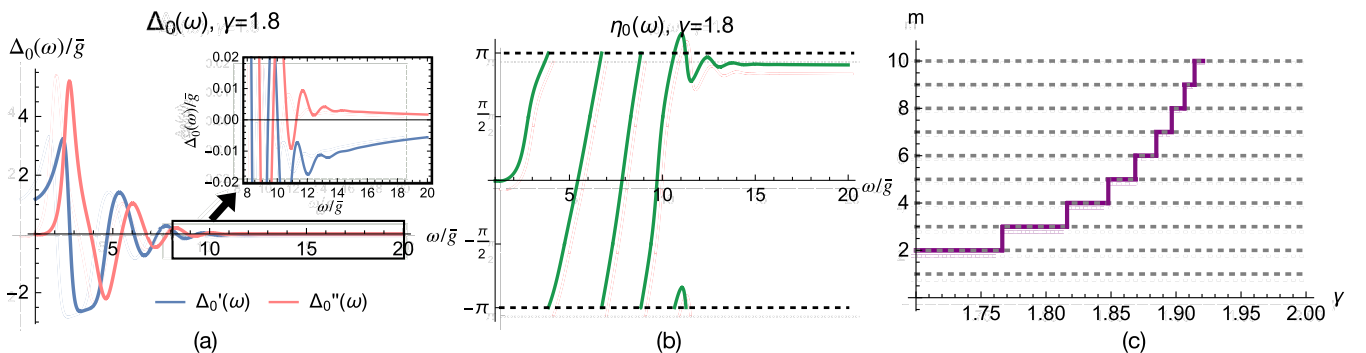
FIG. 17. (a), (b) The same as in Fig. 15, but for \phi' and \phi'' from Eq.(69). At large frequencies, \Delta(\omega) \propto e^{i\pi\gamma/2}/\omega^\gamma . The total variation of the phase of \Delta is \delta\eta = 2\pi m + \pi\gamma/2 . (c) Variation of m with \gamma . As before, there is a discrete set of \gamma_i , where m jumps by 1. The set becomes progressively more dense at \gamma \rightarrow 2 .
