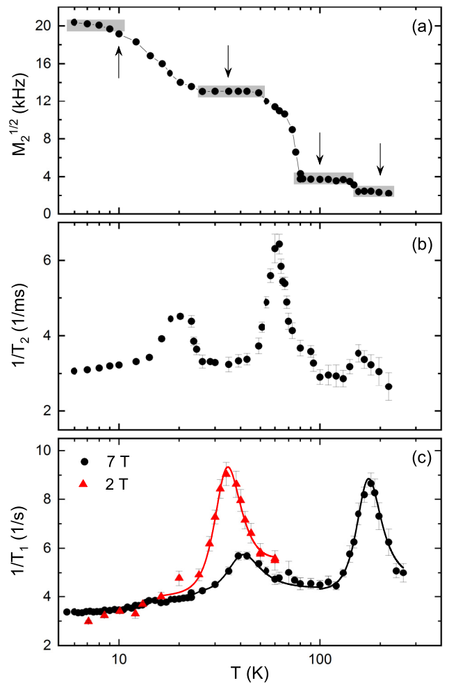
FIG. 3. (a) Temperature dependence of the square root of the ^{31}\text{P} second spectral moment at 7 T. The vertical arrows indicate the temperatures at which the angular-dependent ^{31}\text{P} NMR spectra were recorded, see Figs. 4 and 5. (b) Temperature dependence of the ^{31}\text{P} nuclear spin-spin relaxation rate at 7 T. (c) Temperature dependence of the ^{31}\text{P} nuclear spin-lattice relaxation rate at 7 and 2 T. The black (red) lines represent fits with the BPP model to the 7 T (2 T) data.
