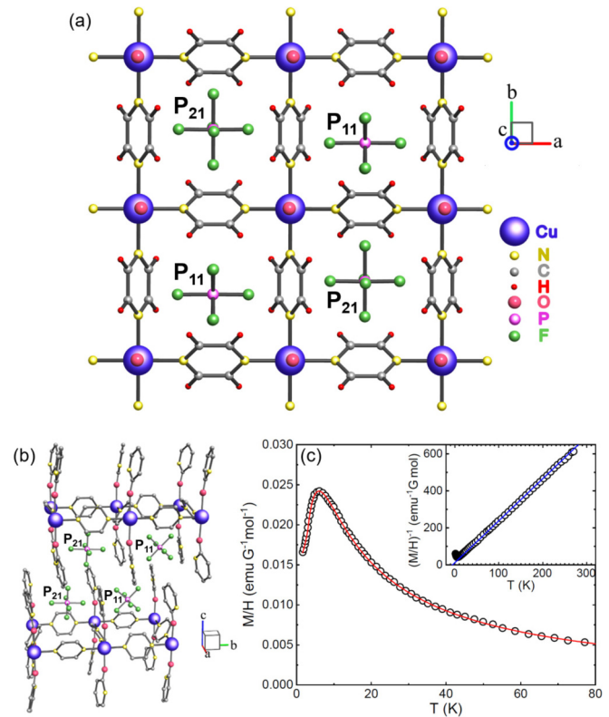
FIG. 1. (a) In CuPOF, quasi-2D planes of \text{Cu}^{2+} ions are linked by pyrazine molecules, forming the motif of a magnetic square lattice. Two structurally slightly inequivalent \text{PF}_6 molecules are located in-between the layers. (b) View on two adjacent Cu-pyrazine layers, with hydrogen atoms omitted for clarity. (c) Temperature dependence of the static susceptibility (circles). The red line shows the best fit of 2D QHAF model calculations to the magnetic susceptibility of a polycrystalline sample [27]. The inset of (c) shows the temperature dependence of the inverse static susceptibility. The blue line denotes the best fit with a Curie-Weiss behavior.
