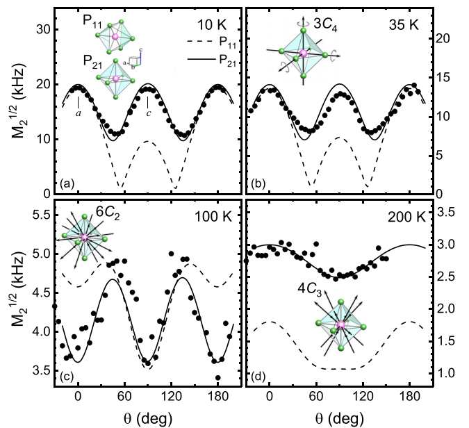
FIG. 5. Angular dependence (with H \parallel a or \parallel c corresponding to \theta = 0 or 90 degrees, respectively) of square root of the ^{31}\text{P} second spectral moment at (a) 10, (b) 35, (c) 100, and (d) 200 K, compared to calculations for the nuclear \text{P}_{11} and \text{P}_{21} sites for (a) a rigid lattice and in the presence of \text{PF}_6 molecular reorientations around the symmetry axes (b) 3C_4 , (c) 6C_2 , and (d) 4C_3 . The inset in (a) shows a sketch of the local \text{P}_{11} and \text{P}_{21} symmetry with respect to the in-plane ( H \parallel a , horizontal) and out-of-plane ( H \parallel c , vertical) field orientation. The insets in (b), (c), and (d) show sketches of the molecular symmetry axes, around which the \text{PF}_6 molecular reorientations occur.
