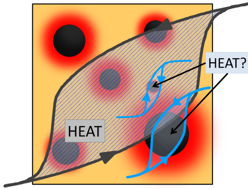
FIG. 1. Illustration of global vs local heat in a nanoparticle ensemble: do individual (single-particle) loops represent local heating?
