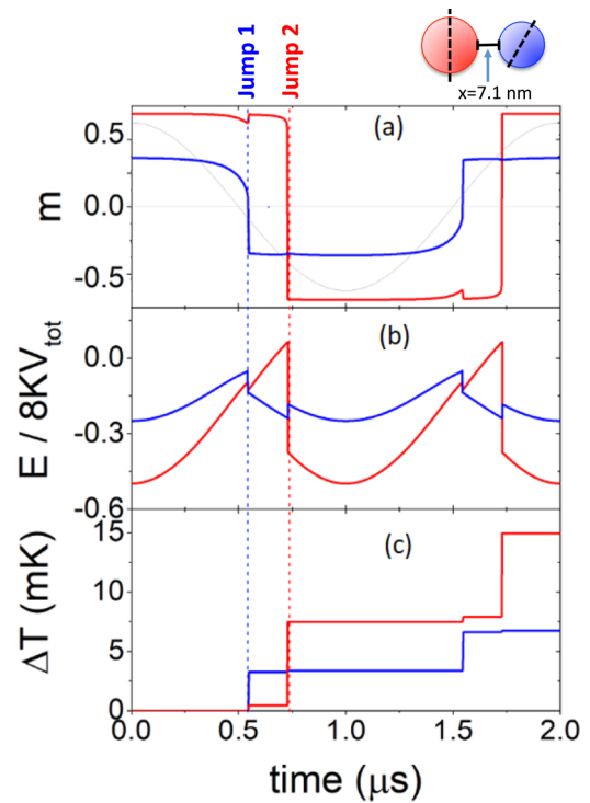
FIG. 3. Dynamics of (a) normalized magnetization, (b) total energy (normalized by the maximum possible stored energy 2M_s 2H_K V_{\text{tot}} = 8KV_{\text{tot}} , where V_{\text{tot}} is the system volume and H_K = 2K/M_s is the anisotropy field), and (c) temperature change \Delta T as computed by Eq. (1). The blue line corresponds to nanoparticle B and the red line to nanoparticle A. The nanoparticles are separated by x = 7.1 nm.
