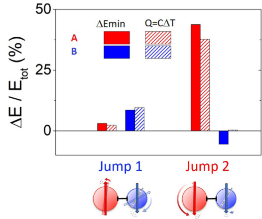
FIG. 4. A comparison of energy change (work plus heat, solid bars) and heat released (hashed bars) during the two irreversible magnetization jumps for the two particles A (red) and B (blue). The energy changes \Delta E_{\text{min}} are evaluated from individual hysteresis loops, while the heat released Q is calculated using Eq. (1) with large damping \alpha_{\perp} = 1.0 . The results are normalized to the total energy “stored” in the global hysteresis loop. The nanoparticles are separated by 7.1 nm, as in Fig. 3. The sketches illustrate whether the magnetization of the particle switches, or wobbles, within the same energy well.
