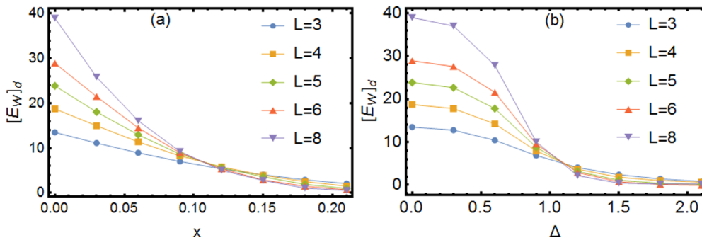
FIG. 9. Domain-wall energy [E_W]_d for the (a) binary and (b) Gaussian phase-glass models in the limit g \rightarrow 0 for increasing disorder ( x or \Delta ) and different systems sizes L . The common crossing point of the curves gives an estimate of the chiral-glass disorder threshold x_C and \Delta_C in the phase diagrams of Fig. 1.
