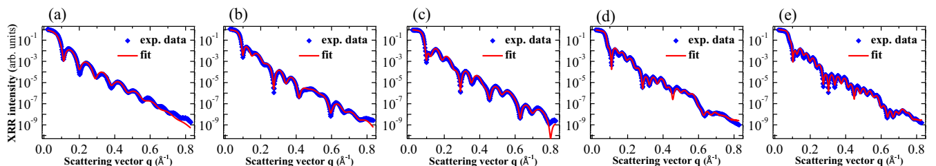
FIG. 2. (a)–(e) The off-resonant (11 467 eV) averaged XRR signals with fits for all the multilayers.
