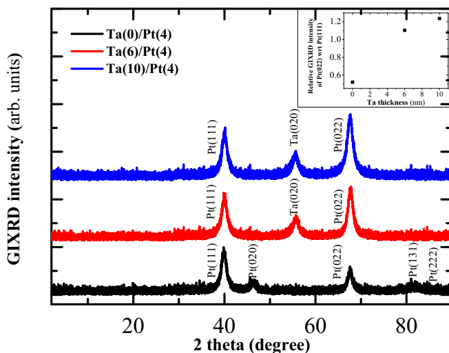
FIG. 7. Grazing incidence x-ray diffraction data with an incidence angle of 0.5^\circ of Ta( t )/Pt(4 nm) bilayers with t = 0, 6, and 10 nm. Data have been vertically shifted with an offset for a better view. The inset shows the relative intensity ratio of Pt(022) with respect to Pt(111).
