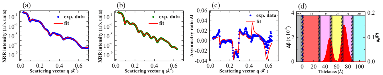
FIG. 6. (a) The off-resonant (11 467 eV) averaged XRR signals with fits; (b) the resonant (11 567 eV) averaged XRR signals with fits; (c) the corresponding measured and fitted XRMR asymmetry ratio \Delta I(q) for the Ta(3)/Pt(2)/Co(2)/Pt(2) multilayer; (d) magneto-optic depth profile, which was used to fit the XRMR asymmetry ratio. Red histograms depict the in-depth distribution of the spin-polarized Pt atoms. The induced magnetic moment per Pt atom has been quantified from ab initio calculation. The dashed lines denote the corresponding interface position between the layers, whereas the dashed rectangles between the layers denote the corresponding interlayer roughness.
