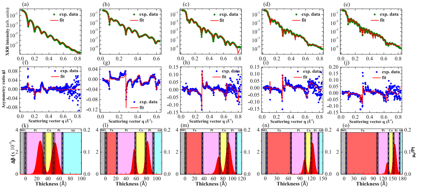
FIG. 3. (a)–(e) The resonant (11 567 eV) averaged XRR signals with fits. (f)–(j) The corresponding measured and fitted XRRM asymmetry ratios \Delta I(q) for the multilayers. (k)–(o) Magneto-optic depth profiles, which were used to fit the XRRM asymmetry ratios. Red histograms depict the in-depth distribution of the spin-polarized Pt atoms. The induced magnetic moment per Pt atom has been quantified from ab initio calculation. The dashed lines denote the corresponding interface position between the layers, whereas the dashed rectangles between the layers denote the corresponding interlayer roughness.
