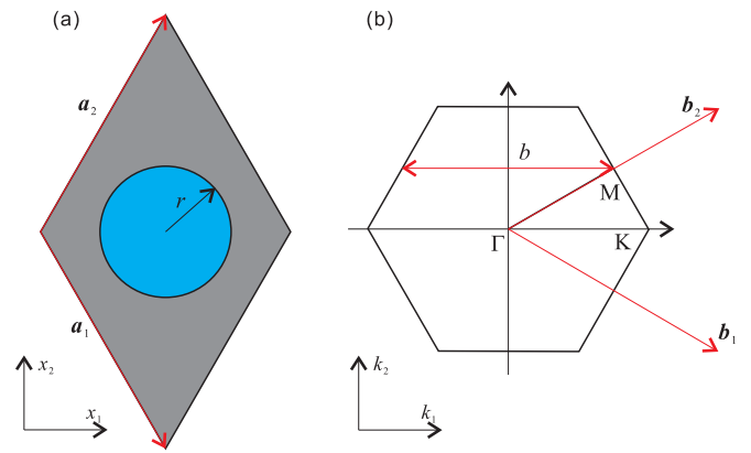
FIG. 1. (a) Primitive unit cell for two-dimensional hexagonal phononic crystals composed of solid cylindrical rods embedded in a fluid matrix. Lattice vectors are represented by the red vectors, with \mathbf{a}_1 = a(\mathbf{i} - \sqrt{3}\mathbf{j})/2 and \mathbf{a}_2 = a(\mathbf{i} + \sqrt{3}\mathbf{j})/2 . (b) The first Brillouin zone is also hexagonal. High-symmetry points \Gamma , K , and M are indicated. \mathbf{b}_1 = b(\mathbf{i} - \sqrt{3}/3\mathbf{j}) and \mathbf{b}_2 = b(\mathbf{i} + \sqrt{3}/3\mathbf{j}) with b = 2\pi/a .
