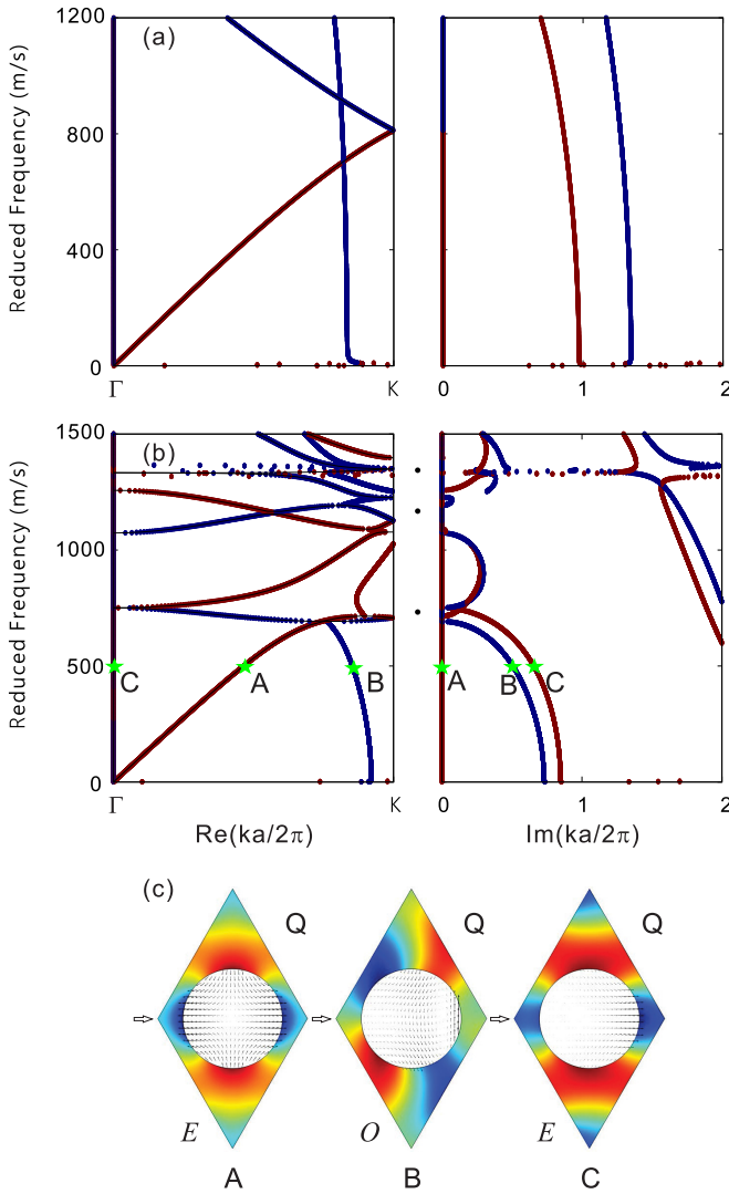
FIG. 6. Complex band structure of the two-dimensional hexagonal phononic crystal in the \Gamma K direction for (a) steel in water and (b) nylon in water. In either case, the left and right panels show the variation of reduced frequency versus the real or imaginary part of the wave vector, respectively. The solid lines are for the classical band structure. Even-symmetric Bloch waves appear in red; odd-symmetric Bloch waves appear in blue. The black points in between the panels of (b) mark the resonant frequencies for nylon in water. (c) Modal field patterns (periodic part only) are displayed at points A, B, and C. The thick arrows indicate the direction of propagation of Bloch waves.
