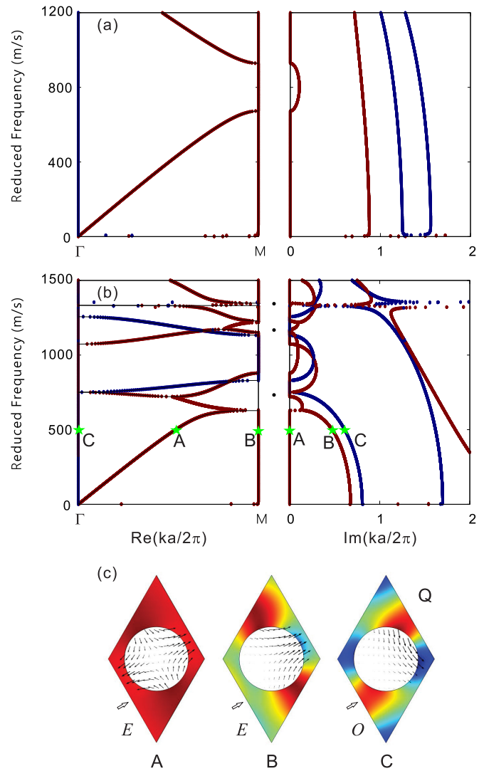
FIG. 5. Complex band structure of the two-dimensional hexagonal phononic crystal in the \Gamma M direction for (a) steel in water and (b) nylon in water. In either case, the left and right panels show the variation of reduced frequency versus the real or imaginary part of the wave vector, respectively. The solid lines are for the classical band structure. Even-symmetric Bloch waves appear in red; odd-symmetric Bloch waves appear in blue. The black points in between the panels of (b) mark the resonant frequencies for nylon in water. (c) Modal field patterns (periodic part only) are displayed at points A, B, and C. The thick arrows indicate the direction of propagation of Bloch waves.
