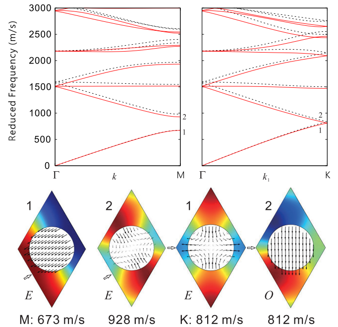
FIG. 2. Phononic band structure for a two-dimensional hexagonal phononic crystal of steel rods in water, accounting for acoustoelastic coupling. Dashed lines are for the simplified fluid-fluid case, with shear waves in the solid neglected. The first two Bloch waves at the M and K points of the first Brillouin zone are presented below the band structure. The color scale represents the pressure in water, from negative (blue) to positive (red) amplitudes. The thin arrows represent the displacement vector in the solid inclusion. The thick arrow indicates the direction of propagation of Bloch waves. The two Bloch waves at the K point are degenerate in frequency.
