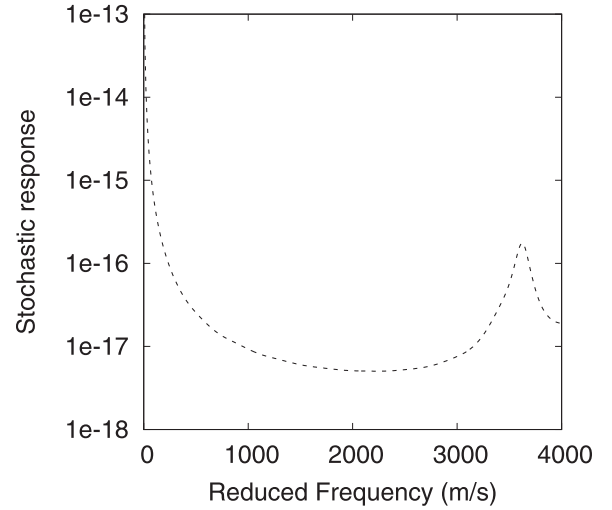
FIG. 7. Stochastic response of a single steel rod in water. The plot shows the total elastic energy as a function of the forcing reduced frequency \omega a/(2\pi) , with the lattice constant a having the same value as for the phononic crystal.
