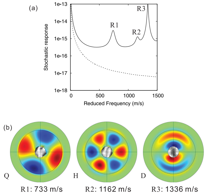
FIG. 4. (a) Stochastic response of a single nylon (solid line) or steel (dashed line) rod in water. The plot shows the total elastic energy as a function of the forcing reduced frequency \omega a/(2\pi) , with the lattice constant a having the same value as for the phononic crystal. (b) The resonant modes at the three resonant peaks are shown for the nylon rod. The color scale represents the pressure from negative (blue) to positive (red) maximum amplitude. The thin arrows indicate the displacement vectors. The external annular domain is the perfectly matched layer (see text). Modal symmetry is either quadrupolar (Q), hexapolar (H), or dipolar (D).
