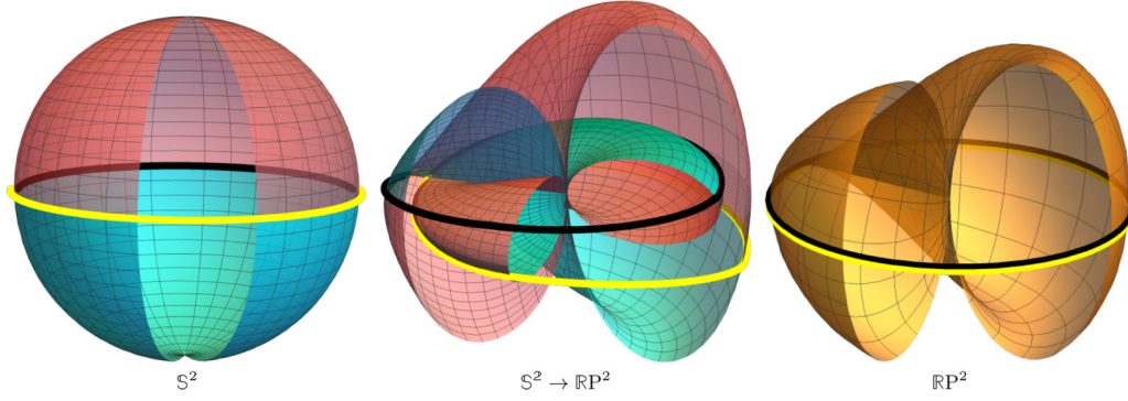
FIG. 2. Orientable double cover \mathbb{S}^2 \rightarrow \mathbb{RP}^2 obtained through the folding of the sphere onto itself. It is dictated by the twisted folding of the equator, i.e., we form the shape “8” and fold the black loop onto the yellow loop. This results in identifying every antipodal pair of points of the sphere to a single point of the projective plane \mathbb{RP}^2 .
