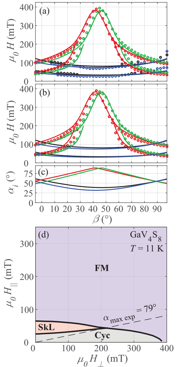
FIG. 4. Magnetic phase transitions measured in GaV 4 S 8 at T = 11 K. Features extracted from DCM measurement of (a) \Delta f(H) and (b) \Gamma(H) are plotted as open circles as a function of \beta . Black, red, green, and blue circles correspond to domains P_1 , P_2 , P_3 , and P_4 , respectively. Color-coded lines indicate phase boundaries for each domain according to the phase diagram in (d). (c) Angle \alpha_i between the corresponding \hat{\mathbf{c}}_i and the external field \mathbf{H} vs \beta for all four rhombohedral domains, using the same color code as in (a) and (b). (d) Best-fit magnetic phase diagram for single-domain GaV 4 S 8 as a function of field applied perpendicular and parallel to the axis of symmetry.
