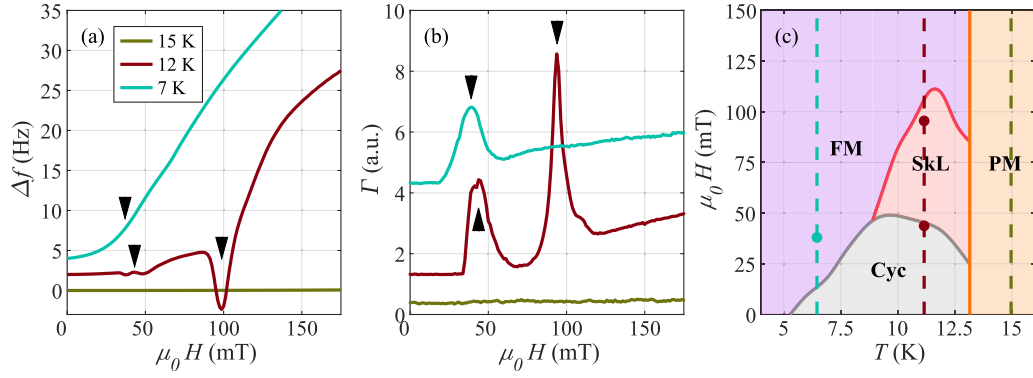
FIG. 2. Temperature and field dependence of magnetic phase transitions measured by DCM in \text{GaV}_4\text{S}_8 . DCM measurements of (a) \Delta f(H) and (b) \Gamma(H) taken at T = 7, 12, and 15 K in cyan, maroon, and brown, respectively. Curves are shifted for better visibility. \beta = 0 , i.e., approximately \mathbf{H} \parallel [100] . Arrows indicate features corresponding to phase transitions. (c) Sketch of the expected magnetic phase diagram as a function of temperature and applied field for \mathbf{H} \parallel [100] [17]. Color-coded dashed lines and points correspond to temperatures and measured features in (a) and (b).
