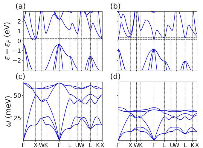
FIG. 3. Band structure of (a) Si and (b) GaAs. The Fermi level is located so that n_e = 10^{18} and 10^{15} \text{ cm}^{-3} for Si and GaAs, respectively. The energy window used to filter the \mathbf{k} points for transport computations is represented by horizontal dashed lines. Phonon dispersions of (c) Si and (d) GaAs.
