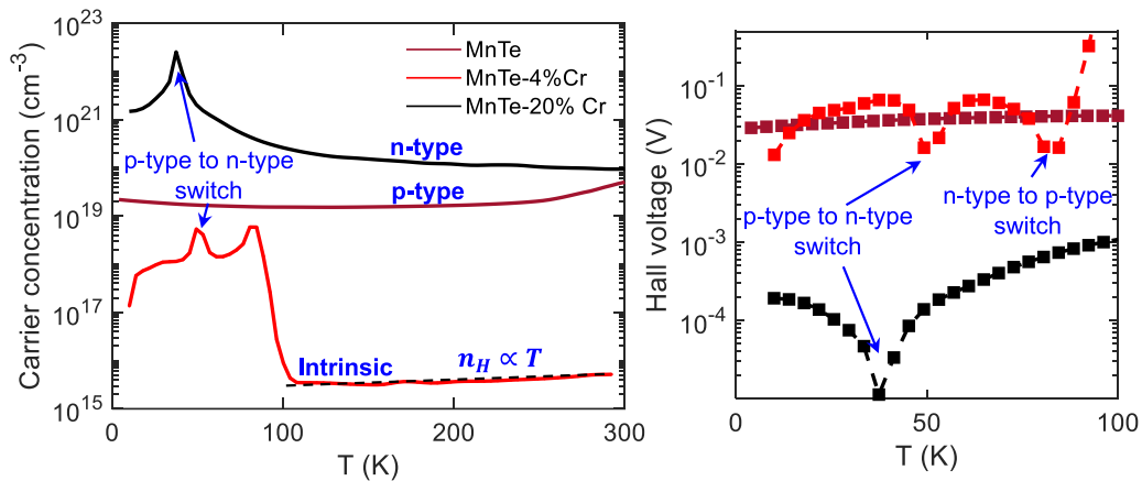
FIG. 6. (Left panel) Temperature-dependent carrier concentration of MnTe- x\% Cr samples ( x = 0, 4, and 20 ), (Right panel) the absolute value of the Hall voltage showing the switching of carrier type between the p - and n -type.
