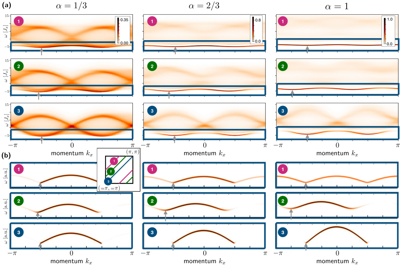
FIG. 7. One-hole spectral function in the dimensional crossover. (a) For varying anisotropy \alpha = t_y/t_x (indicated in top row) of the hopping elements, and \alpha^2 = J_y/J_x of the superexchange couplings, we use td-MPS to calculate the spectral function. We consider cylinders of length L_x = 40 along x , with circumference L_y = 4 along the periodic y direction; t_x/J_x = 3 is fixed. The MPS is wrapped around the cylinder along diagonals, which allows us to calculate diagonal cuts: k_y = k_x + k_y^{(0)} with k_y^{(0)} = \pi, \pi/2, 0 (cuts 1,2,3, see inset below left panel). (b) Predictions for the spinon contribution Z_s to the spectral weight (color map) and dispersion from fermionic mean-field theory of spinons, as described in the text. Mean-field parameters are taken from Ref. [83]. The delta-function peaks are represented by broadened lines with integrated weight equal to Z_s(\mathbf{k}) . In (a) and (b) the locations of dispersion minima in the low-energy region (blue boxes) are indicated by gray arrows.
