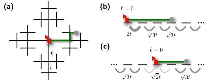
FIG. 14. Spinon-charge repulsion. (a) We consider a model where the charge fluctuations are described by string states, corresponding to the sites of a Bethe lattice. (b) Assuming a central-symmetric potential on the Bethe lattice, the one-particle hopping problem on the Bethe lattice, describing the fluctuating string, can be mapped to a semi-infinite one-dimensional chain with the indicated hopping amplitudes and a linear potential along the chain. (c) The problem in (b) can be related to an infinite one-dimensional problem with a mirror symmetry around the origin and reduced hopping matrix elements \sqrt{2}t to the central site, as compared to \sqrt{3}t elsewhere. As described in the text, this inhomogeneous tunneling gives rise to a strong (of order t ) microscopic spinon-charge repulsion.
