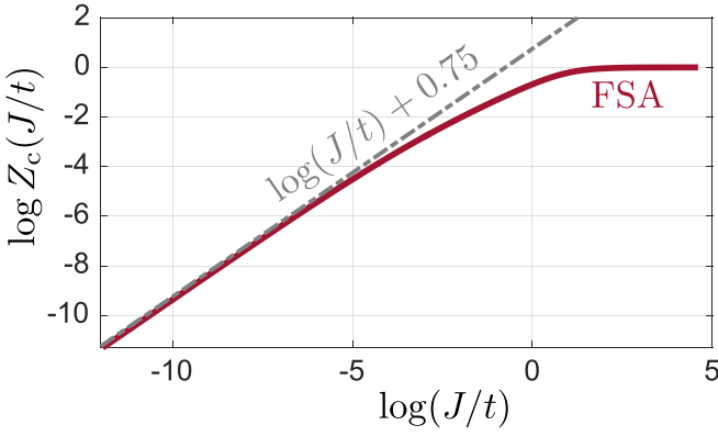
FIG. 15. Chargeon contribution to the quasiparticle weight. Z_c(J/t) is calculated from the model in Eq. (B3), based on the frozen spin approximation (FSA), and shown in a double-logarithmic plot. In the strong coupling regime J \ll t the asymptotic power law Z_c(J/t) \propto J/t is obtained as a result of spinon-chargeon repulsion.
