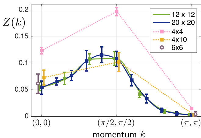
FIG. 16. Size dependence of the quasiparticle weight. Z(\mathbf{k}) is shown along the diagonal cut from (0,0) to (\pi, \pi) . We evaluated the spinon-chargon trial wave function for different system sizes (see legend). No significant finite-size dependence can be observed beyond 6 \times 6 . We set t/J = 3 , B_{\text{st}}/J_{\text{eff}} = 0.44 , and \Phi = 0.4\pi . Solid lines are guides to the eye only. Some data points are slightly offset horizontally for better visibility; for 6 \times 6 only a selection of \mathbf{k} points are shown.
