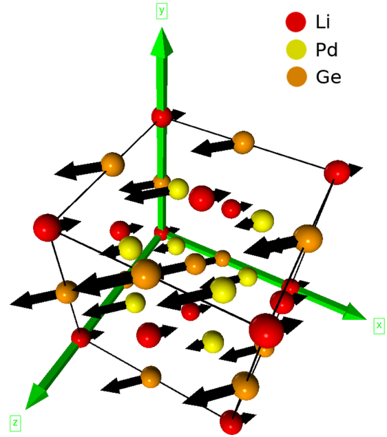
FIG. 11. Visualization of atomic vibrations with \mathbf{q} = (1/3, 1/3, 0) , for the first transverse acoustic mode of \text{LiPd}_2\text{Ge} . Red balls represent Li, orange balls in the middle of the edges and one in the middle of the cell represent Ge, and yellow balls inside the cube represent Pd. Pd and Ge vibrate in phase with each other and out of phase with Li.
