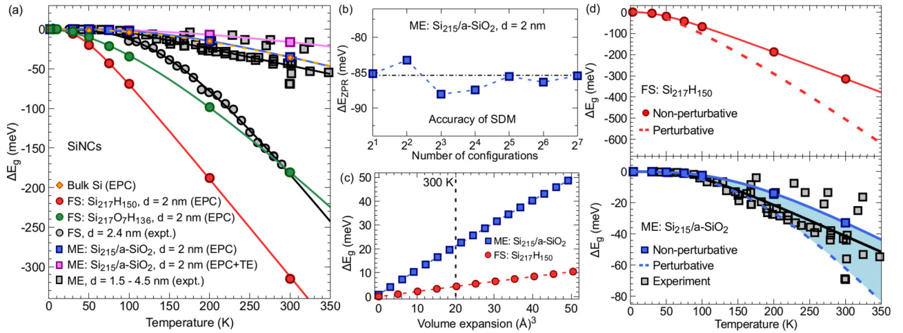
FIG. 3. (a) Temperature dependence of the band gap renormalization of freestanding (FS) and matrix-embedded (ME) SiNCs up to 350 K. Calculated band gaps using the ZG displacement [26] for H-terminated ( \text{Si}_{217}\text{H}_{150} ), oxidized ( \text{Si}_{217}\text{O}_7\text{H}_{136} ) and matrix-embedded ( \text{Si}_{215}/\text{a-SiO}_2 ) SiNCs are shown as red discs, green discs and blue squares, respectively. The diameter of the nanocrystals employed for our calculations is 2 nm. Magenta squares represent the band gaps of matrix-embedded SiNCs including also the effect of thermal expansion (TE). Orange diamonds represent data of bulk Si reported in Ref. [27]. Experimental data of oxidized freestanding SiNCs (black discs) is from Ref. [23] and of matrix-embedded SiNCs in a-SiO 2 (black squares) is from Refs. [20–22,73]. All curves represent fits to Eq. (11). (b) Variation of the zero-point renormalization of the matrix-embedded SiNC with the number of deterministic ZG configurations. The horizontal dashed line indicates the zero-point renormalization of 86 meV calculated using only one antithetic pair of ZG configurations. (c) Band gap renormalization versus volume expansion of H-terminated SiNCs (red discs) and matrix-embedded SiNCs in a-SiO 2 (blue squares). The vertical dashed line indicates the volume expansion at 300 K. (d) Comparison of temperature-dependent band gaps of the H-terminated SiNC (top panel) and matrix-embedded SiNCs in a-SiO 2 (bottom panel) calculated using the SDM (solid lines) and finite differences (dashed lines). The shaded area can be taken as the uncertainty of the band gap renormalization calculated for matrix-embedded SiNCs in a-SiO 2 . Experimental data of matrix-embedded SiNCs is as for (a).
