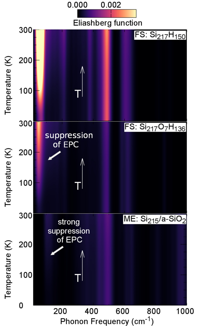
FIG. 5. Temperature dependence of the Eliashberg spectral function up to 300 K versus phonon frequency calculated for the freestanding fully H-terminated SiNC, the freestanding oxidized SiNC, and the matrix-embedded SiNC in a-SiO 2 from top to bottom, respectively. Thin arrows indicate the direction of increasing temperature and thick arrows highlight the suppression of electron-phonon coupling (EPC) after oxidation, and after placing the nanocrystal inside the matrix.
