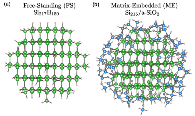
FIG. 1. Structures of (a) H-terminated freestanding (FS) and (b) matrix-embedded (ME) SiNCs with diameter d = 2 nm. Si atoms in the nanocrystals and passivating H atoms are shown in green and white. Matrix Si and O atoms are colored blue and gray, respectively.
