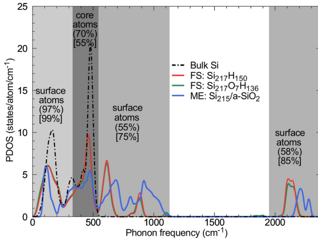
FIG. 4. Phonon density of states (PDOS) of the H-terminated freestanding SiNC (red), oxidized freestanding SiNC (green), matrix-embedded SiNC in a-SiO 2 (blue), and bulk Si (black). The shaded areas define the frequency range of the vibrational modes associated mainly with displacements of surface (light gray) and core atoms (dark gray). Percentages in round [square] brackets show the contribution to the vibrational modes associated with displacements of the indicated group of atoms in the freestanding [matrix-embedded] SiNC.
