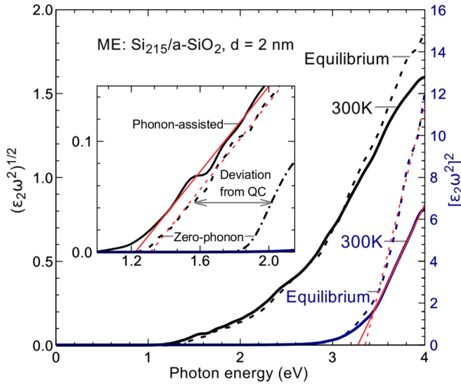
FIG. 7. Tauc plots [\epsilon_2\omega^2]^{1/2} (black spectra) and [\epsilon_2\omega^2]^2 (blue spectra) of the matrix-embedded SiNC, d = 2 nm, for indirect and direct transitions. The inset shows the Tauc plots close to the absorption onset. The dashed and solid lines represent spectra calculated with the nuclei at their relaxed equilibrium positions (zero-phonon) and for T = 300 K (phonon-assisted), respectively. The thin red lines represent the corresponding linear fits in the range of photon energies 1.3–2.0 eV and 3.4–4.0 eV for [\epsilon_2\omega^2]^{1/2} and [\epsilon_2\omega^2]^2 , respectively. The dashed-dotted line in the inset represents the zero-phonon spectrum of the freestanding SiNC, d = 2 nm, calculated with the nuclei at their relaxed QC positions. A Gaussian broadening of 50 meV was used for all spectra.
