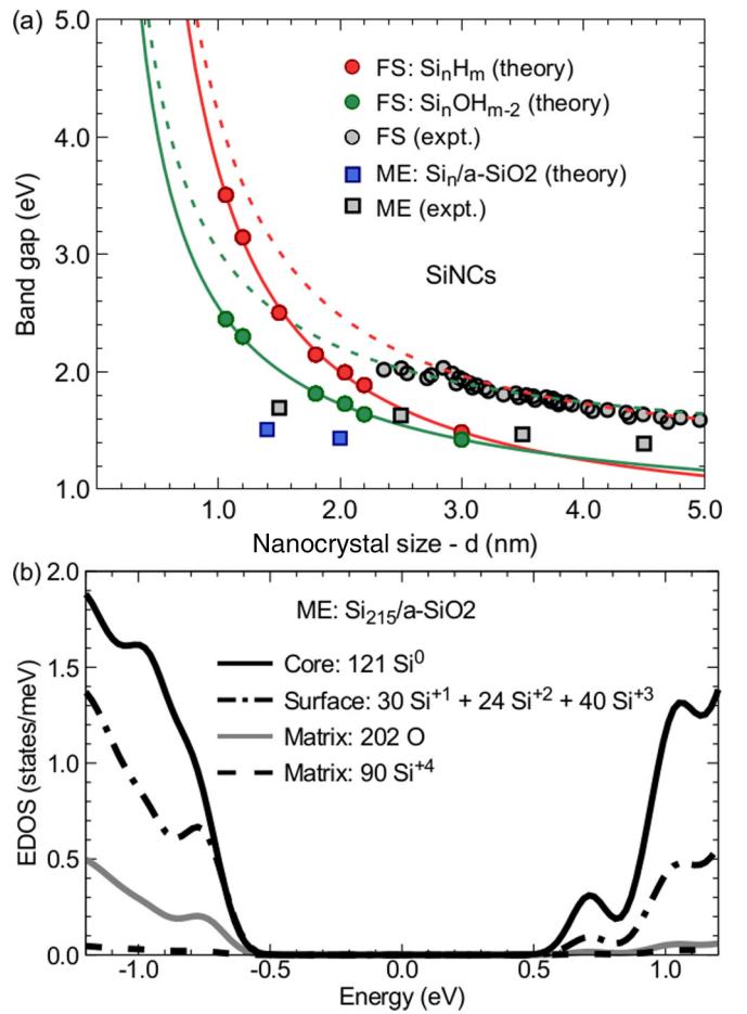
FIG. 2. (a) Band gap of silicon nanocrystals (SiNCs) as a function of average diameter d . Calculated band gaps of H-terminated ( \text{Si}_n\text{H}_m ), oxidized SiNCs ( \text{Si}_n\text{OH}_m ), and matrix-embedded ( \text{Si}_n/\text{a-SiO}_2 ) SiNCs are shown as red discs, green discs, and blue squares, respectively. The solid curves are fits of the form E_0 + a/d^b to the calculated band gaps of H-terminated SiNCs (red) and oxidized SiNCs (green) [67]. The dashed curves represent vertically shifted theoretical fits such that E_0 corresponds to the GW corrected band gap of bulk Si [70]. Experimental data of matrix-embedded SiNCs in a-SiO 2 (black squares) and freestanding SiNCs with oxidized surface (black discs) are from Refs. [22] and [65]. (b) Decomposition of the electronic density of states (EDOS) of the matrix-embedded SiNC into contributions from Si core atoms (black solid line), passivated surface Si atoms (black dashed dotted line), O matrix atoms (gray solid line), and Si matrix atoms (black dashed line). The Fermi level is set at the middle of the gap. A Gaussian broadening of 70 meV was used.
