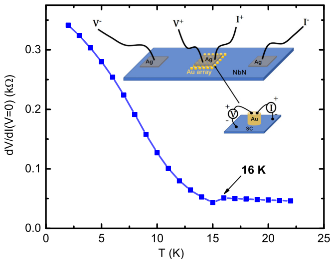
FIG. 3. The temperature dependence of differential resistance at zero-bias voltage. The inset shows a schematic structure of the measurement configuration for electrical transport in the nano-Au array/NbN structure and the circle shows point contact from one Au island.
