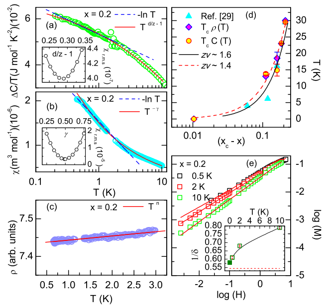
FIG. 7. (a) \Delta C/T and (b) \chi as a function of T (on a semilog scale). The solid red line represents the power-law fit. The dashed blue line represents a -\ln T behavior. (c) \rho(T) in the range 0.5–3 K, where the solid red line represents a linear fit. (d) Variation of T_C with x_C - x (on a semilog scale), where the solid and dashed lines represent fits. (e) M-H isotherms plotted as the \log M vs \log H , where the lines are the linear fits. Inset: 1/\delta as a function of temperature (closed symbols) and extrapolated to 0 K (open symbols). The red dotted line marks the value in the preasymptotic limit.
