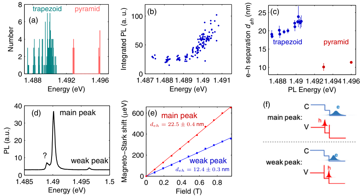
FIG. 8. (a) Distribution of the PL energy for excitons bound to the trapezoid and pyramid structures. 1.5 K. 810 nm excitation. (b) PL intensity as a function of E_{\text{SF}} . (c) Electron-hole separation as a function of the E_{\text{SF}} for trapezoid and pyramid structures. The electron-hole separation is measured by the magneto-Stark effect and the calculation uses in-plane exciton mass 0.17m_0 . (d) PL spectrum of a trapezoid with high PL energy. The peak marked by the question mark is unknown and does not exhibit magneto-Stark effect. (e) Magneto-Stark shift as a function of magnetic field for the main peak and second peak. The calculated e-h separation d_{eh} is listed in the figure. (f) Illustration of the exciton wave function for excitons of the two different peaks. C: conduction band. V: valence band. e: electron. h: hole.
