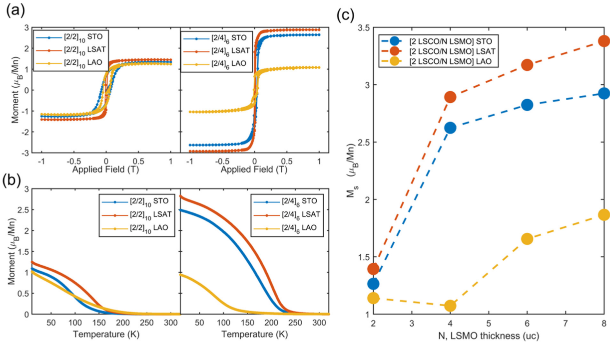
FIG. 3. Magnetic properties of [2\text{LSCO}/N\text{LSMO}]_x heterostructures as a function of strain and LSMO thickness. Magnetization for [2\text{LSCO}/2\text{LSMO}]_{10} and [2\text{LSCO}/4\text{LSMO}]_6 SLs grown on (001)-oriented STO, LSAT, and LAO as a function of (a) in-plane magnetic field at 10 K and (b) temperature. (c) Saturation magnetization, M_s , from magnetization versus applied magnetic field at 10 K as a function of LSMO thickness, N , and strain at 10 K for [2 - \text{uc LSCO}/N - \text{uc LSMO}]_x SLs.
