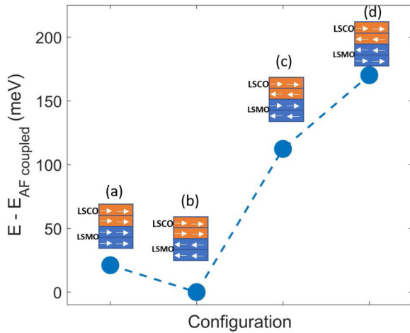
FIG. 7. Calculated energies for magnetic configurations theoretically investigated for [2 LSCO/2 LSMO] heterostructures compressively strained to \text{LaAlO}_3 . The minimum energy state, E_{AF^{\text{coupled}}} , corresponds to configuration (b) where the spins are aligned within each layer but are antialigned between the layers. The energies of the states are compared with the minimum energy state.
