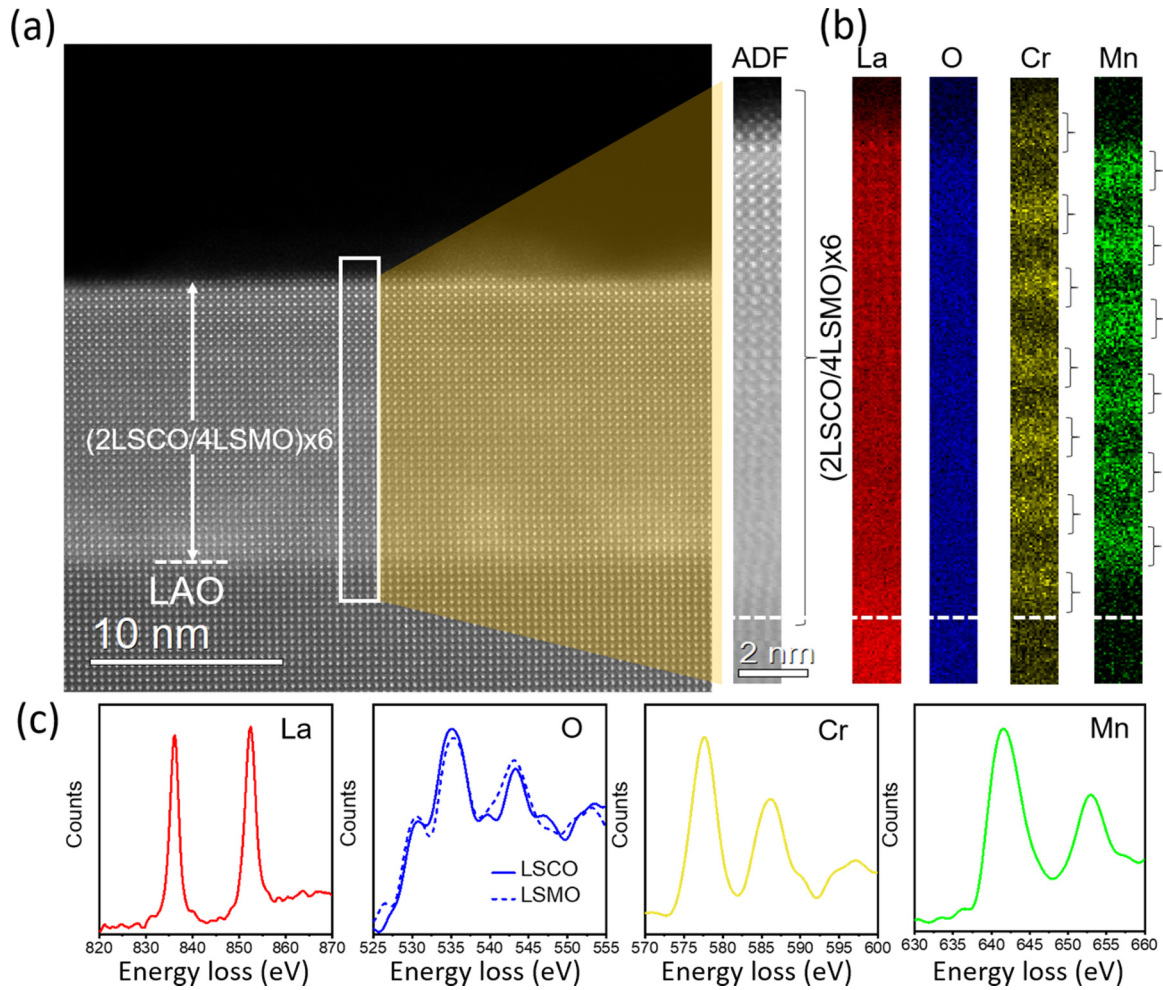
FIG. 2. High-resolution transmission electron microscope images of a [2\text{LSCO}/4\text{LSMO}]_6 grown on (001)- \text{LaAlO}_3 . (a) High-angle annular dark field image along the LAO (100) zone axis, (b) elemental maps obtained by electron energy loss spectroscopy measurements, and (c) representative EELS spectra for La, O, Cr, and Mn. EELS spectra are shown for O within the LSMO and LSCO sublayers.
