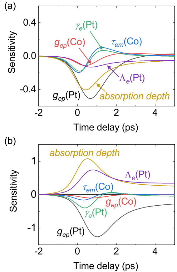
FIG. 3. Sensitivities of magnon temperatures to materials parameters in Pt(42)/Co(0.8)/Pt(4)/sapphire when pump is incident on (a) Pt(4) surface and (b) Pt(42) surface. \Lambda_e is electron thermal conductivity.
