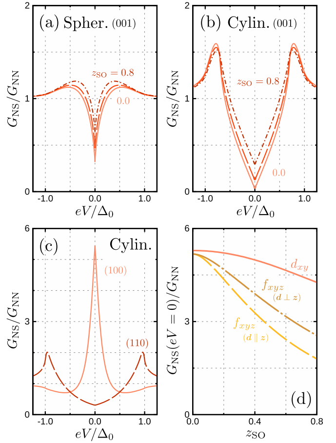
FIG. 9. (a),(b) Conductance of the nonchiral d -wave junction with c \parallel z . The width of the V shaped is characterized by \Delta_0 . (c) Conductance of the nonchiral d -wave junction with c \perp z . (d) z_{SO} dependences of G_{NS}|_{eV=0} for d_{xy} - and f_{xyz} -wave pairings. The zero-energy peak for the d_{xy} -wave junction is more robust against spin mixing than those for f wave. The barrier parameters are set to z_0 = 1 in (a), (b), (c), and (d). The spin-orbit interaction is set to z_{SO} = 0.0, 0.6 , and 0.8 in (a) and (b), and z_{SO} = 0.0 in (c).
