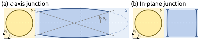
FIG. 2. Schematics of the Fermi surfaces. The FS of the SC is anisotropic due to the anisotropic effective mass. The cut-off angle \theta_c is introduced to make the FS in the SC cylindrical which is important when we estimate the effects of the Rashba spin-orbit coupling.
