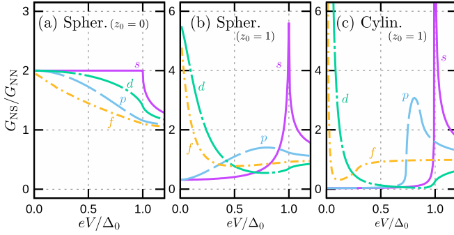
FIG. 3. Conductance of the NS junction along the c axis. The indices s , p , d , and f mean the SW, helical PW, chiral DW, and FW pairing, respectively. The Fermi surface is spherical in (a) and (b), and cylindrical in (c). The normalized effective masses in (c) are set to (\bar{m}_x, \bar{m}_y, \bar{m}_z) = (1.3, 1.3, 16.0) . The barrier potential is set to z_0 = 0 in (a) and z_0 = 1 in (b) and (c). The conductance is normalized to its value in the normal state G_{NN} . The result for chiral PW is identical to that for helical PW in the absence of spin-dependent potentials.
