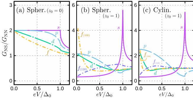
FIG. 8. Conductance of the NS junction with c \perp z . The results are plotted in the same manner as in Fig. 3. In the in-plane junction, G_{NS} for the FW SC depends on the direction of the interface; ZEP for (100) and V shaped for (110).
