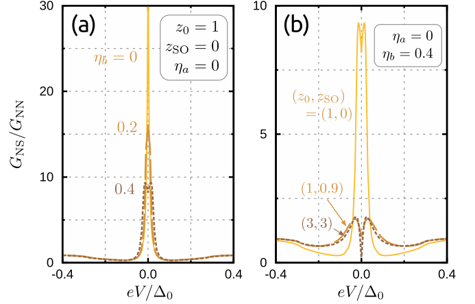
FIG. 7. Effects of the subdominant component e_c k_b on G_{NS} of the FW junction. A subdominant component is added to the FW pairing as given in Eq. (12). In the calculations, we set \eta_a = 0 and \eta_b \neq 0 reflecting the nematic superconducting state. The results for \eta_a \neq 0 and \eta_b = 0 are not qualitatively different from those shown in the figures above. The cylindrical FS is used. (a) The subdominant component splits the ZEP, where the parameters are set to z_0 = 1 and z_{SO} = 0 . (b) When both the subdominant component and the RSOI exist, G_{NS} can be even a narrow V-shaped one, where the parameters are set to (z_0, z_{SO}) = (1, 0), (1, 0.9), or (3, 3) .
