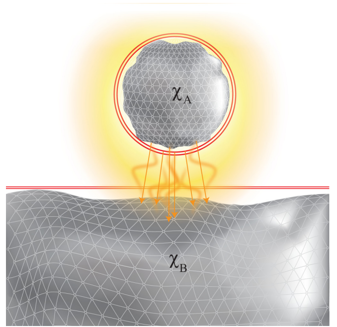
FIG. 1. Two bodies labeled A and B exchange heat in vacuum. Each body could be compact or of infinite extent in at least one spatial dimension, and for given susceptibilities \chi_p , the optimal structures may be quite complicated, but the upper bounds, which depend on \zeta_p = |\chi_p|^2/\text{Im}(\chi_p) , can be evaluated in simpler bounding domains that enclose each object while respecting any other design constraints present.
