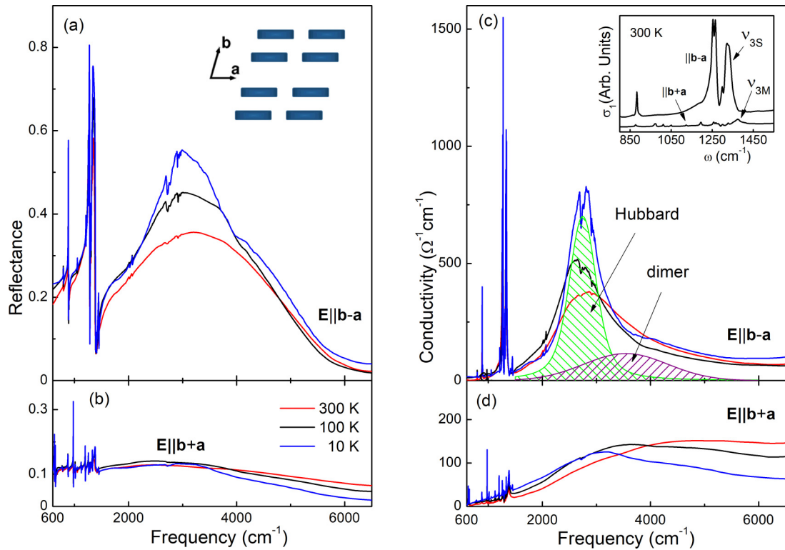
FIG. 3. Polarized reflectance and optical conductivity spectra of \beta' -(BEDT-TTF) _2 CF _3 CF _2 SO _3 for the \mathbf{E}||\mathbf{b}-\mathbf{a} (a, c) and \mathbf{E}||\mathbf{b}+\mathbf{a} (b, d) directions, at selected temperatures T = 300 K, 100 K, and 10 K. The insets in panels (a) and (c) display the simplified structure of the conducting layer and a close-up view of the 300-K optical conductivity in the vibrational range, respectively. Two components, Hubbard and dimer, of the electronic band at 10 K, are marked in panel (c).
