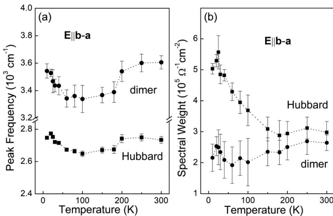
FIG. 4. Temperature-dependent peak frequency (a) and oscillator strength (b) of two components of the mid-infrared band observed in the conductivity spectra of \beta' -(BEDT-TTF) _2 CF _3 CF _2 SO _3 in the more conductive \mathbf{b}-\mathbf{a} direction, Hubbard band, and dimer band.
