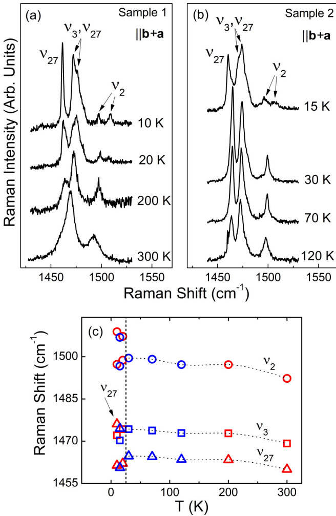
FIG. 5. Temperature dependence of the Raman spectra of \beta' -(BEDT-TTF) _2 CF _3 CF _2 SO _3 for sample 1 (a) and sample 2 (b). Polarization of the incident and detected light was parallel to the \mathbf{b}+\mathbf{a} direction; spectra are shifted for clarity. Panel (c) displays the Raman shift of the \nu_{27} ( \Delta ), \nu_2 ( \circ ), and \nu_3 ( \square ) mode components, as observed in the spectra of sample 1 (red color) and sample 2 (blue). The dashed line marks the approximate temperature point below which the splitting of the \nu_2 mode is observed. Lines between points are intended to guide the eye.
