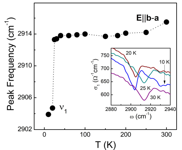
FIG. 7. The \nu_1 vibrational BEDT-TTF mode observed in the more conductive \mathbf{E}||\mathbf{b-a} direction observed in optical conductivity spectra of \beta' -(BEDT-TTF) _2 CF _3 CF _2 SO _3 . Inset: optical conductivity spectra at 10, 20, 25, and 30 K in this frequency range.
