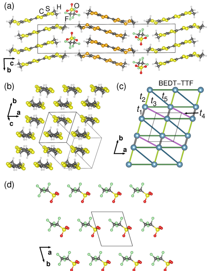
FIG. 1. Packing diagrams of \beta' -(BEDT-TTF) _2 CF _3 CF _2 SO _3 at 100 K. (a) BEDT-TTF molecules A and B are drawn with yellow and orange sulfur atoms, respectively. (b) BEDT-TTF layer of molecules A located at z = 0 . (c) Lattice of BEDT-TTF molecule centers for \beta' -(BEDT-TTF) _2 CF _3 CF _2 SO _3 with important hopping paths. (d) CF _3 CF _2 SO _3^- anions.
