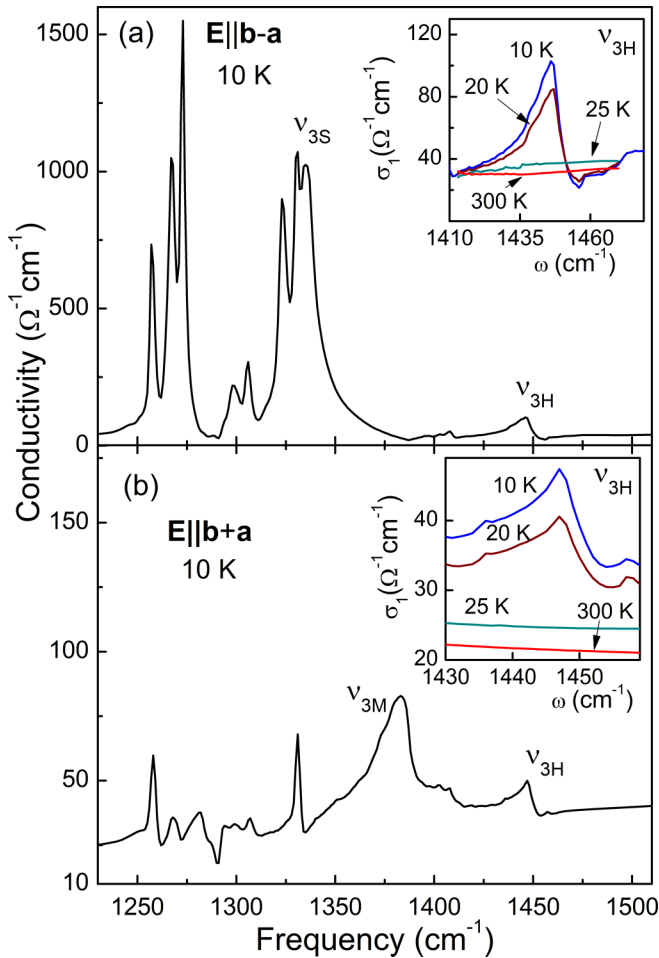
FIG. 6. Optical conductivity spectra of \beta' -(BEDT-TTF) _2 CF _3 CF _2 SO _3 at 10 K, in the frequency range of the electron-molecular vibration-activated \nu_3 mode for (a) the more conductive direction ( \mathbf{E}||\mathbf{b-a} ) and (b) perpendicular to the more conductive direction ( \mathbf{E}||\mathbf{b+a} ). Insets in panels (a) and (b) display a close-up view of the temperature dependence of the \nu_{3H} mode at 1446 \text{cm}^{-1} that appears in both spectra below 30 K.
