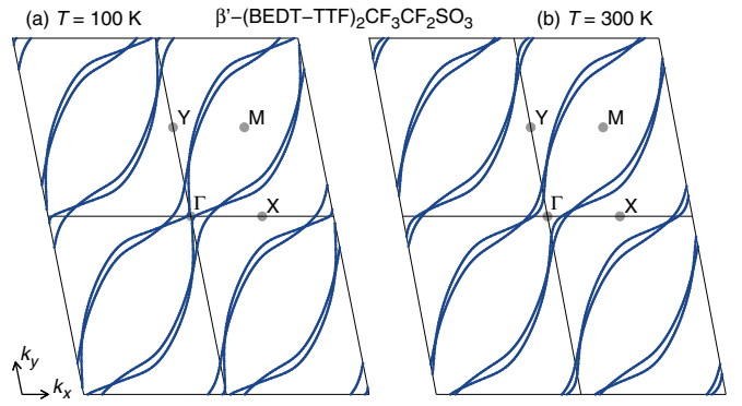
FIG. 2. Fermi surface of \beta' -(BEDT-TTF) 2 CF 3 CF 2 SO 3 at (a) T = 100 K and (b) T = 300 K.
