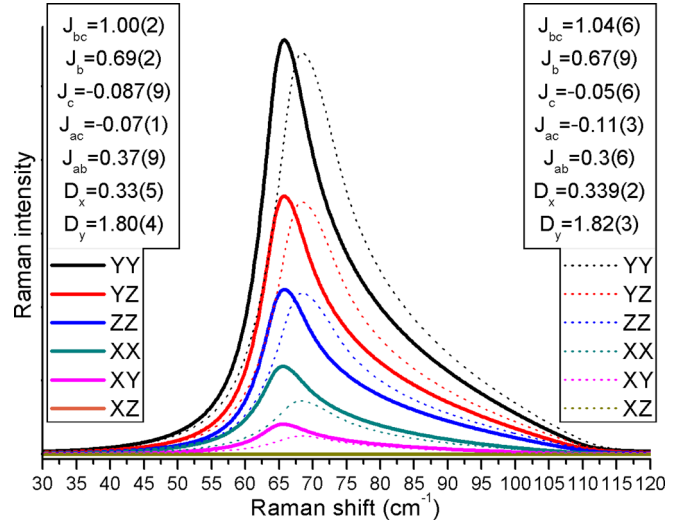
FIG. 5. Comparison between calculated two-magnon Raman spectra of \text{LiNiPO}_4 for different polarizations for the exchange and anisotropy parameters reported by Jensen et al. [9] and for the refined parameters obtained with the simulated annealing procedure explained in the text, in units of meV.
