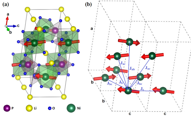
FIG. 1. (a) Orthorhombic unit cell of \text{LiNiPO}_4 (space group Pnma No. 62) with lattice parameters a = 10.02 \text{ \AA} , b = 5.83 \text{ \AA} , and c = 4.66 \text{ \AA} [6]. The magnetic structure is composed of \text{Ni}^{2+} magnetic moments oriented along the c axis with a small canting along the a axis [5]. (b) Detailed view of the magnetic structure and definition of the most important magnetic exchange paths between \text{Ni}^{2+} moments, namely J_b , J_c , J_{ab} , J_{ac} , and J_{bc} .
