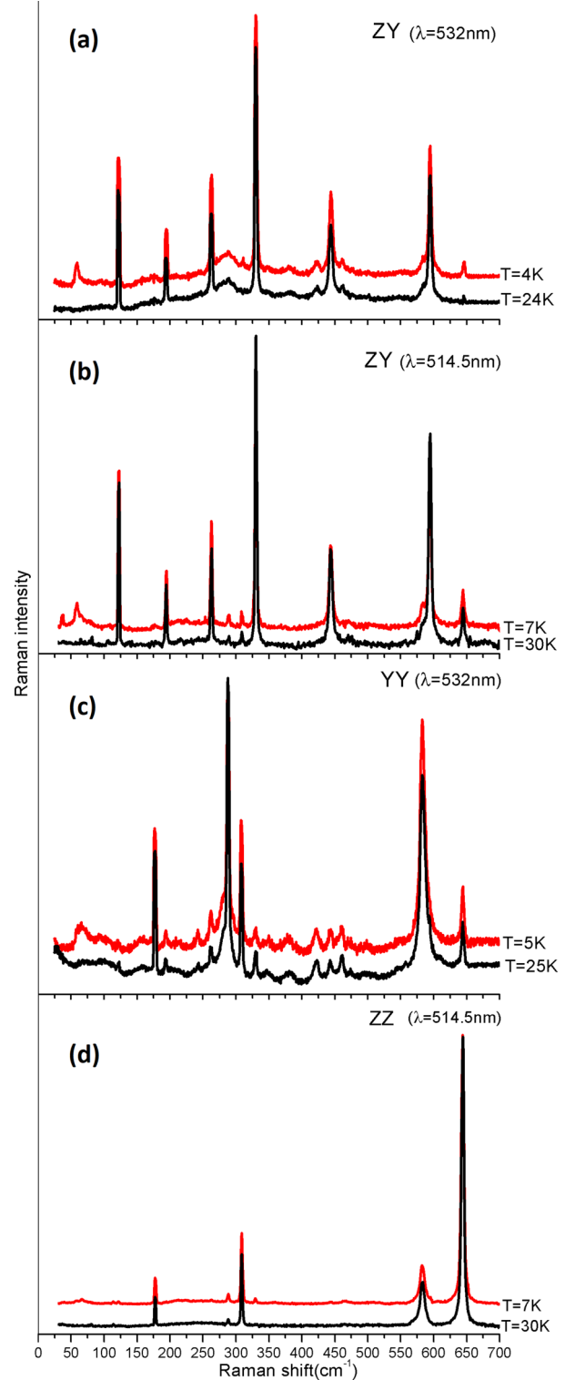
FIG. 2. Polarized Raman spectra below and above T_N = 20.8 \text{ K} with ZY polarization, \lambda = 532 \text{ nm} (a); ZY polarization, \lambda = 514.5 \text{ nm} (b); YY polarization, \lambda = 532 \text{ nm} (c); and ZZ polarization, \lambda = 514.5 \text{ nm} (d). The spectra were vertically translated for clarity.
