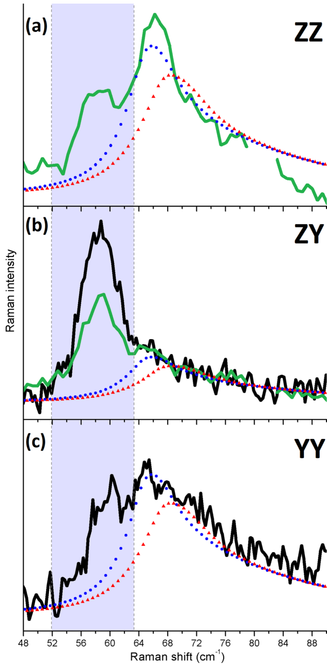
FIG. 4. Experimental Raman spectra in (a) ZZ polarization with \lambda = 514.5 nm (solid line), (b) ZY polarization with \lambda = 514.5 nm (green solid line) and \lambda = 532 nm (black solid line), and (c) YY polarization with \lambda = 532 nm (solid line), in a selected frequency range covering the two-magnon excitations at zero magnetic field and low temperatures, in comparison to calculated two-magnon profiles using an optimized set of exchange constants (blue circles, see text) and the set of constants given in Ref. [9] (red triangles). The marked spectral region between 52 and 63.5 \text{cm}^{-1} was excluded from the two-magnon fitting model due to the additional excitation observed at 58 \text{cm}^{-1} , not captured by our model.
