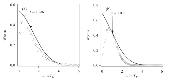
FIG. 11. The probability distribution of -\ln T_L at \nu = 0.0912 THz and that of -\ln T_T at \nu = 0.0552 THz. T_L and T_T are the total transmission rates of Fig. 10. The open circles are the numerical data for 10 000 samples, and the arrows indicate the averaged magnitude t of the numerical data. The solid lines are the theoretical probability distributions Eq. (28).
