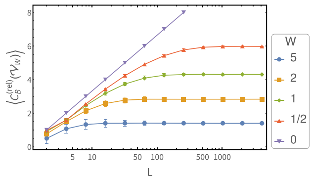
(b) relative entropy CGP (Anderson)
