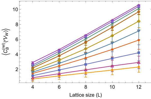
(b) relative entropy CGP (MBL)
