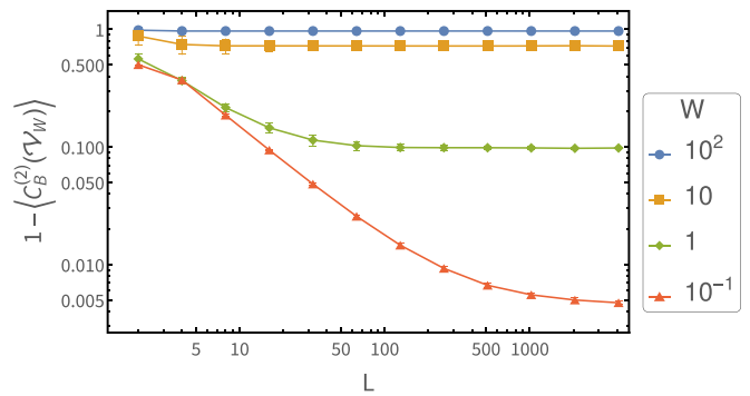
(a) average return probability (Anderson)
