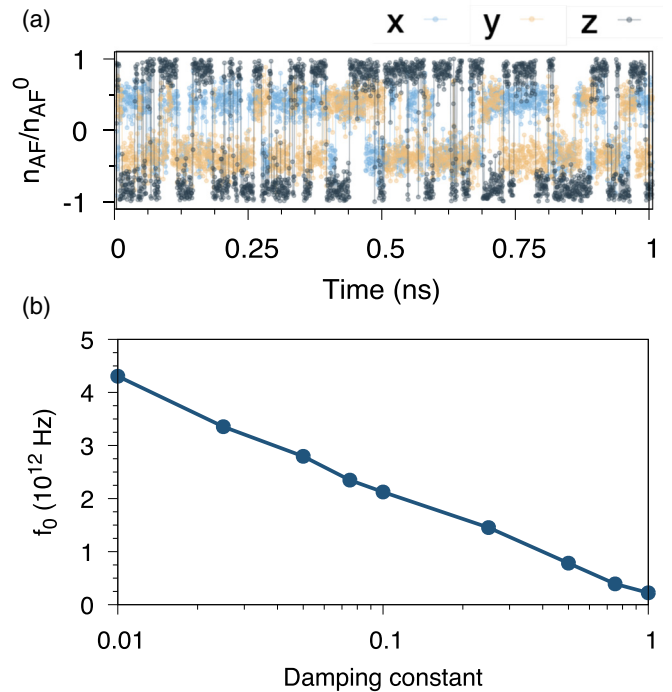
FIG. 4. Time-dependent magnetization of IrMn 3 at 100 K simulated using atomistic spin dynamics and dependence of the switching frequency on the damping constant. (a) The magnetization of IrMn 3 was simulated for 100 ns for a damping constant of 0.1, where only the first 1 ns is shown for clarity. The sublattice magnetization flips superparamagnetically between different coherent ground-state orientations. At this temperature, the sublattice ordering is approximately 90% since the system is simulated far from the Néel temperature. (b) Dependence of the attempt frequency for reasonable values of the damping constant from 0.01–1 shows a range for the attempt frequency between f_0 = 0.1 - 4 THz
