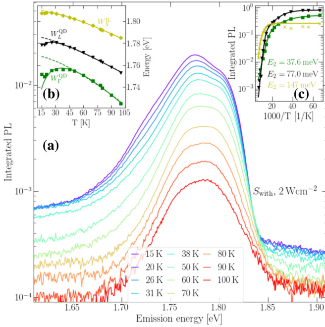
FIG. 14. S_{\text{with}} . (a) Measured PL at D = 2 \text{ W cm}^{-2} for temperatures between 15 and 100 K. In inset (b) we show the emission energy of W_{\Gamma}^{\text{QD}}-W_X^{\text{IL}} (symbols) as a function of temperature fitted by the Varshni Eq. (9), solid curve, [modified Varshni Eq. (11), dashed curve] model. In inset (c), integrated PL of individual transitions W_{\Gamma}^{\text{QD}}-W_X^{\text{IL}} (symbols) fitted (solid curves) by the Boltzmann model, Eq. (12) is shown along with the high temperature activation energies E_2 .
