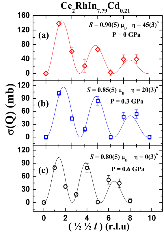
FIG. 4. l dependence (in reciprocal lattice units) of \sigma(Q) for the magnetic peaks (\frac{1}{2}, \frac{1}{2}, l) measured with the neutron energy of 35 meV at T = 2.0 K for (a) ambient pressure Ce 2 RhIn 7.79 Cd 0.21 (open diamonds) and with applied pressures of (b) 0.3 GPa (open squares) and (c) 0.6 GPa (open circles). The solid lines in each panel represent the best fit using the model discussed in Eqs. (1)–(3).
