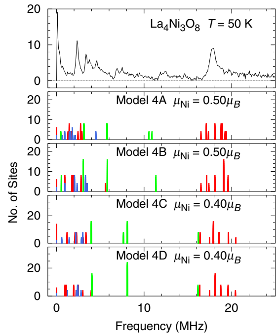
FIG. 23. Histograms of dipolar-field \mu^+ frequencies from AFM stripe models 4A–4D compared to 50-K \mu\text{SR} FT spectrum in \text{La}_4\text{Ni}_3\text{O}_8 . Colors as in Fig. 9.
