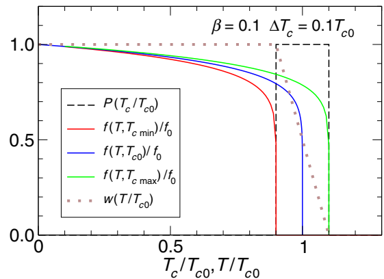
FIG. 24. Dashed curve: temperature dependence of transition temperature distribution P(T_c) , normalized by 2\Delta T_c for display. Solid curves: temperature dependencies of spontaneous NMR/NQR/ \mu\text{SR} frequencies f(T, T_c) for T_c^{\min} (red), T_{c0} (blue), and T_c^{\max} (green). Dotted curve: spectral weight w(T) .
