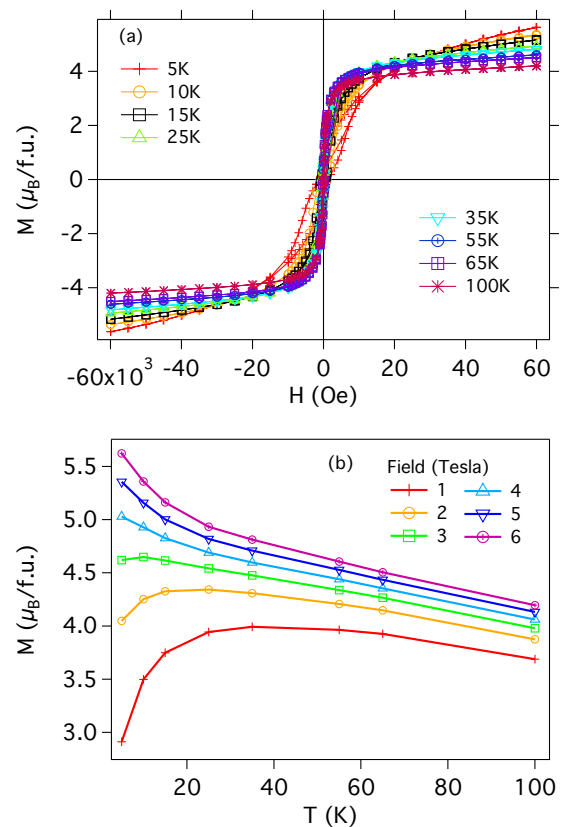
FIG. 4. (a) Magnetization vs field loop measured at different temperatures. (b) Magnetization vs temperature measured at different applied field.
