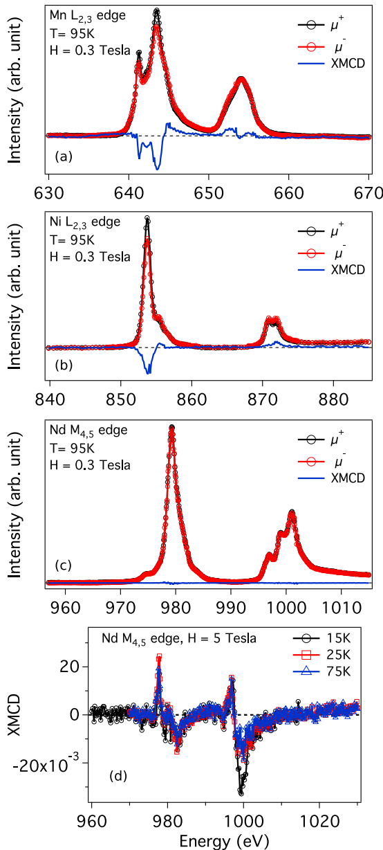
FIG. 5. X-ray magnetic circular dichroism (XMCD) data collected over (a) Mn L_{2,3} , (b) Ni L_{2,3} , and (c) Nd M_{4,5} edges at 95 K with an applied field of H = 0.3 T. (d) XMCD data collected over Nd M_{4,5} edge at 15, 25, and 75 K with an applied field of 5 T.
