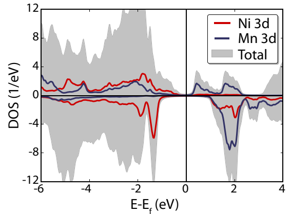
FIG. 6. Total density of states for majority and minority spin as well as the 3d-projected density of Ni and Mn atoms in \text{Nd}_2\text{NiMnO}_6 .
