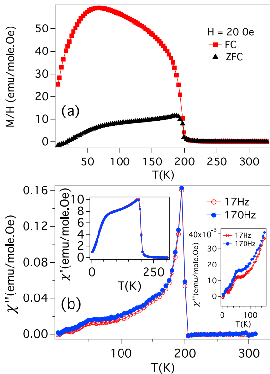
FIG. 3. (a) The field cooled (FC) and zero field cooled (ZFC) M/H , measured with an applied magnetic field ( H ) of 20 Oe. (b) The temperature variation of the imaginary part of the ac susceptibility at 17 Hz and 170 Hz with an amplitude of the ac field of 4.0 Oe. The two insets show the temperature variation of the real part of the ac susceptibility and an enlarged plot of the imaginary part of the ac susceptibility below 100 K in separate panels.
