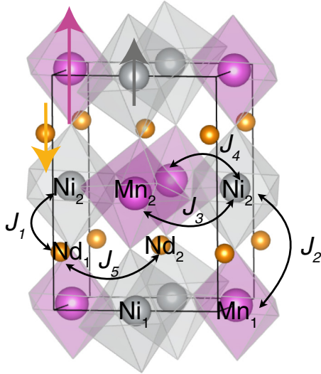
FIG. 7. The crystal structure of \text{Nd}_2\text{NiMnO}_6 . The labels indicate the exchange couplings between, as an example, \text{Ni}_2 and the other atoms in the system. The exchange parameters between atom Ni, Mn, and Nd with the neighboring atoms in meV are as following: J_1 = 0.03 (0.23) between Ni (Mn) and Nd, J_2 = 5.99 , J_3 = 4.90 , J_4 = 19.05 , and J_5 \leq 0.01 (due to the distortion in the system and smallness of J_1 and J_5 , the averaged values are given). For the further neighbors the exchange parameters quickly decay to almost zero. For more detail, see Table I. The orientations of magnetic moments, including the spin and orbital contributions, at different sites in the ground state are shown on three types atoms in the top left corner of the unit cell. For the Nd site, the spin moment is oriented in a direction opposite to that of the total moment or in other words, in a parallel orientation with the spin moments of Ni and Mn shown here.
