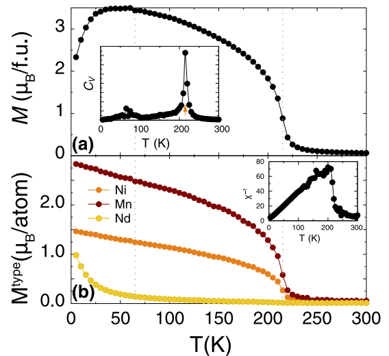
FIG. 8. (a) The total magnetization of \text{Nd}_2\text{NiMnO}_6 calculated as a function of temperature T . The inset shows the calculated specific heat as a function of temperature. The red arrow indicates the peak in C_V related to ferromagnetic phase transitions. (b) Element-specific magnetization calculated as a function of the temperature, where different elements are indicated by different colours. The inset shows the inverse susceptibility of Nd moments in presence of the internal field arising from ordered Ni+Mn moments (see text for more details) as a function of the temperature, suggesting a very close adherence to the Curie-like behavior.
