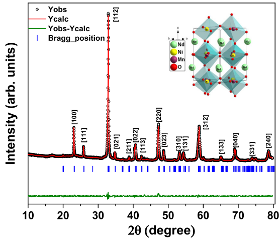
FIG. 1. Observed (open circle), calculated (red line), and residual (green line) XRD pattern. Vertical lines are the Bragg peak positions.
