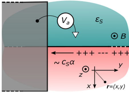
FIG. 1. Top view of the edge of a two-dimensional material (red half-plane) in the quantum Hall regime surrounded by an insulator (green region) with dielectric constant \epsilon_S . The QH material supports edge excitations that are driven by an external potential V_a applied to a capacitively coupled ideal electrode (gray area). The edge magnetoplasmon propagates chirally at the boundary of the QH material with a velocity \sim c_S \alpha , where c_S is the speed of light in the medium and \alpha \approx 1/137 is the fine structure constant.
