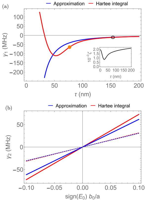
FIG. 10. Coupling constants \gamma_{1,2} . For the plots, we use 2a = 30 nm, \Omega = 3.85 meV, B = 0.44 T, and L_y = 27.7 \mu\text{m} ; we consider l' = 0.75l_B and x_0 = 1.15l_B , as discussed in Sec. II B. We also include the effect of a top gate placed at distance d = 0.6 \mu\text{m} from the EMP. In (a), we consider E_0 = 0 . The blue line is obtained using Eq. (86), and the red line is obtained using Eq. (93). In the inset, we plot the dimensionless parameter \zeta , defined in Eq. (C18), which quantifies the coupling between the computational and the noncomputational subspace of the double dot. In (b), we show the dependence of the coupling \gamma_2 on a homogeneous electric field E_0 . The length b_0 is defined in Eq. (91) and it is proportional to |E_0| ; to include negative values of E_0 , we rescale the horizontal axis by \text{sign}(E_0) . The blue and red lines are obtained respectively by using Eqs. (89) and (94). The solid and dashed lines are obtained by using \tau = \tau_s = x_0 + a + l_T \approx 77 nm, and \tau = 2\tau_s \approx 154 nm. These values of \tau are marked in (a) by using an orange dot and a black circle, respectively.
