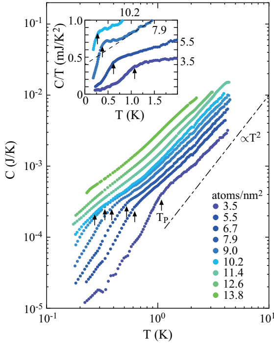
FIG. 2. Heat capacity of ^4\text{He} as a function of temperature for various areal densities below 14 \text{ atoms/nm}^2 . The arrows indicate T_p , and the dot-dashed line is proportional to T^2 . The areal densities are presented in units of \text{atoms/nm}^2 . Inset: C/T as a function of T below 10.2 \text{ atoms/nm}^2 . The dashed line displays an extrapolation from the high-temperature side of the peak.
