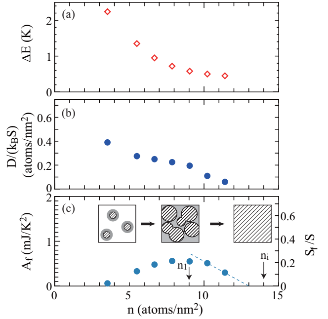
FIG. 5. Fitting results for (a) \Delta E , (b) D/(k_B S) , and (c) A_f as a function of areal density. In (c), the dashed line shows the extrapolation of the decrease above 10 atoms/nm 2 . The right vertical axis of (c) is S_f/S . The inset plots in (c) show schematic top views of the film at approximately 3.5 atoms/nm 2 , n_1 , and n_i , from left to right (at T \gg T_p for the former two areal densities). The hatched and gray areas correspond to solid and fluid areas, respectively.
