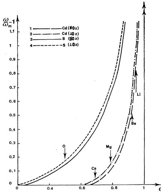
FIG. 3. Variation of a localized-mode frequency as a function of \epsilon_\kappa = (M_\kappa - M')/M_\kappa .
